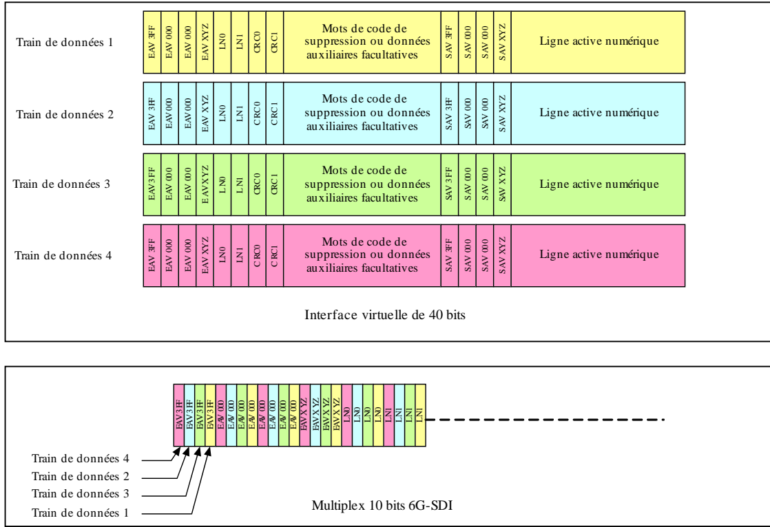
FIGURE 3-10 Multiplex 10 bits 6G-SDI – Type 1
