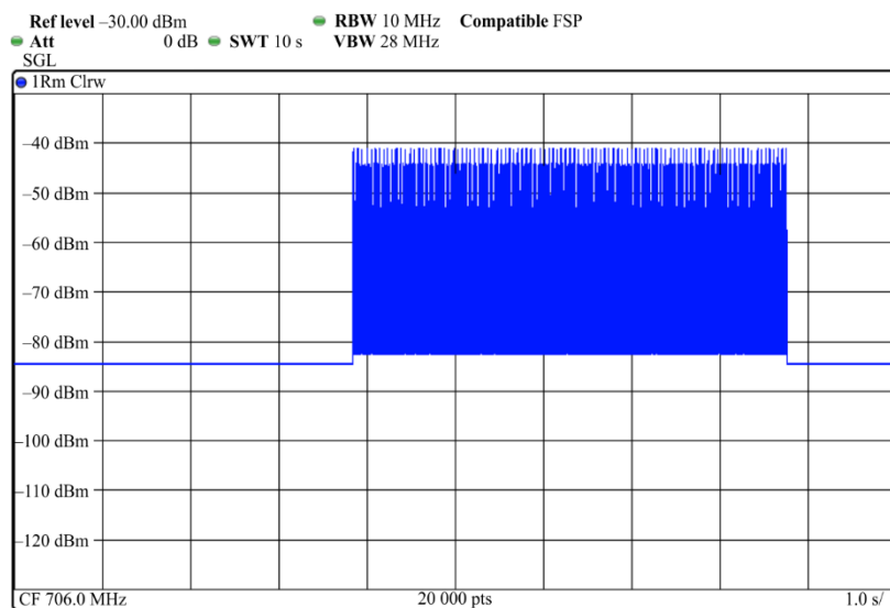
FIGURE 2 Gated LTE 1 Mbit/s signal
