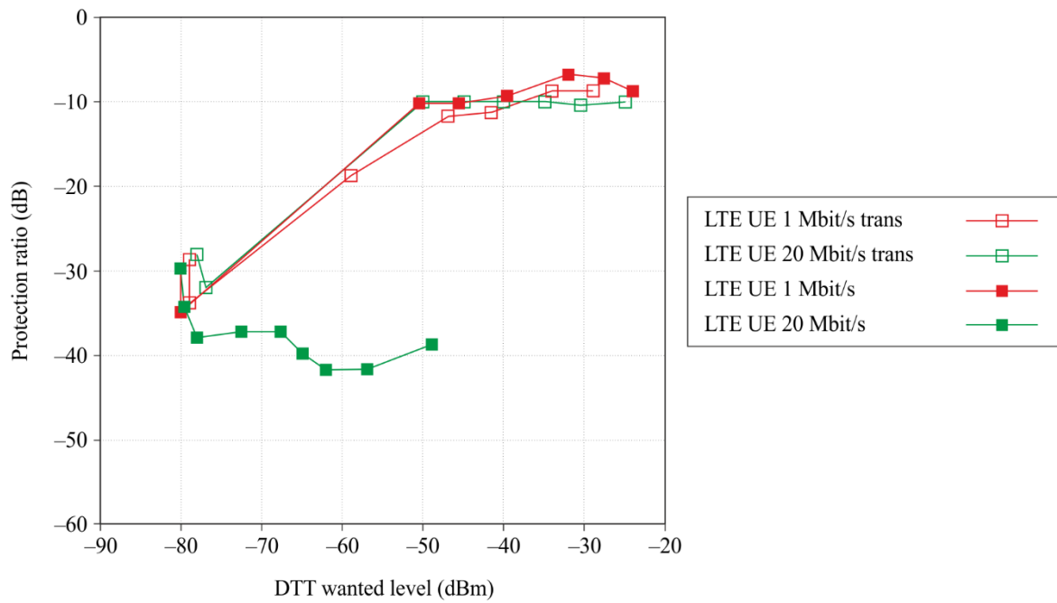
FIGURE 3 Receiver R1 11 MHz offset
