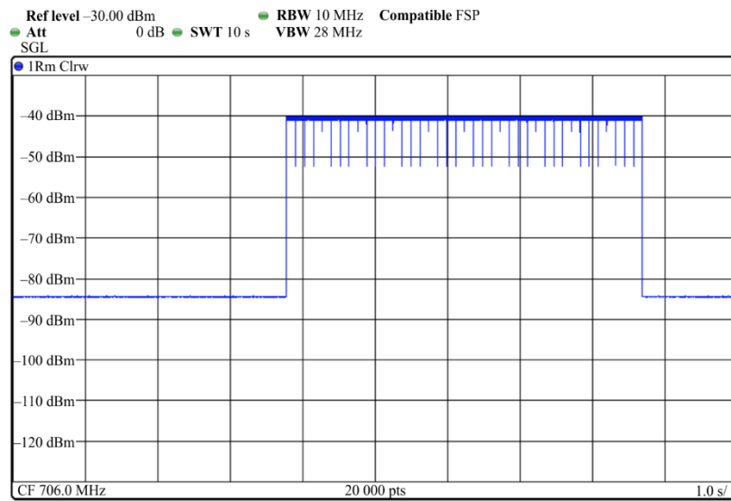
FIGURE 1 Gated LTE 20 Mbit/s signal
