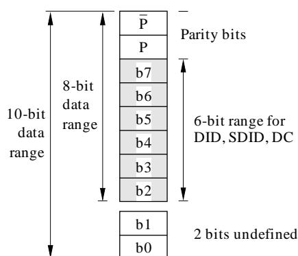
FIGURE 1-2 Coding range for 8-bit DID, SDID, DC
