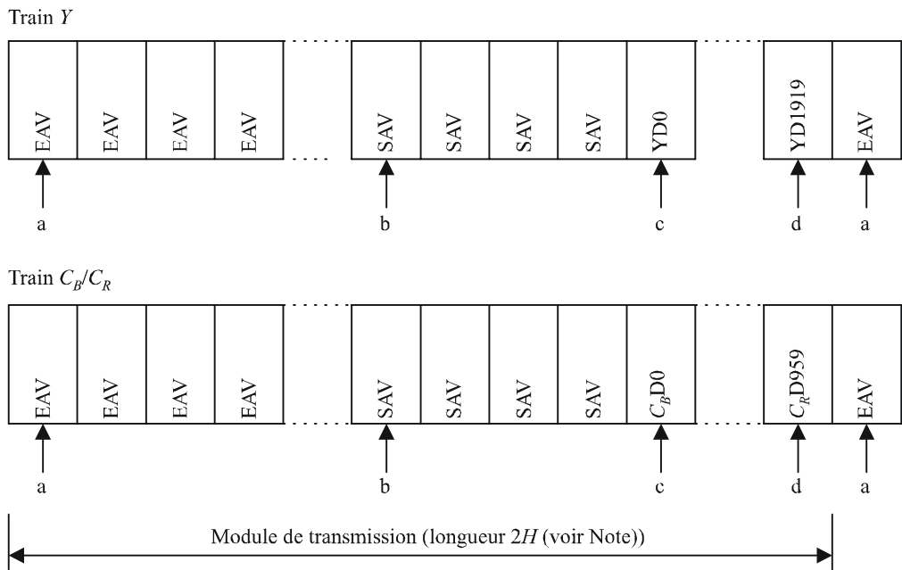
FIGURE 15 Train binaire horizontal multiplexé
