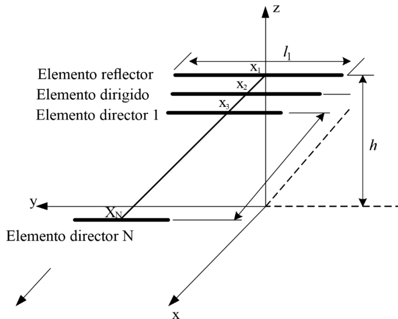
FIGURA 45 Antena general Yagi-Uda
