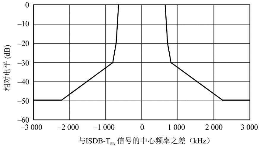
图3 适合于ISDB-T SB 传输信号的频谱掩膜 (BW = 6/14 MHz, n = 3)
