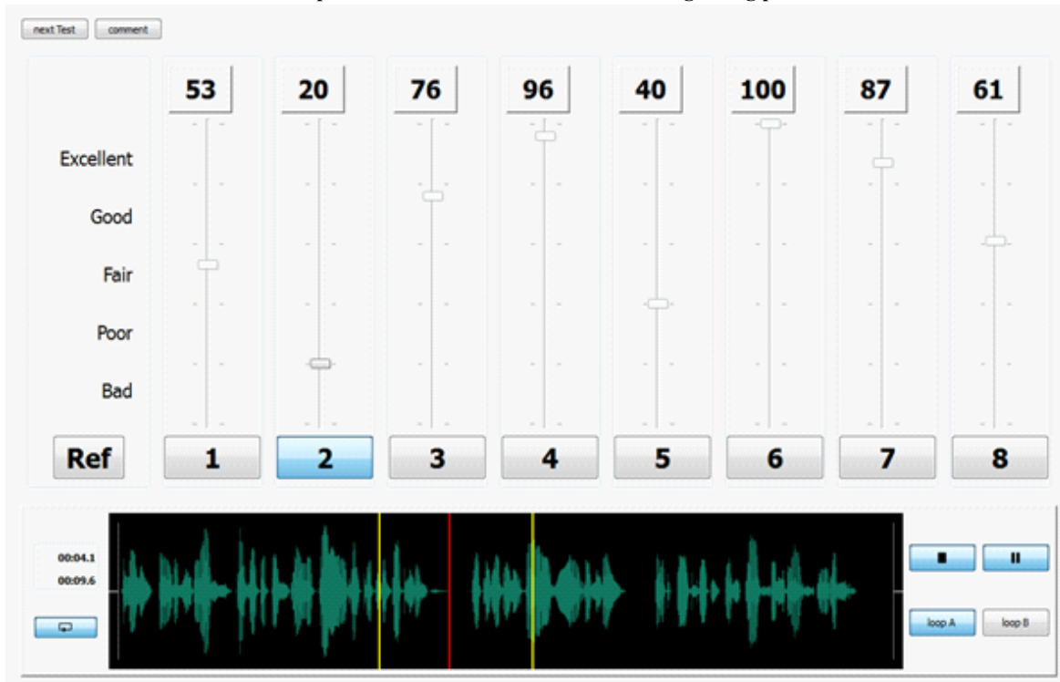
Example of a user interface used in the blind grading phase
