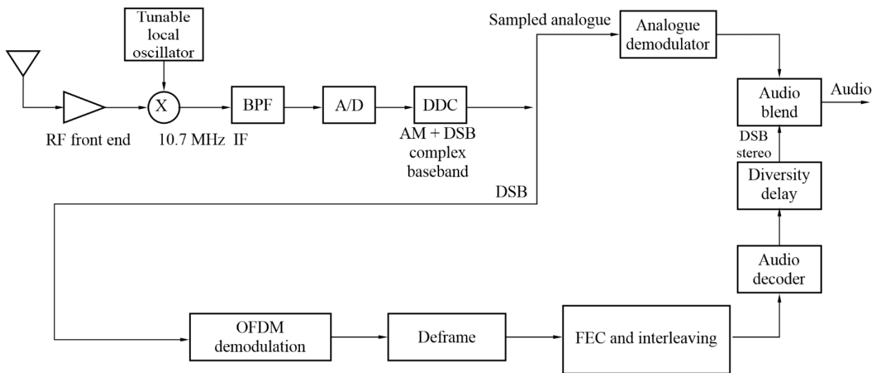
FIGURE 5 Hybrid MF IBOC typical receiver block diagram
