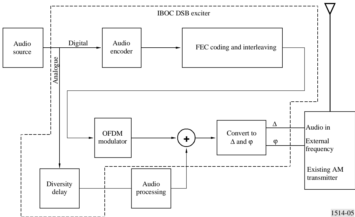
FIGURE 5 Hybrid MF IBOC DSB transmitter block diagram
