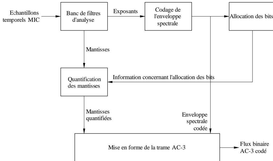
FIGURE 7 Codeur AC-3
