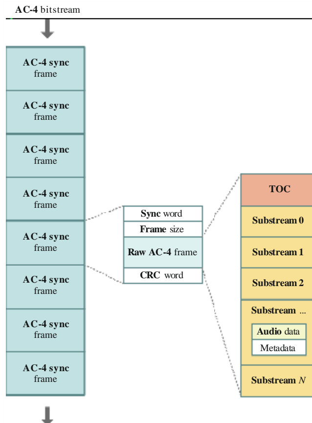
FIGURE 14 High-Level Bitstream Syntax
