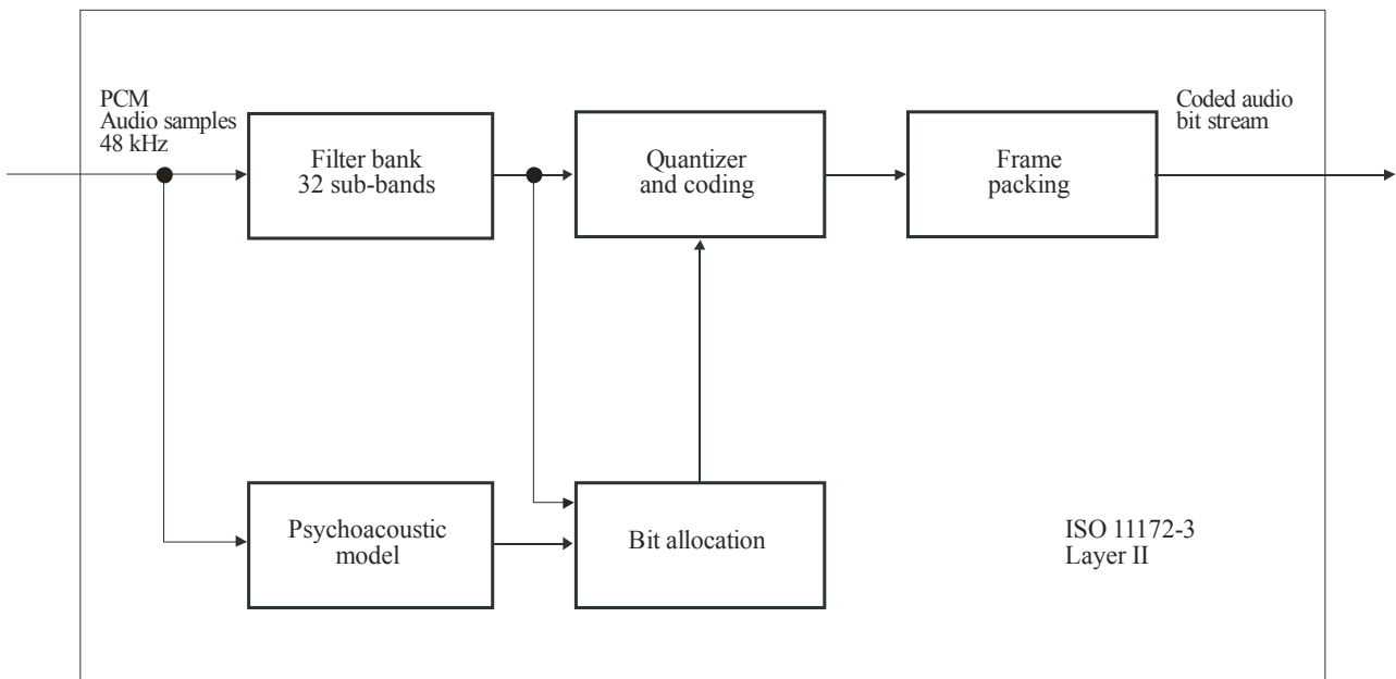
Block diagram of the basic system audio encoder
