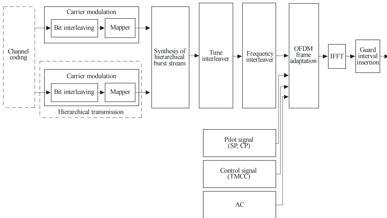
Modulation block diagram
