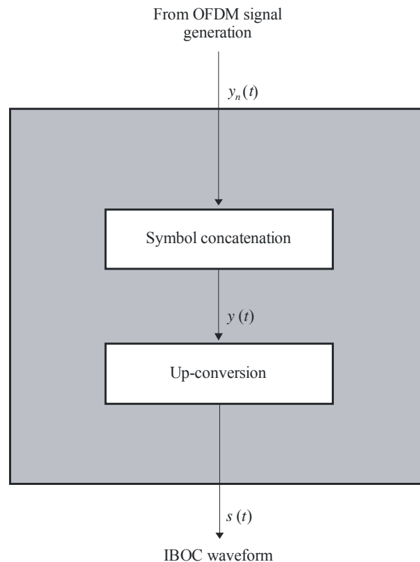
FIGURE 31 All digital transmission subsystem functional block diagram
