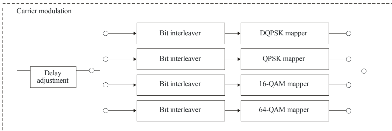
Configuration of carrier modulation block
