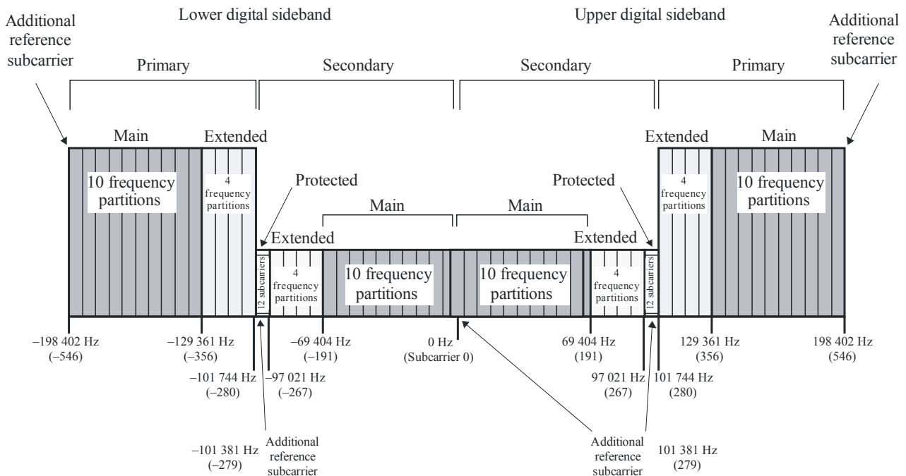
FIGURE 34 Spectrum of the all digital waveform – Service modes MP5 through MP7, MS1 through MS4 (The level of the digital subcarriers is such that the total power of these carriers is no more than 10 dB below the nominal power of the FM analogue carrier that it replaces)
