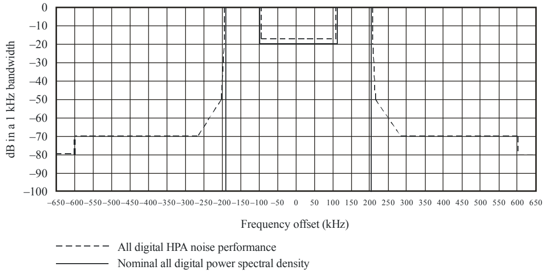
FIGURE 36 All-digital emission limits*
