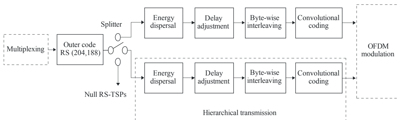
FIGURE 17 Channel coding diagram
