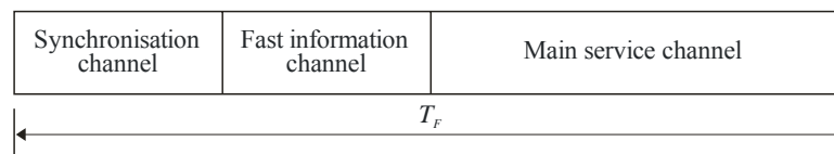
FIGURE 4 Multiplex frame structure
