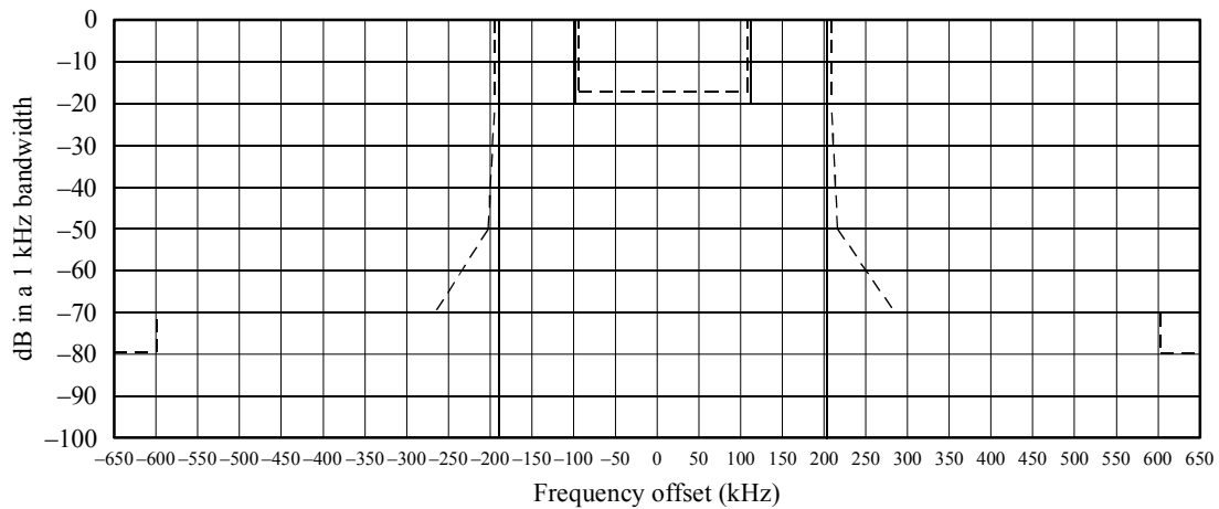
FIGURE 36 All-digital emission limits*
