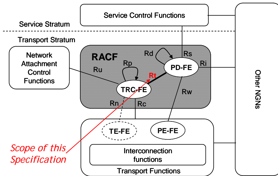
Figure 1: Localization of the Rt reference point in the Generic Resource and Admission Control Functional architecture of NGN
