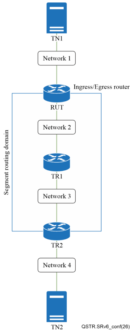
Figure 2 – Common test topology-B
