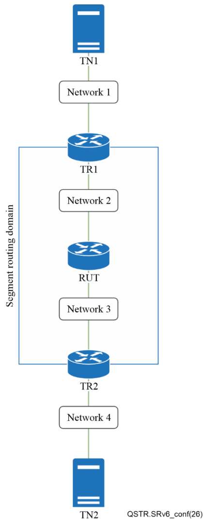
Figure 1 – Common test topology-A
