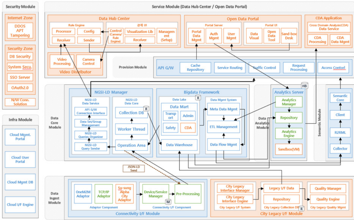
Figure 18: Data hub architecture
