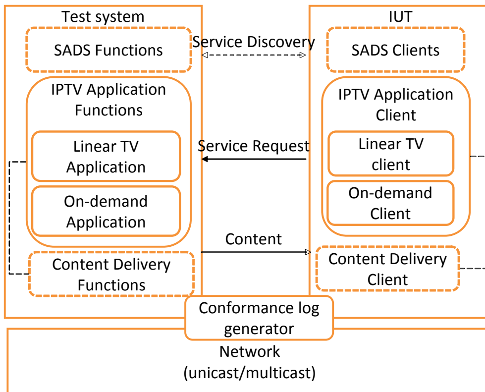
Figure 5-1: Test bed for basic IPTV services
