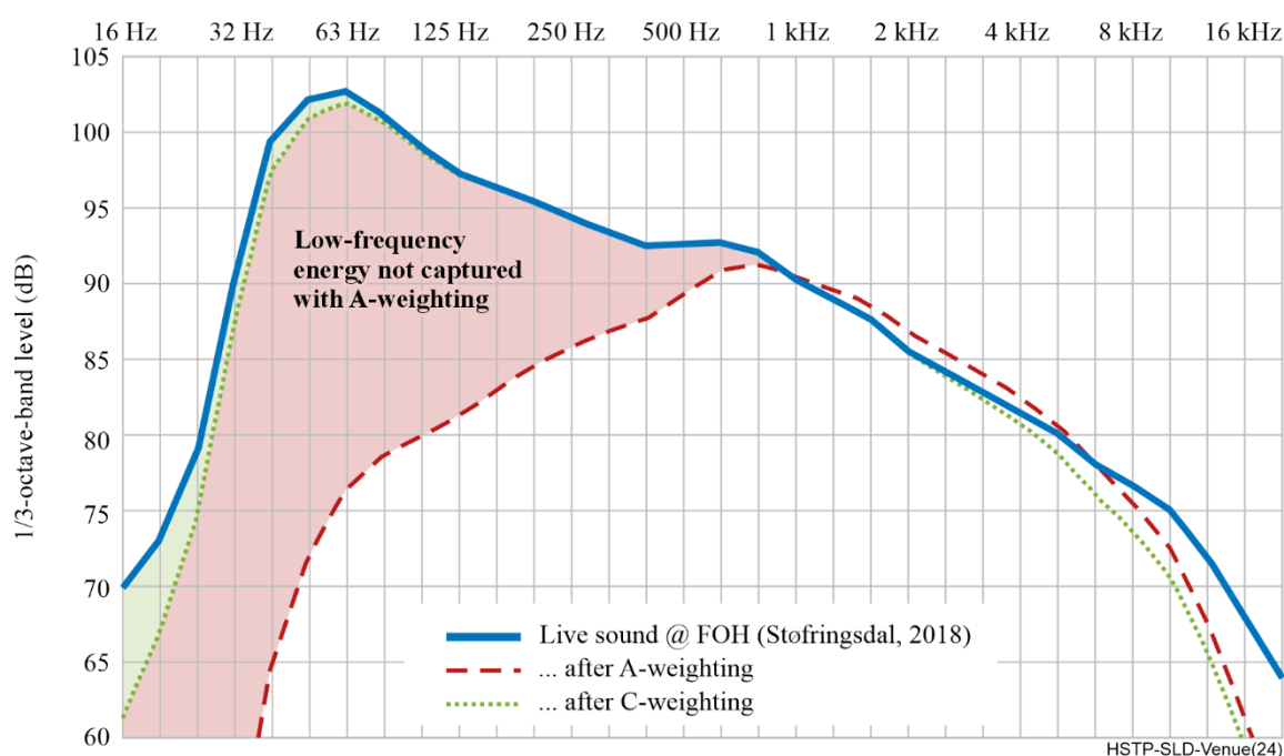
Figure III.1 – Discrepancy in low-frequency contribution with sound measurements
