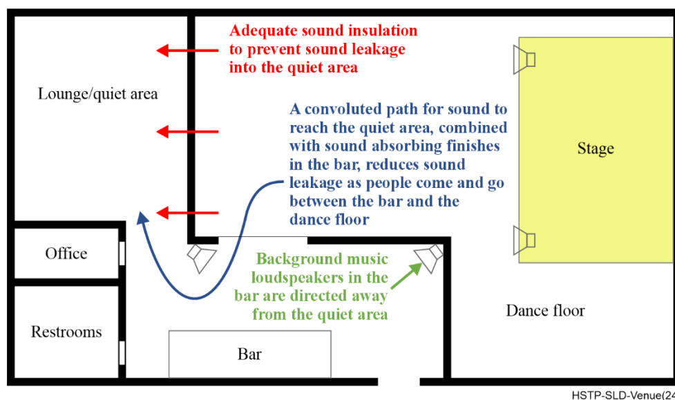
Figure 7 – Example of a venue plan including a quiet zone suitable for meeting the Swiss requirements
