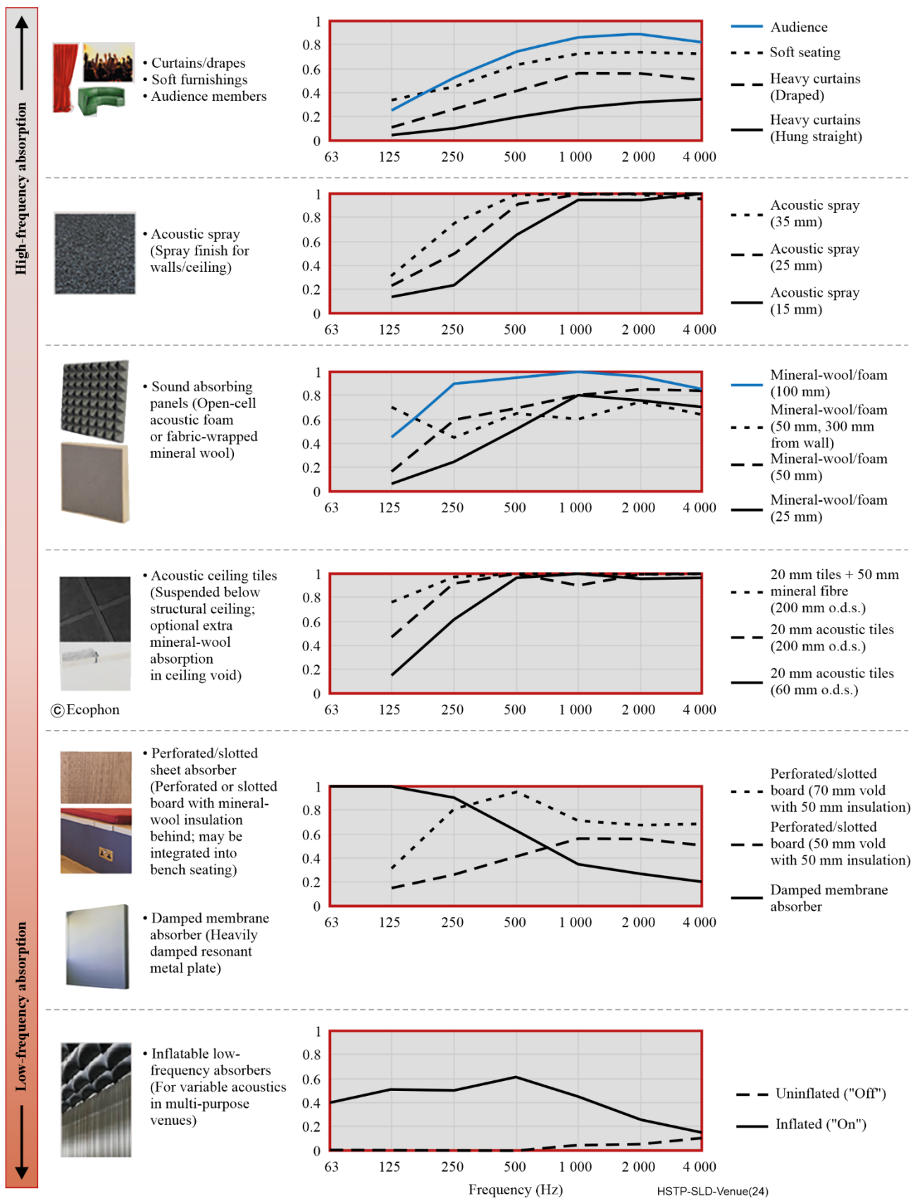
Figure VII.3 – Absorption properties of different objects
