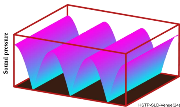
Figure VIII.1 – Example illustration of a room mode
