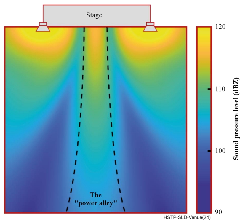
Figure VIII.2 – Visual representation of the power alley effect
