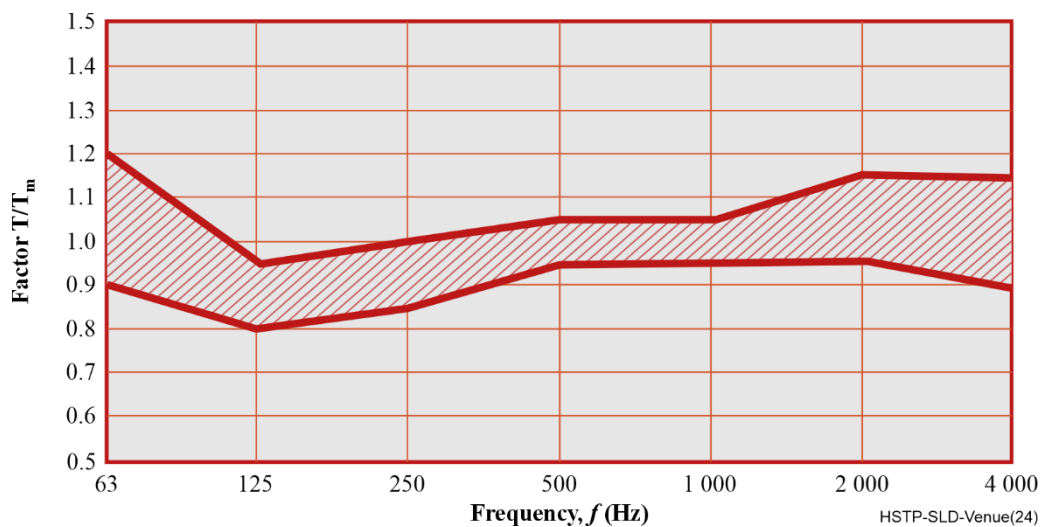
Figure VII.2 – Recommended tolerances for reverberation time* at different octave bands for venues for amplified music
