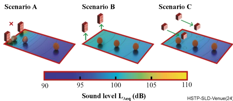
Figure IX.1 – Positioning of loudspeakers and their effect on sound distribution
