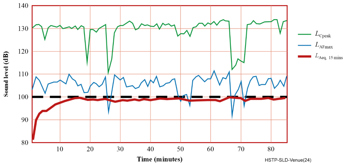
Figure III.2 – Different types of sound-level measurements throughout a performance
