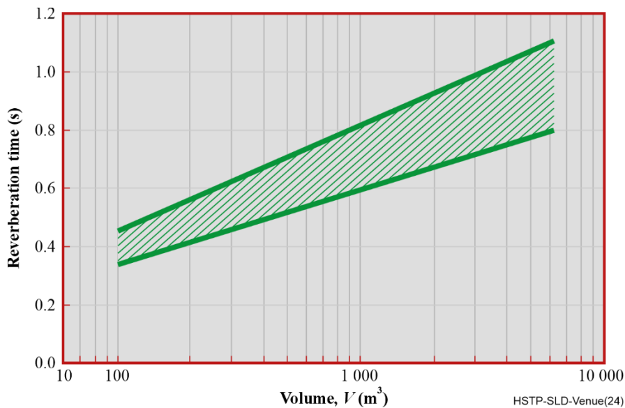
Figure VII.1 – Recommended mid-frequency reverberation times* for venues for amplified music, as a function of room volume
