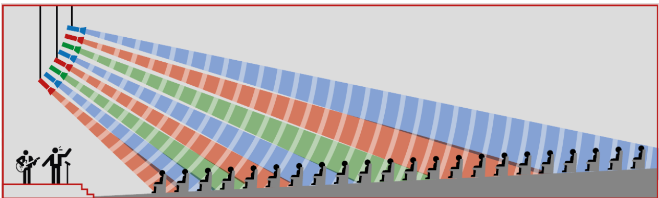
Figure IX.2 – Visual representation of sound distribution with a line array loudspeaker configuration
