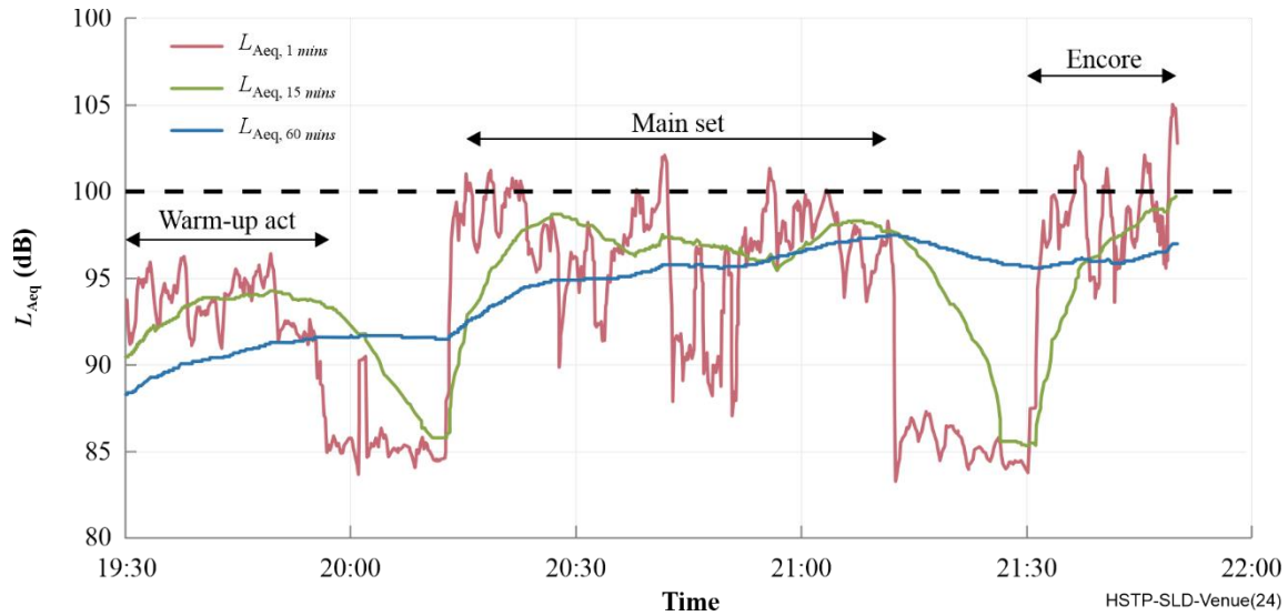
Figure II.1 – Evolution of time-averaged, A-weighted sound level: example for a live-music event
