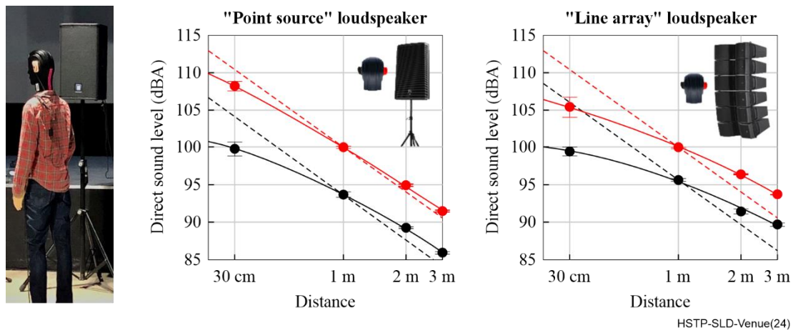
Figure X.1 – Direct sound levels and proximity to point source and line array loudspeakers
