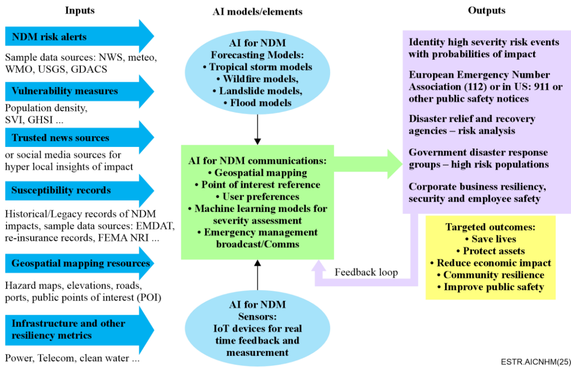
Figure 9 – Suggested inputs, outputs, AI models and targeted outcomes when using AI in dashboards
