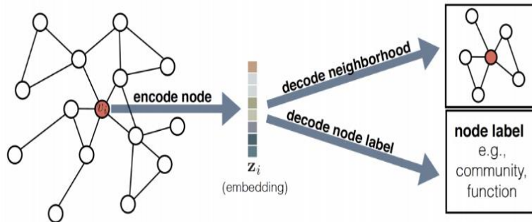
Figure 63 – Node embedding
