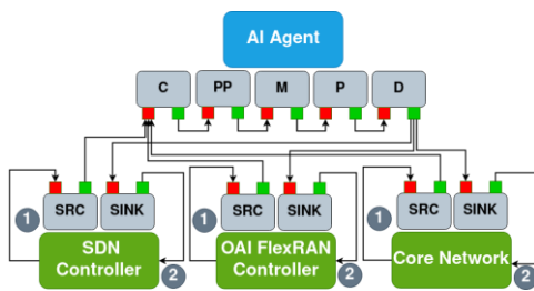
Figure 12 – ITU-T FG-ML5G ML architecture integrated into the testbed structure [41]
