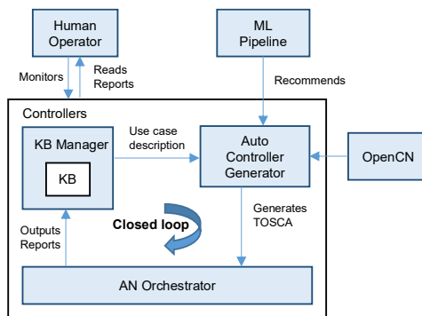
Figure 35 – High-level flow chart for creation and parsing of example intent
