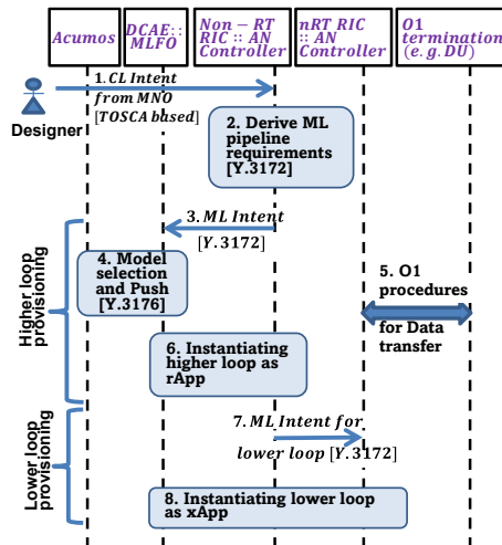
Figure 1 – Overview of the intent-based design and implementation of hierarchical closed-loops, including simulation and testbed domain
