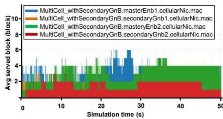
Figure 17 – Avg served blocks, DL, multiCell_withSecondaryGnb
