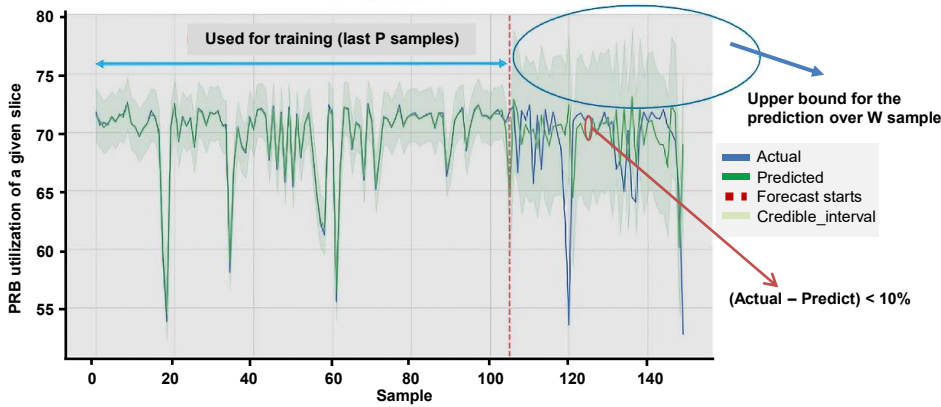
Figure 25 – Time-series forecasting of PRB utilization with GPR
