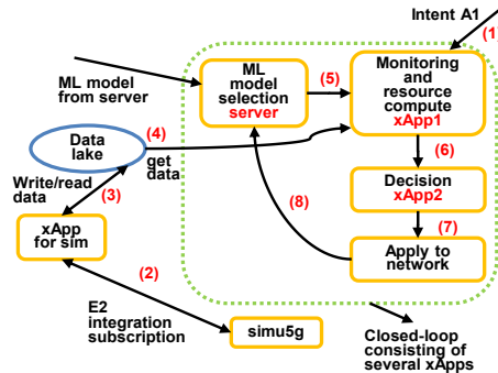
Figure 20 – Block of closed-loop implementation for an emergency slice
