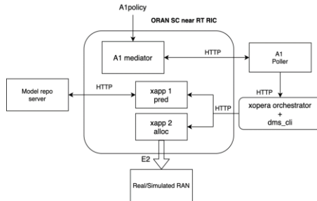
Figure 31 – Overall flow of the final integrated PoC
