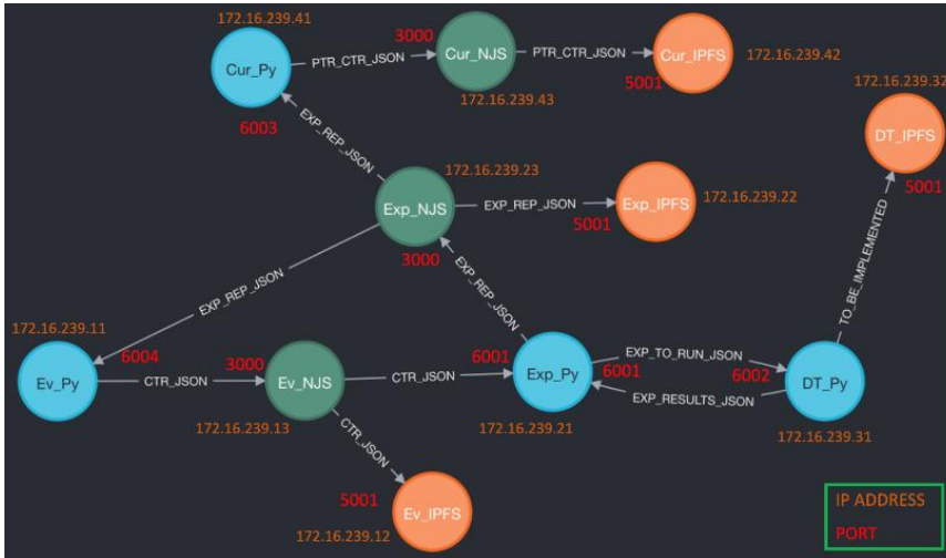
Figure 47 – Network architecture of the PoC
