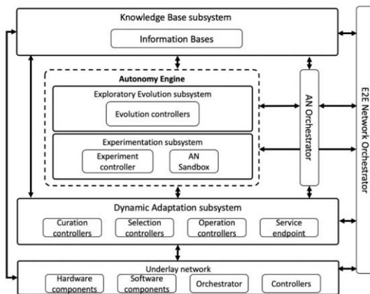
Figure 34 – High-Level Framework for Evolutionary-Driven Autonomous Network [FGAN-O-023]
