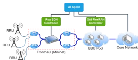
Figure 7 – Design of the proposed testbed network [41]
