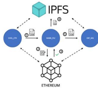
Figure 48 – Example of uploading process in the Marketplace
