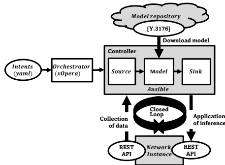
Figure 4 – Setup design for creation and parsing of example intent
