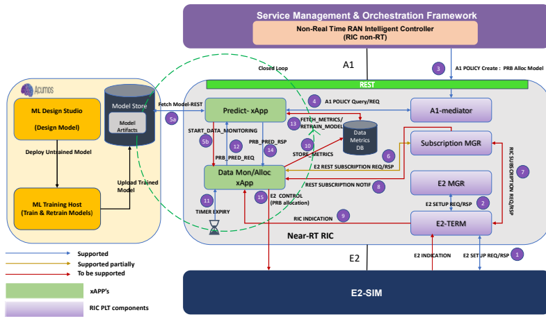
Figure 27 – Modified xApp process model
