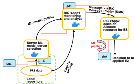
Figure 21 – Workflow of the implementation
