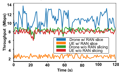
Figure 13 – Results without RAN slicing and a scenario with RAN slicing using an AI agent
