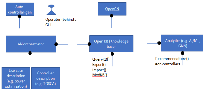
Figure 56 – Possible components diagram
