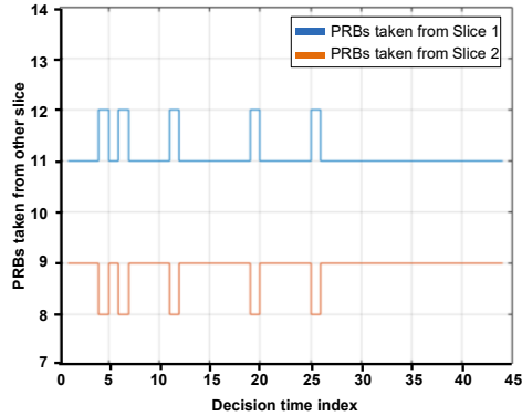
Figure 26 – PRB allocation for ES
