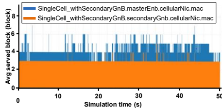
Figure 16 – Avg served blocks, DL, SingleCell_withSecondaryGnb
