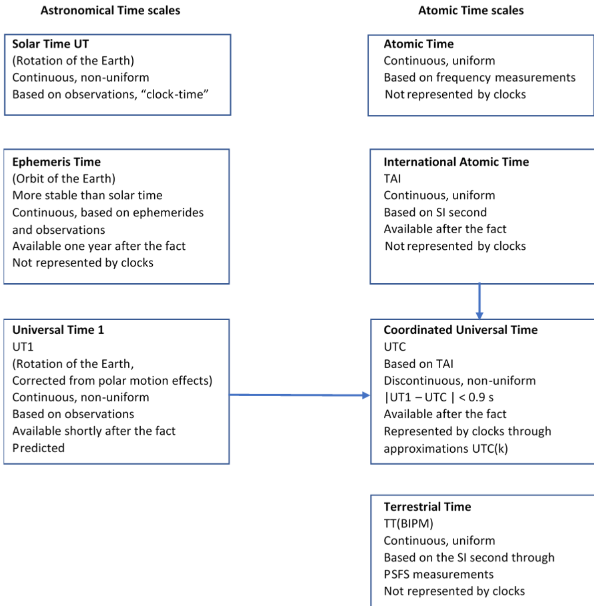
FIGURE 6 Progression of astronomical and atomic time scales
