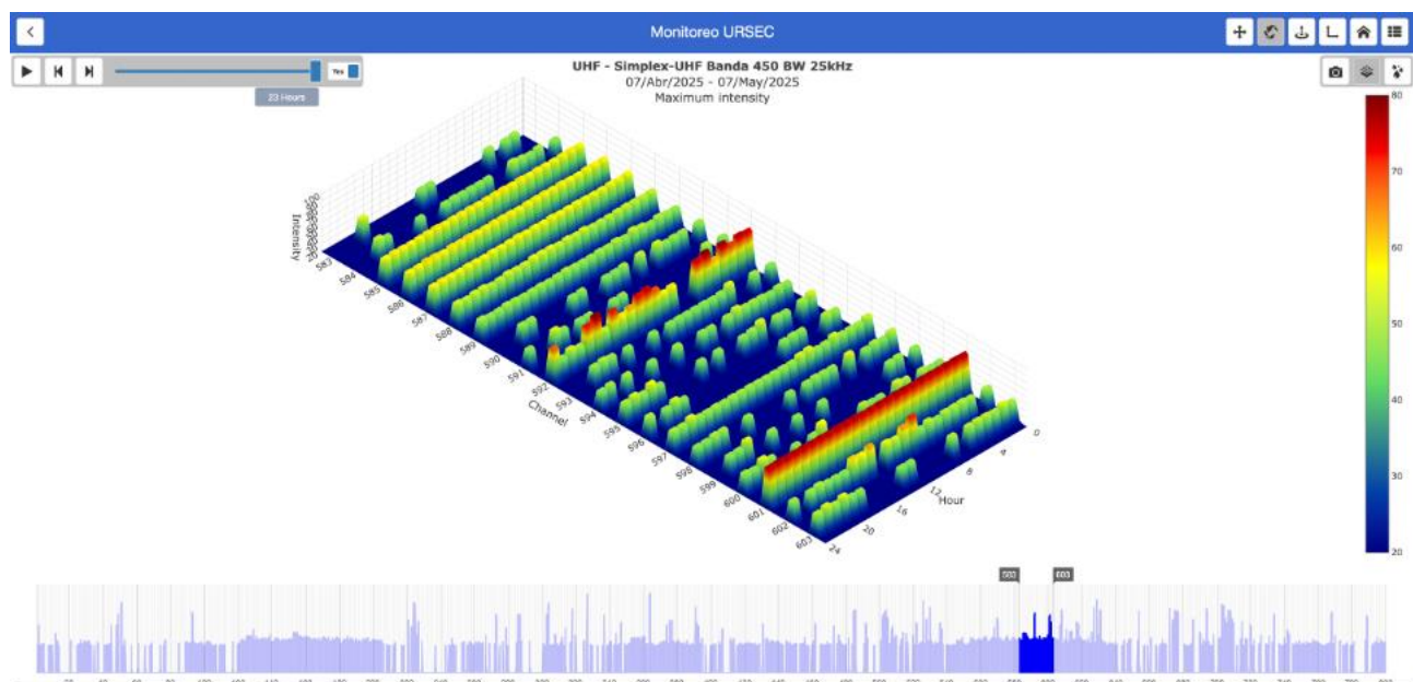
FIGURE A3-7 Online display of historical results for 800 channels in the UHF band
