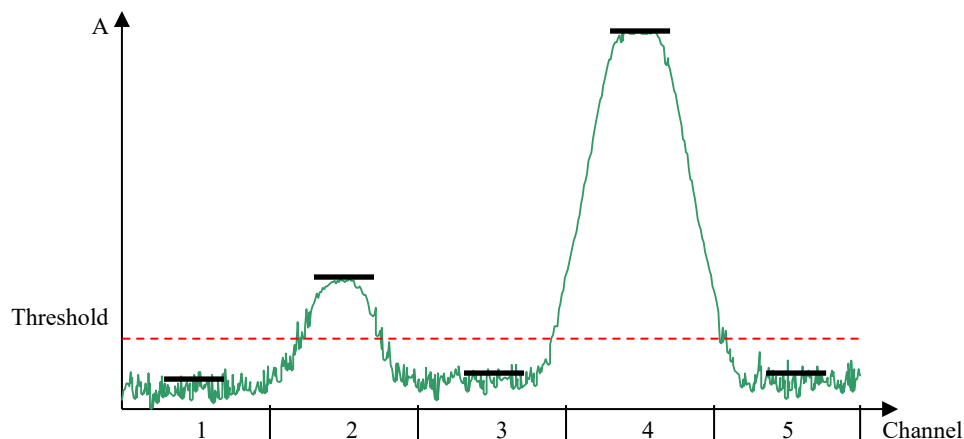
FIGURE 2 Correct setting of measurement bandwidth
