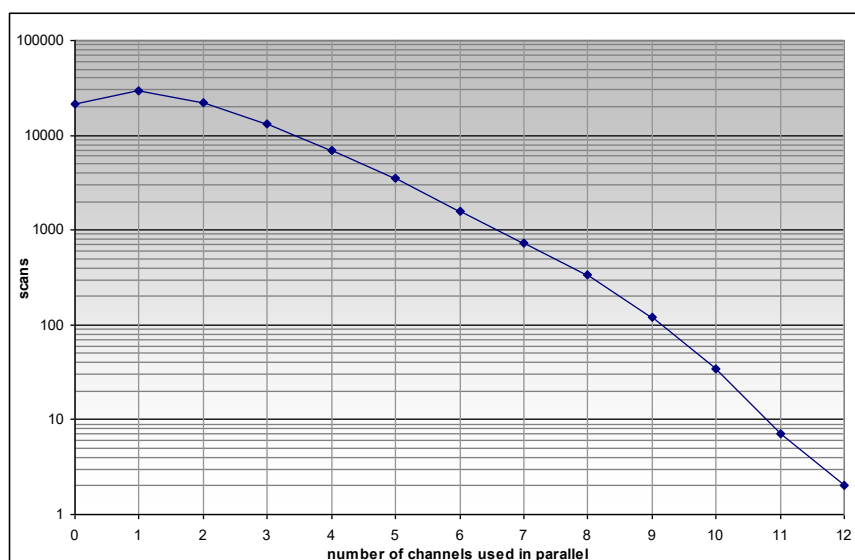
Number of scans with concurrent occupied channels
