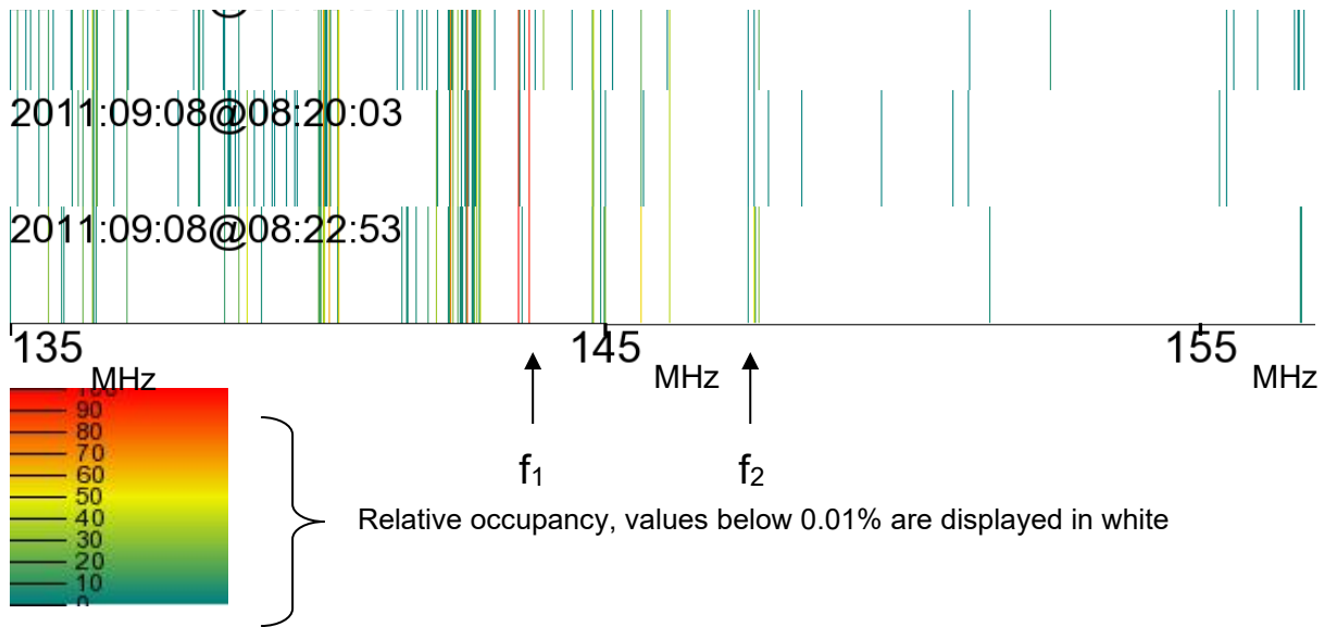
FIGURE 17 Occupancy histogram
