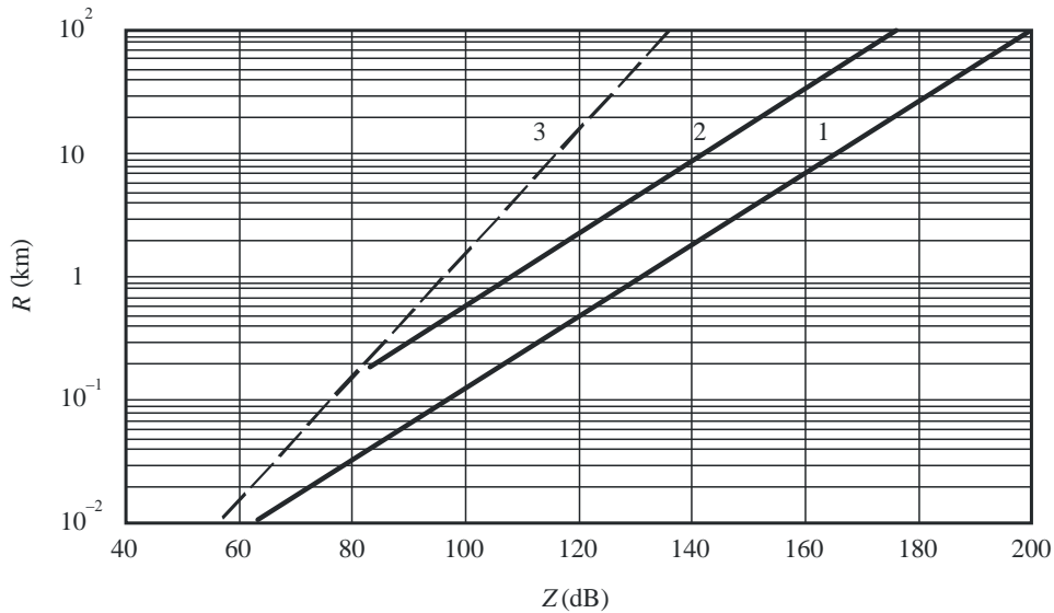
FIGURE 9 Service area radius calculation for frequencies below 1 500 MHz, h_t = 100 m 1: h_r = 1.5 m, 2: h_r = 10 m, 3: free space propagation
