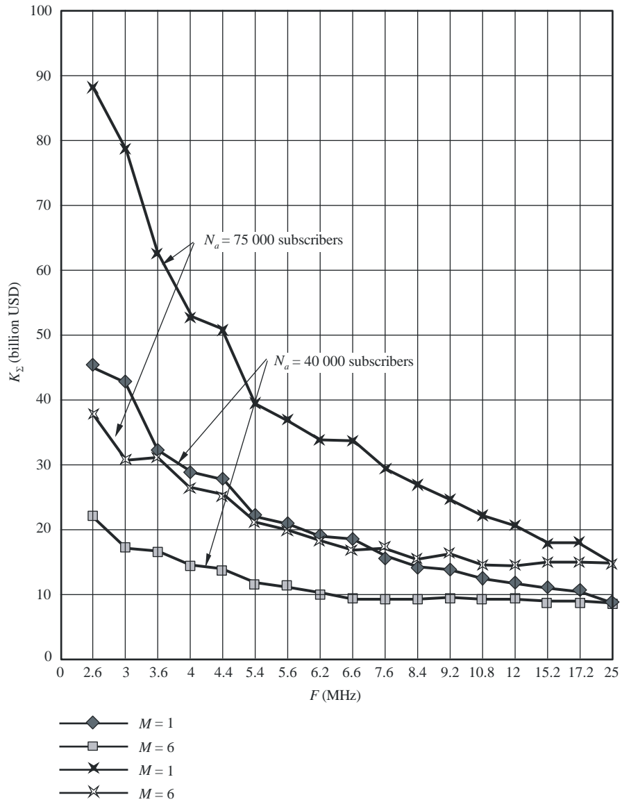
FIGURE 11 Capital investment vs. bandwidth
