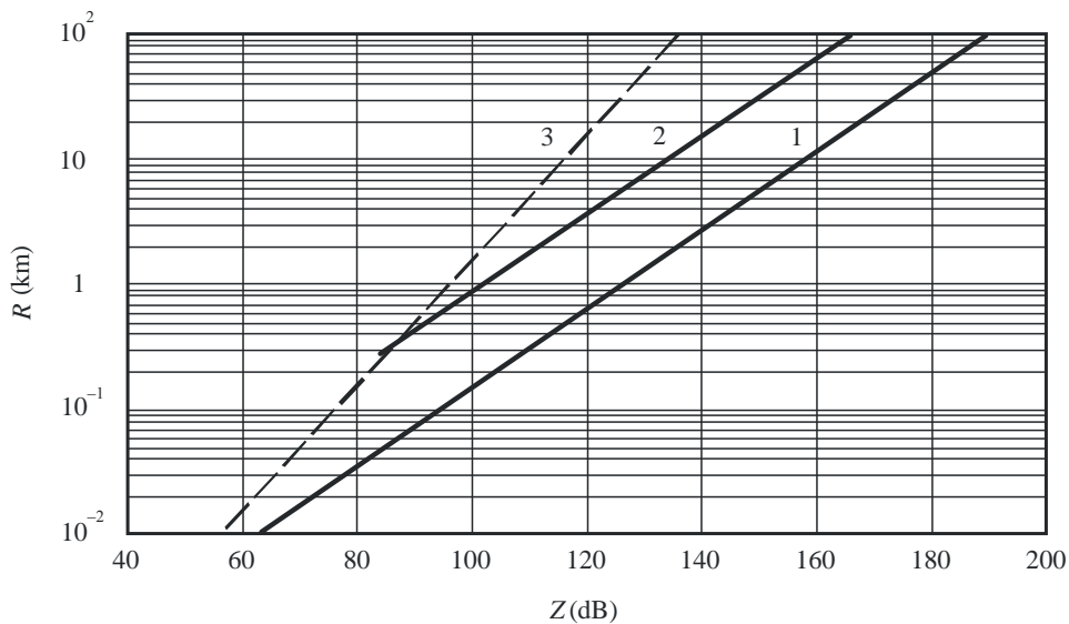
FIGURE 10 Service area radius calculation for frequencies below 1 500 MHz, h_t = 100 m 1: h_r = 1.5 m, 2: h_r = 10 m, 3: free space propagation
