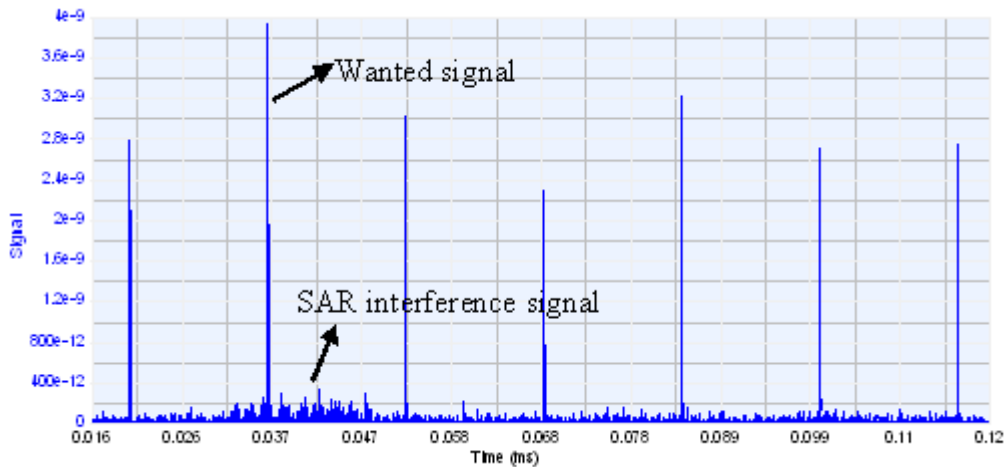
(a) Simulation result when pulse width is 10 μs
