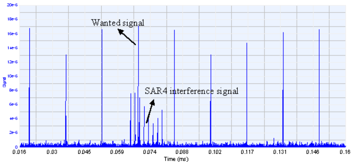
(a) Simulation result when repeat period is 20 μs
