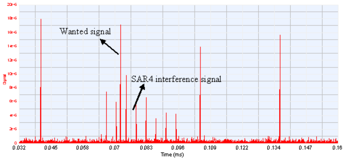
(c) Simulation result when repeat period is 80 \mu\text{s}
