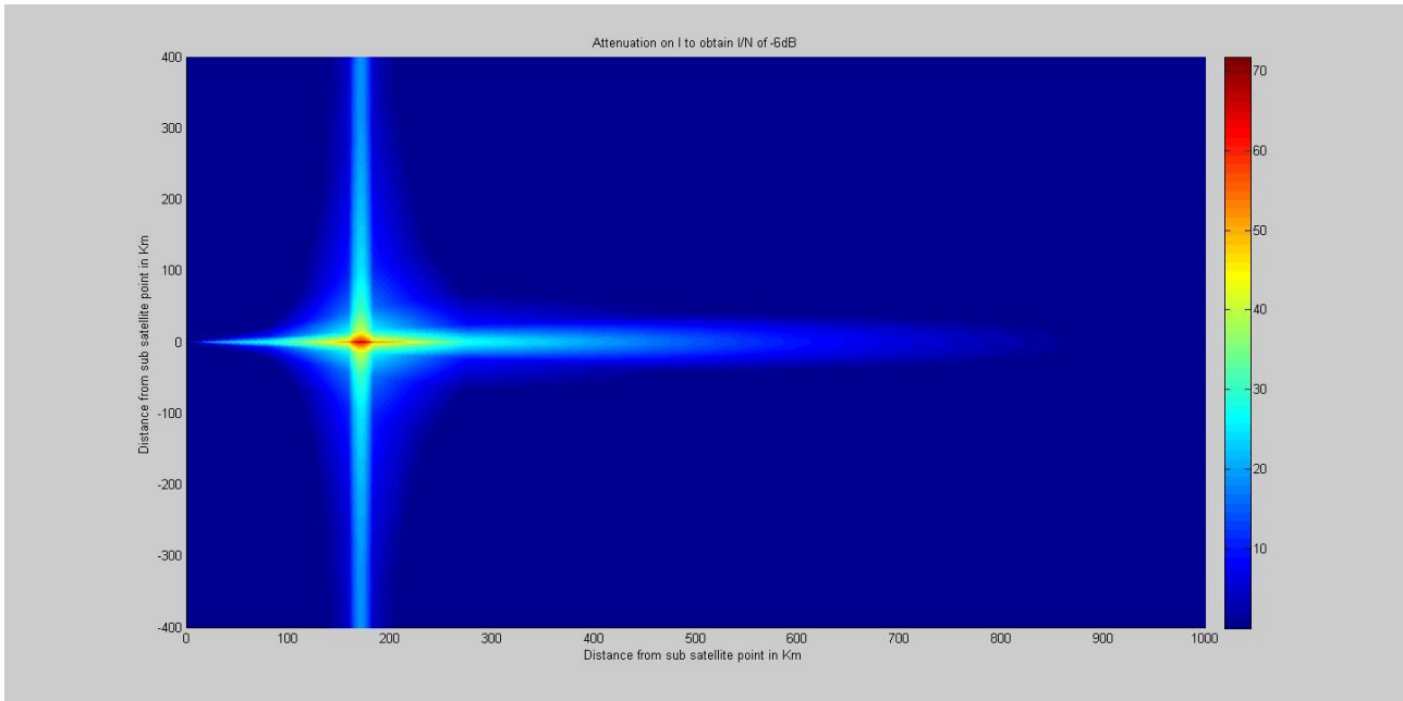
Attenuation needed to meet an I/N_{eff} of -6 dB (Radar S2)
