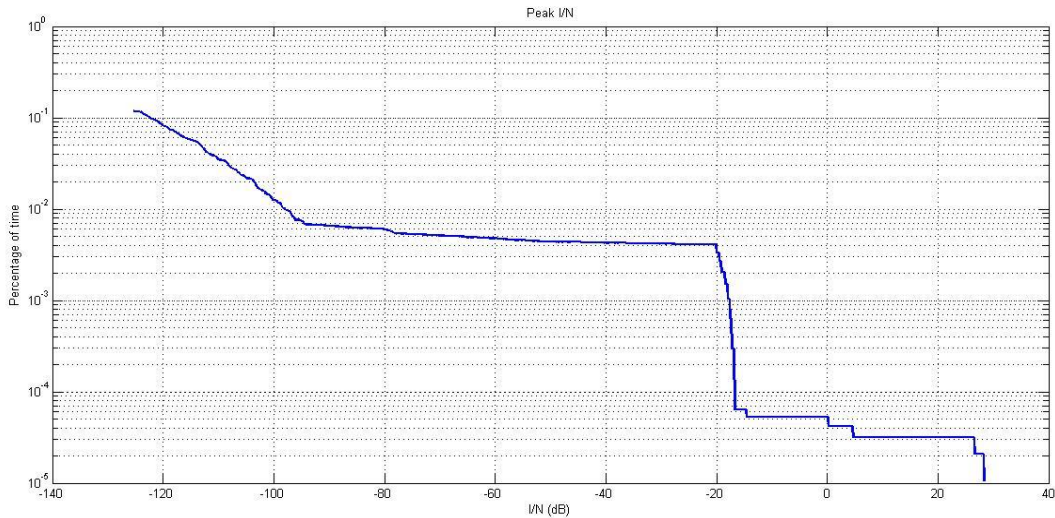
FIGURE 26 Peak I/N cdf for the GCA radar G6
