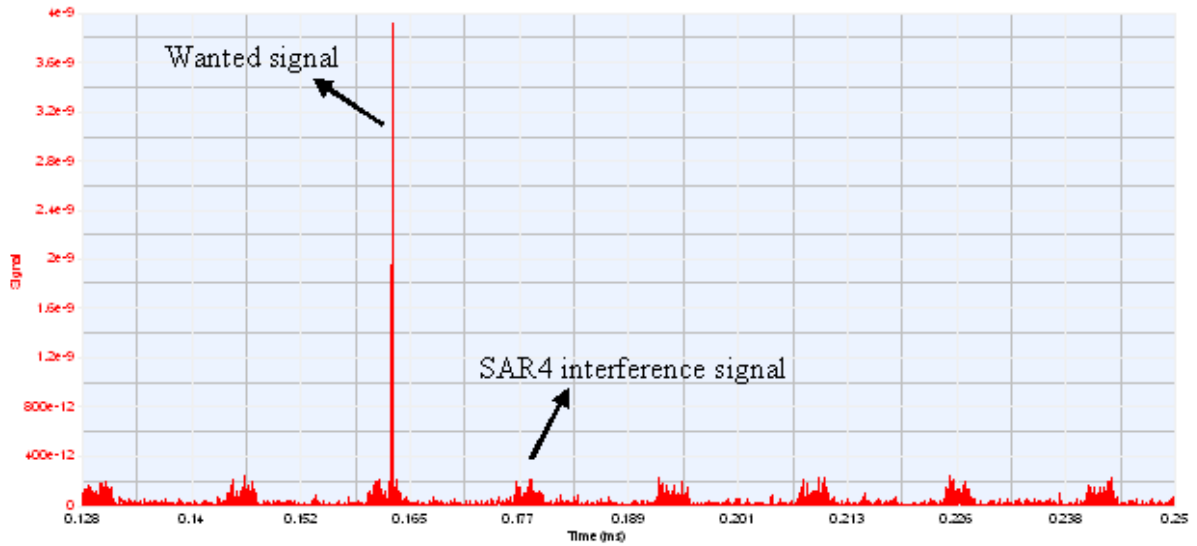
(b) Simulation result when pulse width is 4 \mu s and bandwidth is 15 MHz
