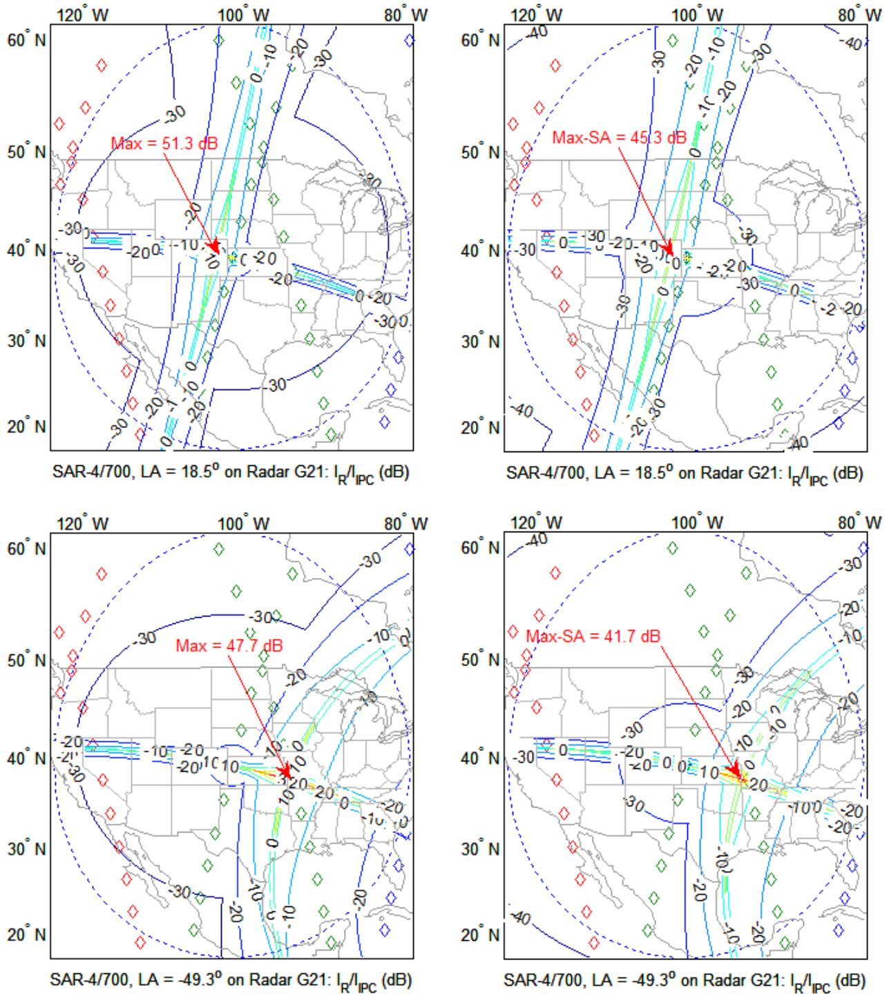
SAR-4/700 vs. Radar G21: I_R/I_{IPC} (dB) Regions
