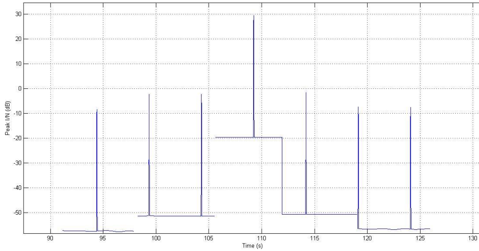
FIGURE 39 Peak I/N values for the GCA radar G6
