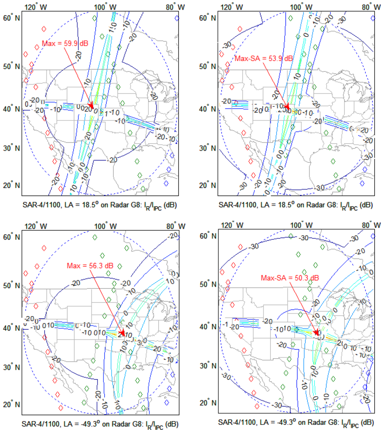
SAR-4/1100 vs. Radar G8: I_R/I_{IPC} (dB) Regions
