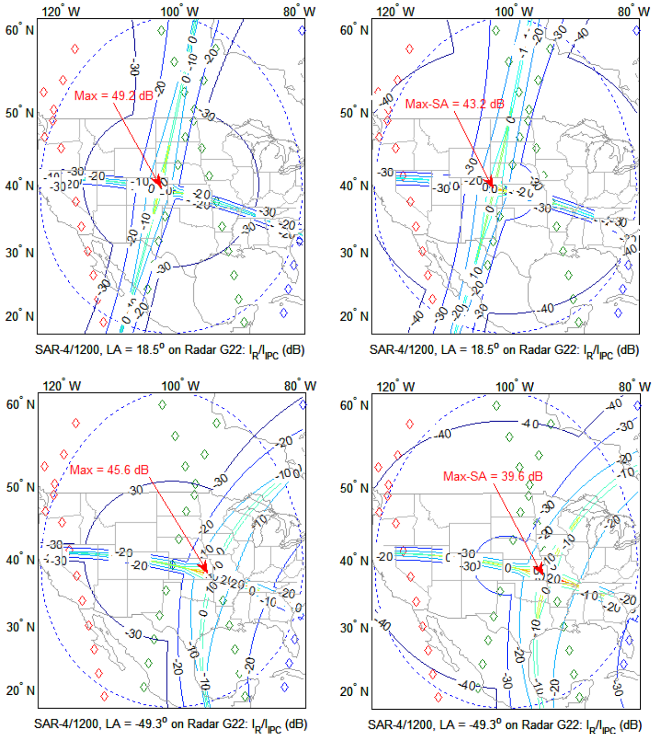
FIGURE 22 SAR-4/1200 vs. Radar G22: I_R/I_{IPC} (dB) Regions
