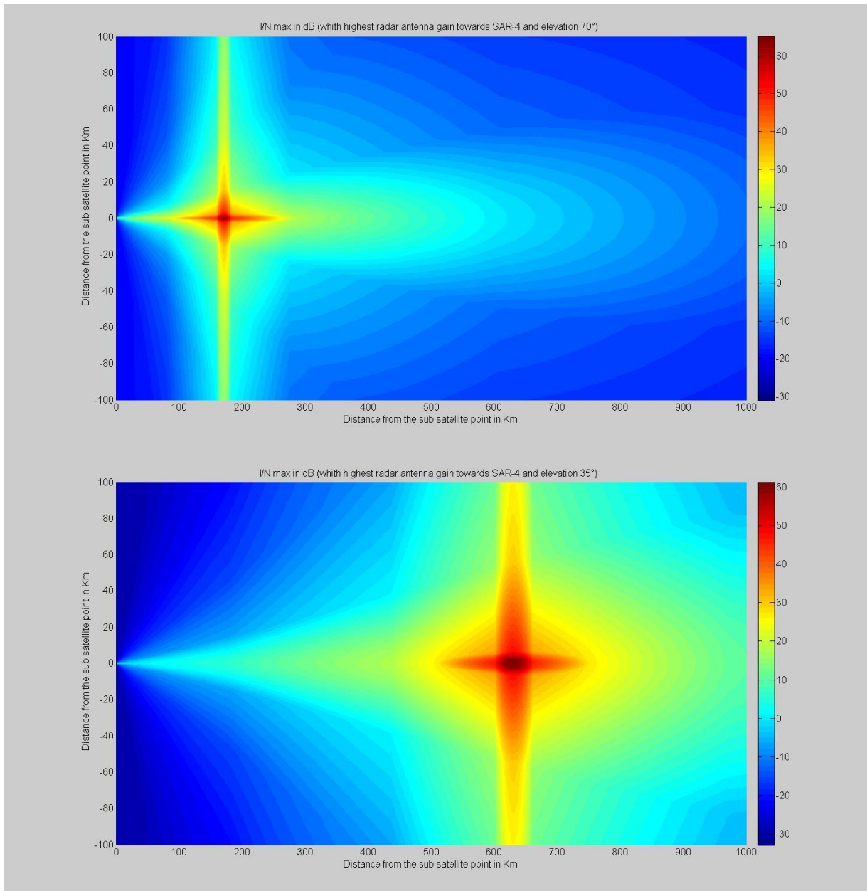
FIGURE 66 Maximum average I/N for an elevation angle 70^\circ and 35^\circ for radar G4
