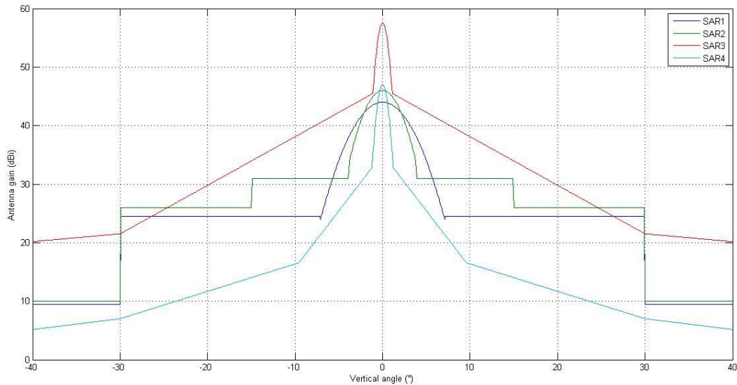
FIGURE 4 Antenna pattern cross track
