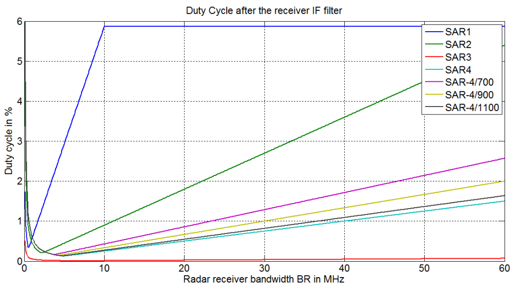
SAR systems duty cycle at the radar receiver IF output for IF bandwidth up to 60 MHz
