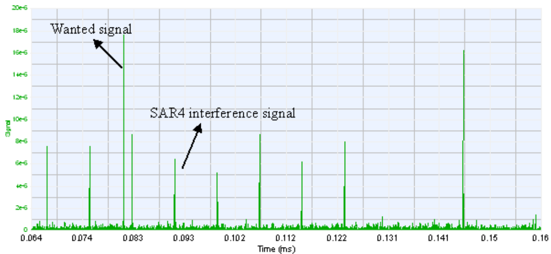
(c) Simulation result when repeat period is 80 \mu\text{s}
