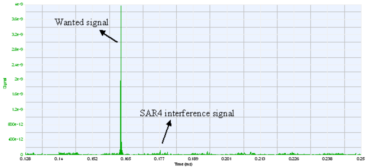
(d) Simulation result when pulse width is 12 \mu s and bandwidth is 5 MHz
