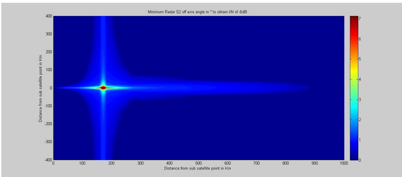
Off-axis angle needed to meet an I/N_{eff} of -6 dB (Radar S2)
