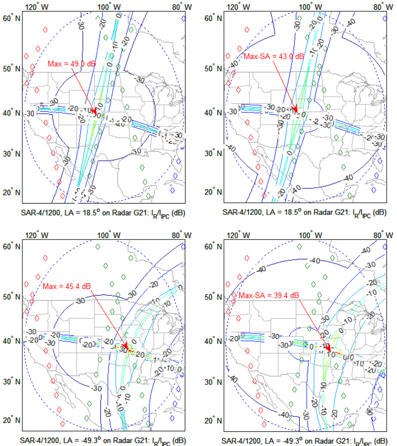
FIGURE 20 SAR-4/1200 vs. Radar G21: I_R/I_{IPC} (dB) Regions
