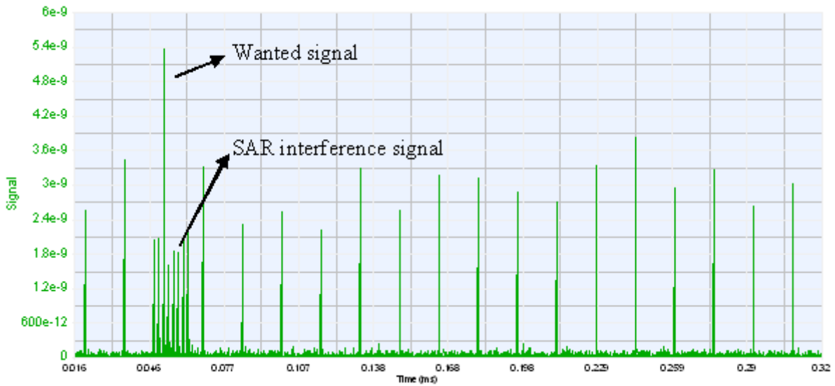
(c) Simulation result when repeat period is 400 \mu s
