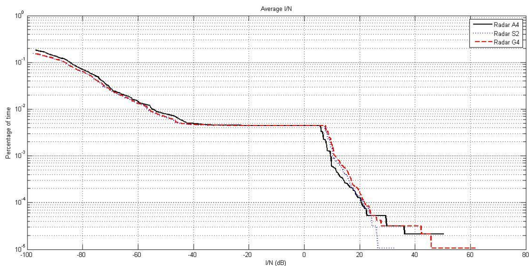
FIGURE 71 Average I/N values random pointing angles ( Radar processing gain not taken into account P_G = 0 dB )
