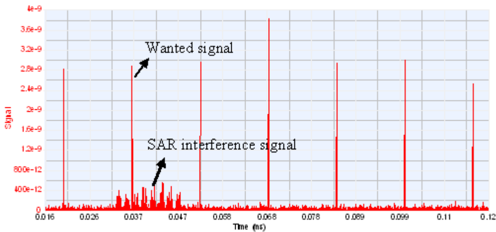
(b) Simulation result when pulse width is 20 μs
