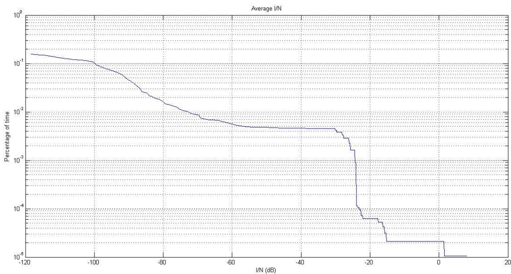
FIGURE 27 Average I/N cdf for the GCA radar G6
