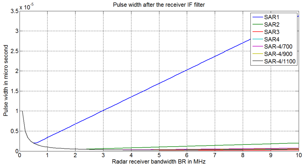
SAR systems pulse width at the radar receiver IF output for up to 10 MHz IF bandwidth
