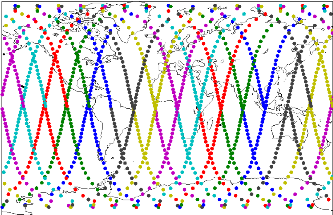
FIGURE 13 SAR-4 ground tracks for 14 orbital periods (each 1 hr 34 min 49 s)
