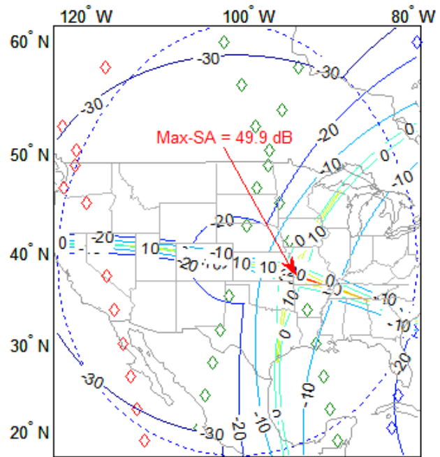
SAR-4/1200, LA = -49.3° on Radar G8: I_R/I_{PC} (dB)
