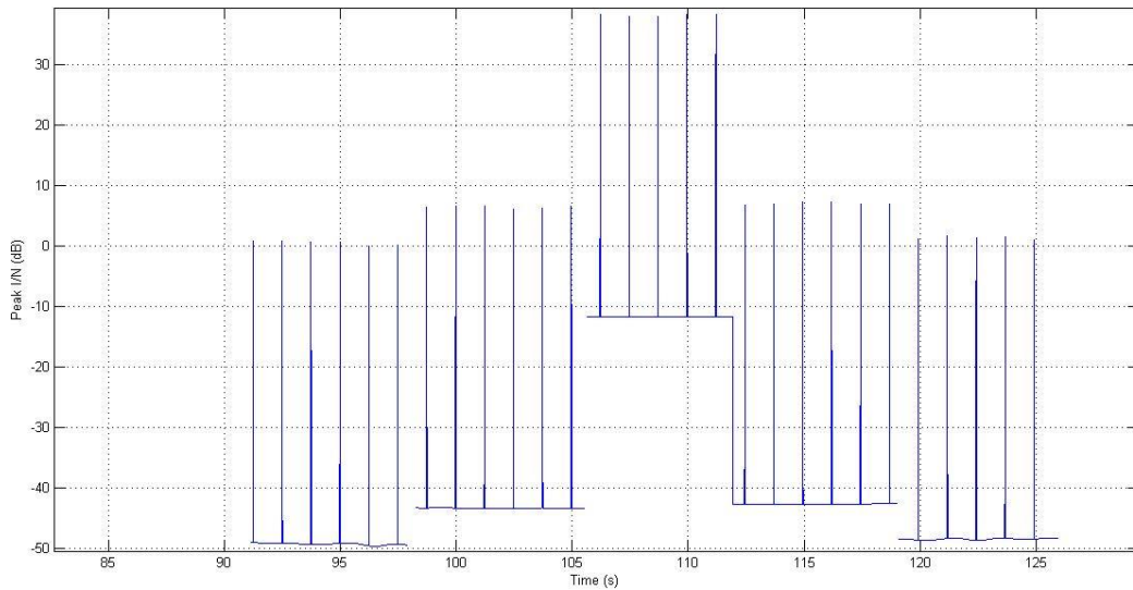
FIGURE 45 Peak I/N values for the maritime radar S14
