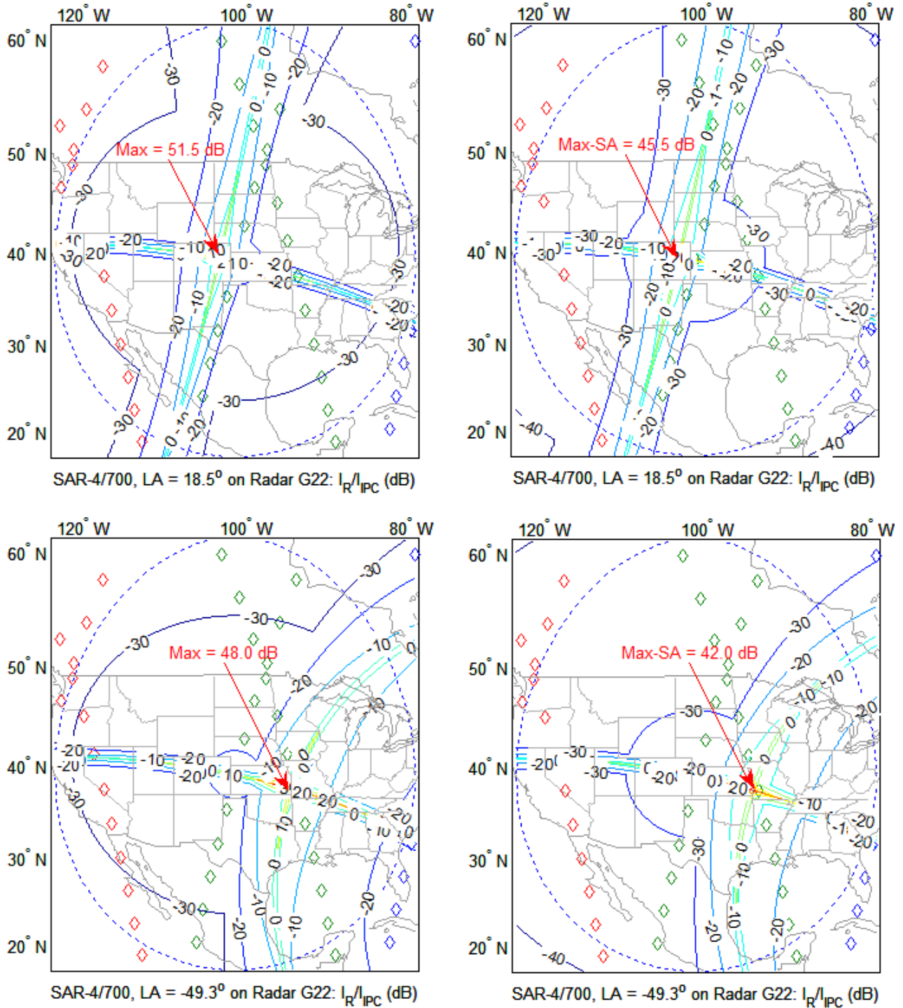
SAR-4/700 vs. Radar G22: I_R/I_{PC} (dB) Regions
