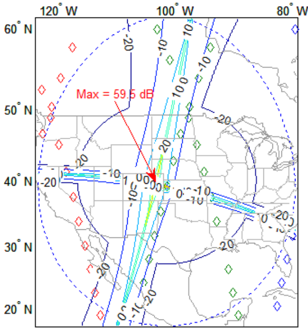
SAR-4/1200, LA = 18.5° on Radar G8: I_R/I_{PC} (dB)
