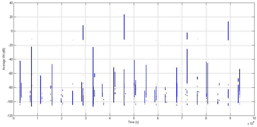
FIGURE 35 Average //N vs time for the ASDE radar G8
