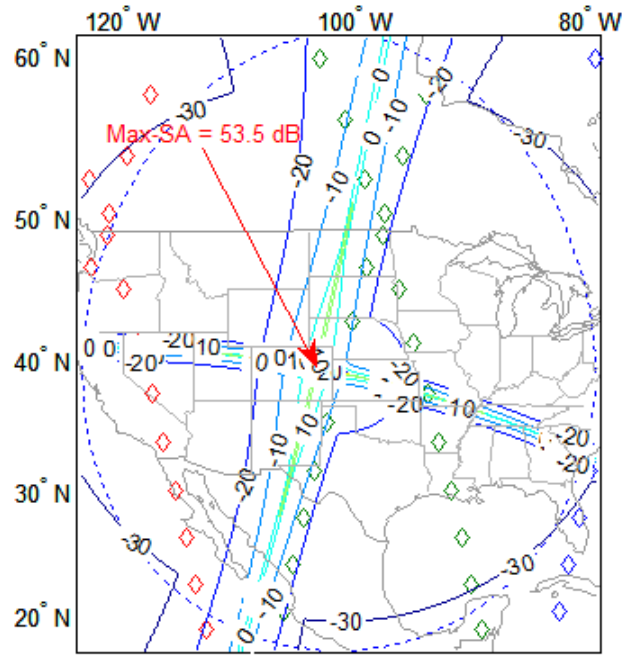
SAR-4/1200, LA = 18.5° on Radar G8: I_R/I_{PC} (dB)
