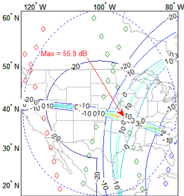
SAR-4/1200, LA = -49.3° on Radar G8: I_R/I_{PC} (dB)
