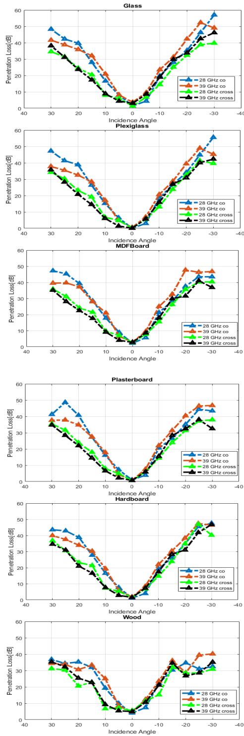
FIGURE 3 Penetration loss vs incident angle for all materials at 28 GHz and 39 GHz in co-polar (VV) and cross-polar (HV) alignments
