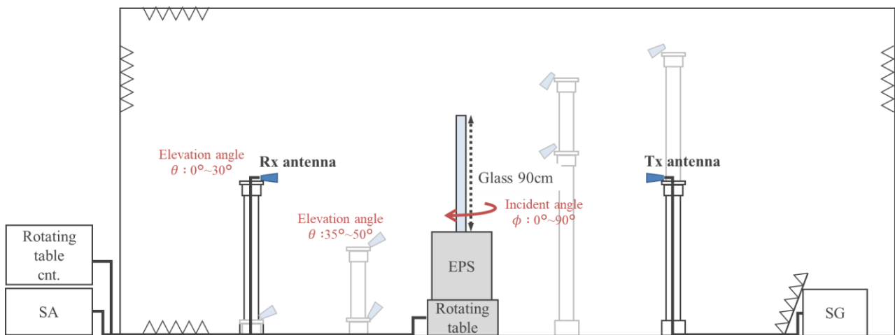
Configuration of the measurement system
