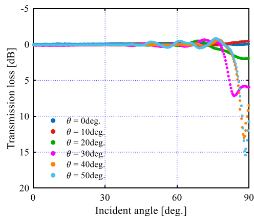
FIGURE 7 Measurement results without glass
