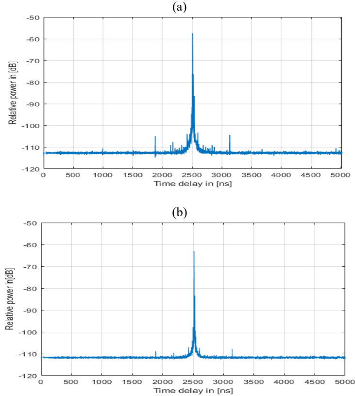
FIGURE 2 Measured power delay profiles at 28 GHz cross-polar at 90° incident angle (a) Free space, (b) Wood flooring
