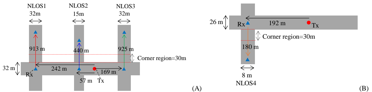
FIGURE 7 Measurement routes at (a) Tx1 (b) Tx2
