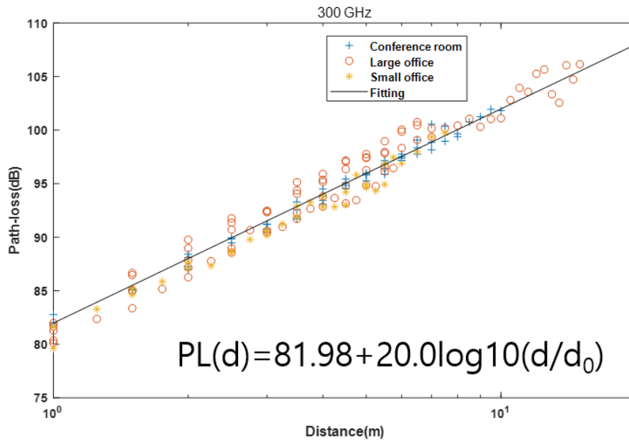
FIGURE 105 Transmission loss measurement results in office environments at 300 GHz
