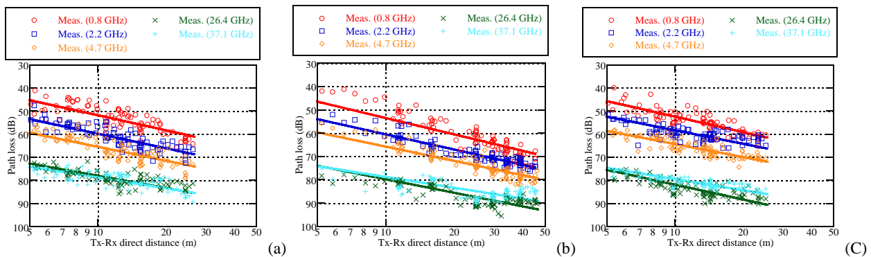
Measurement results and regression results: (a) Tx1, (b) Tx2, (c) Tx3
