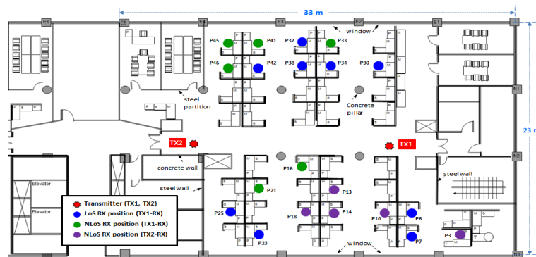
FIGURE 84 Layout of measurement scenario in a typical office environment
