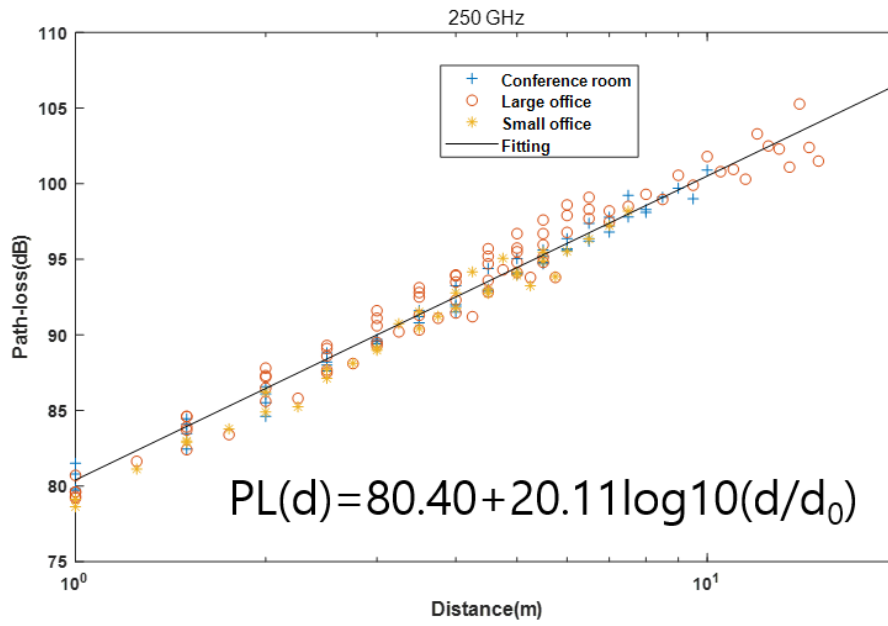
FIGURE 103 Transmission loss measurement results in office environments at 250 GHz
