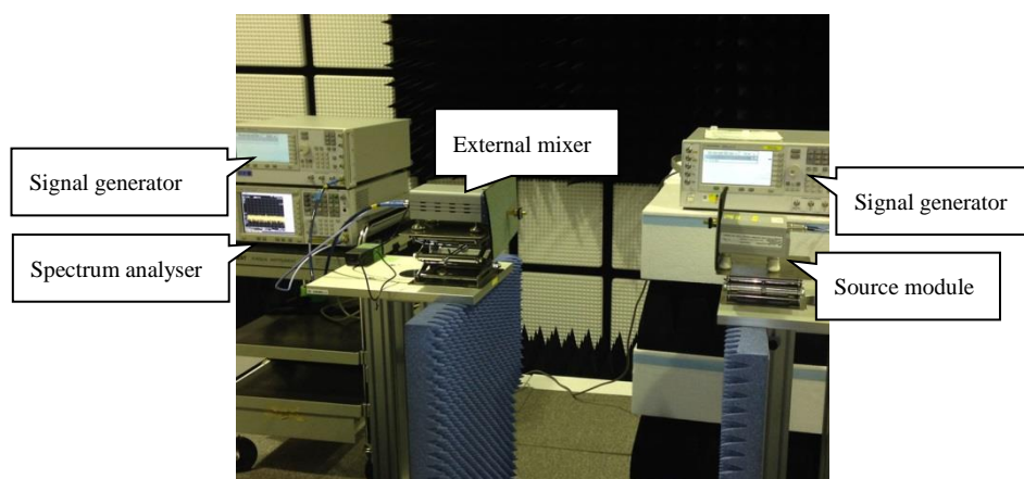
Propagation measurement in anechoic chamber
