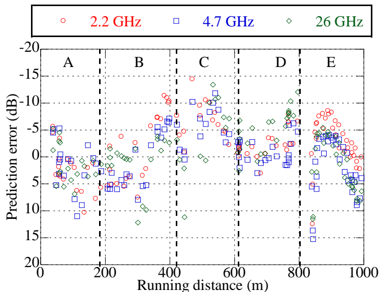
Prediction error versus running distance
