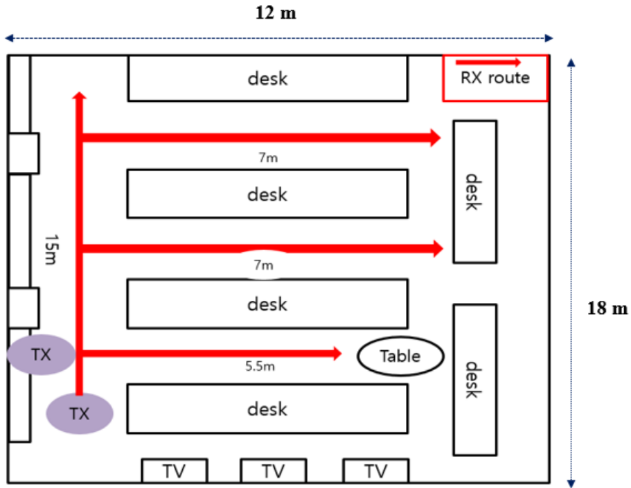
FIGURE 99 Measurement scenarios in a large office environment (a) Measurement environment
