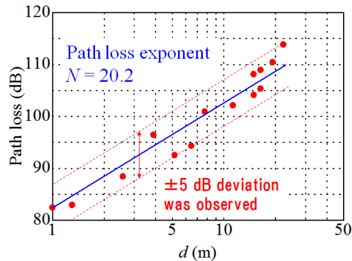
FIGURE 62 Measured transmission loss results in the data centre environment
