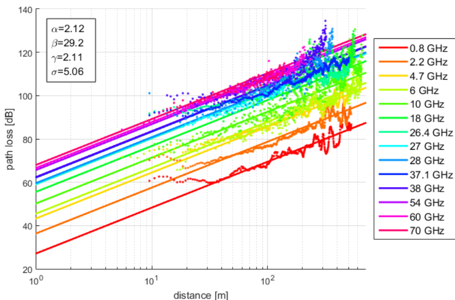
Basic transmission loss for LoS in below-rooftop urban and suburban environments
