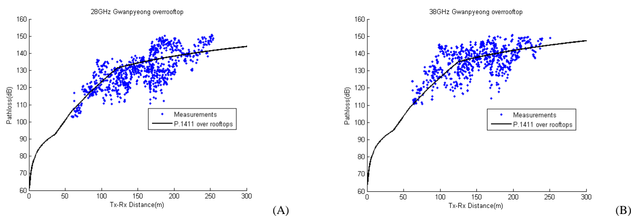
Comparison of the measurements and Rec. ITU-R P.1411 over rooftops at (a) 28 GHz and (b) 38 GHz
