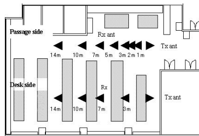
FIGURE 52 Measurement environment (Office)
