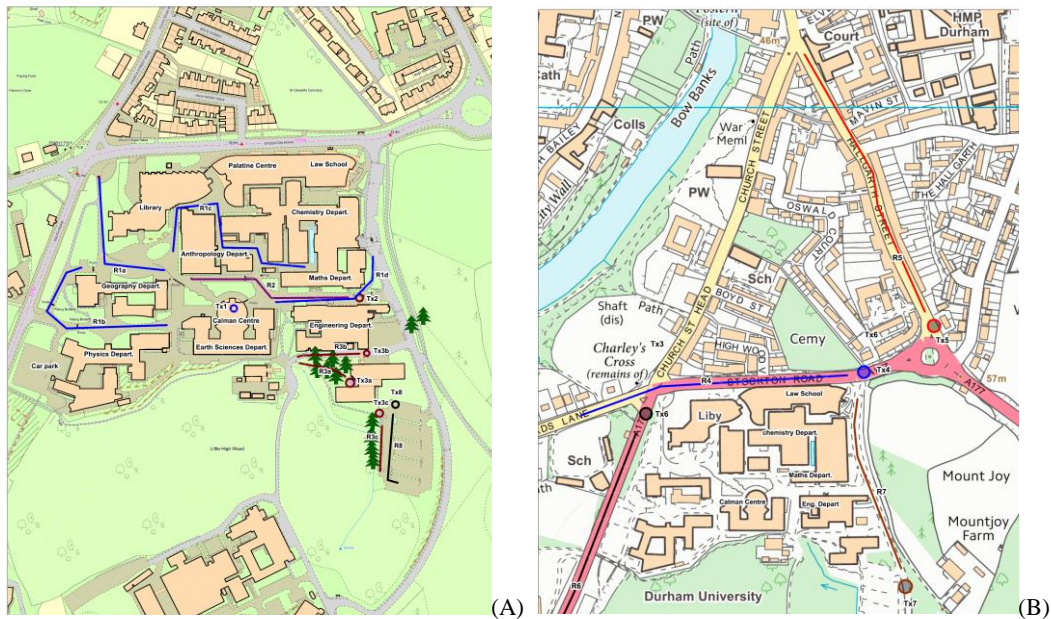
FIGURE 31 Routes of measurement scenarios (a) routes 1-3 and 8, (b) routes 4 and 7
