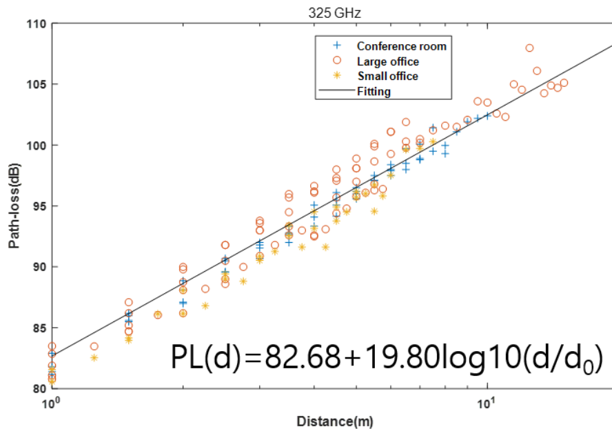
FIGURE 106 Transmission loss measurement results in office environments at 325 GHz
