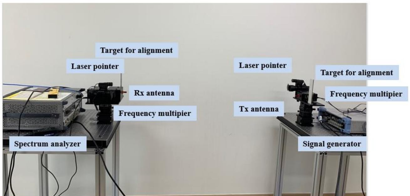
FIGURE 95 Measurement configuration
