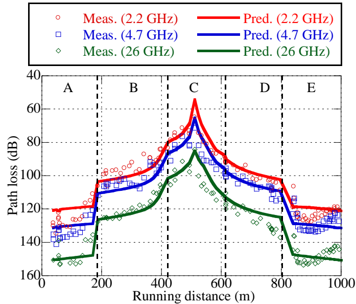
Predicted and measured total basic transmission loss
