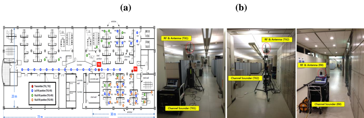
Basic transmission loss measurement campaign in an ETRI office (Site 1): (a) Layout of the measurement scenario, (b) Installation of measurement equipment
