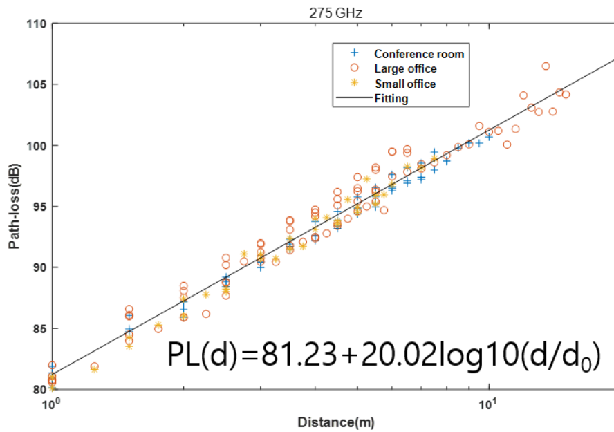
FIGURE 104 Transmission loss measurement results in office environments at 275 GHz
