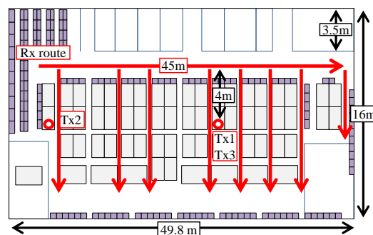
Measurement environment
