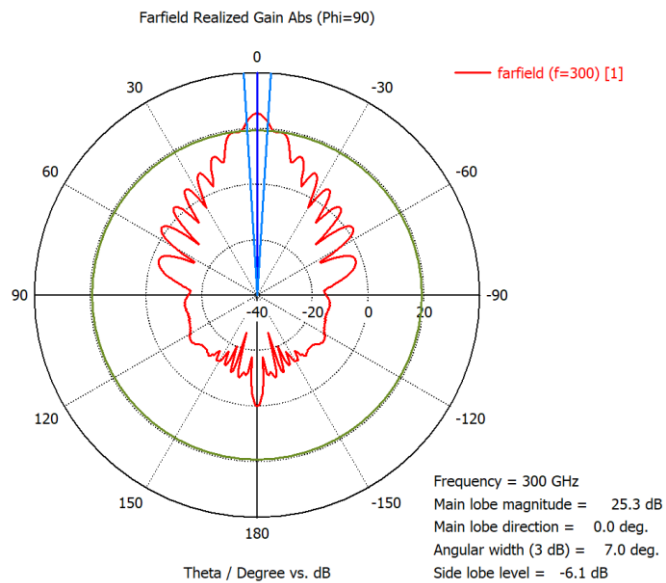
FIGURE 97 Standard gain horn antenna for TX and RX
