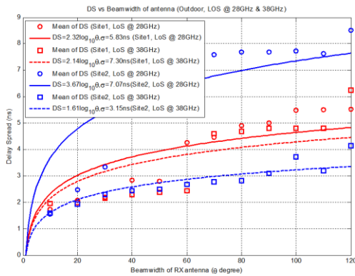
FIGURE 29 Measurement results of rms delay spread for 28 and 38 GHz: (a) LoS case (b) NLoS case
