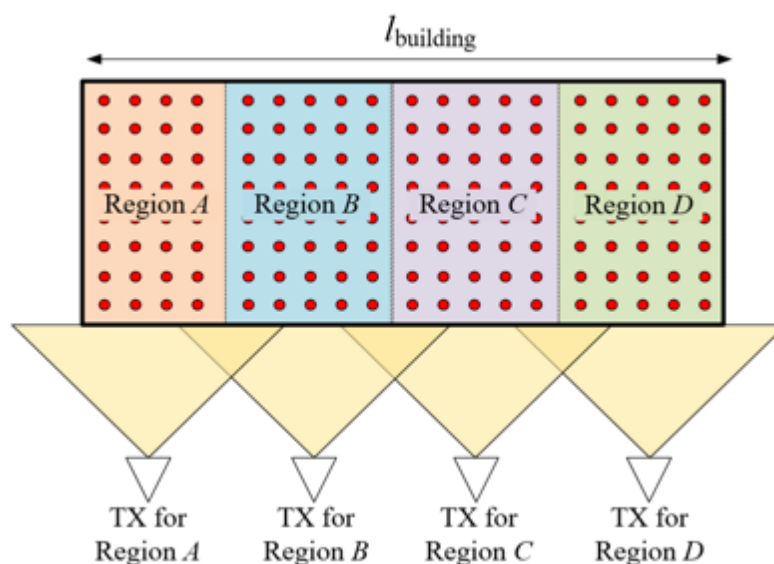
TX positions for near perpendicular incidences
