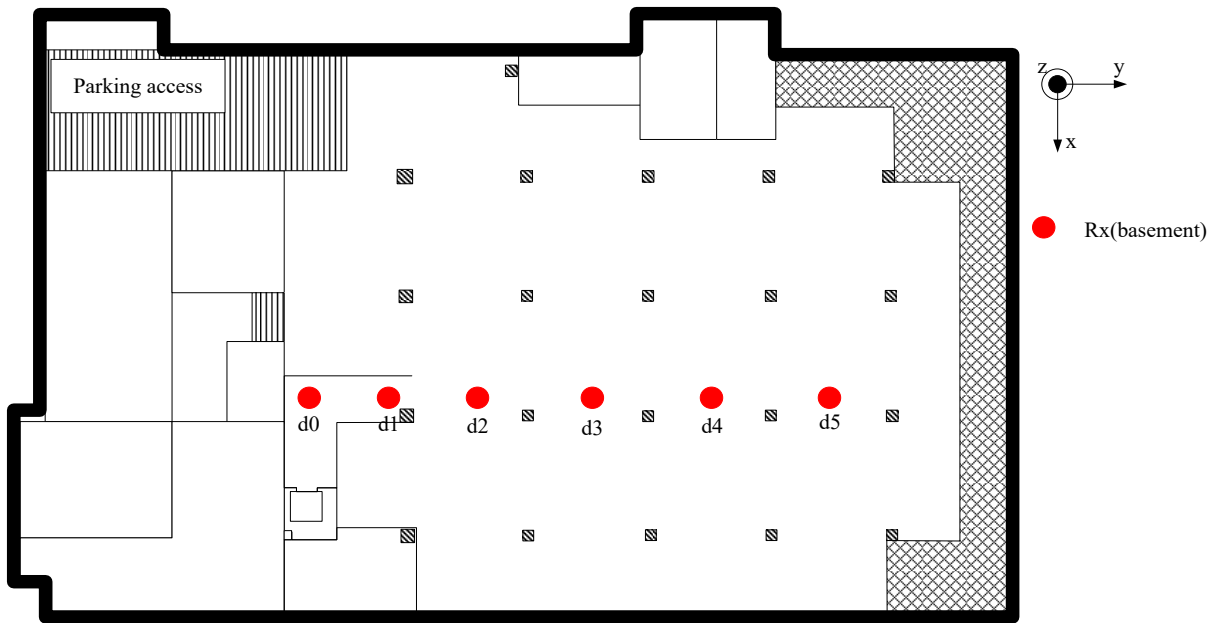
FIGURE 319 The Tx and Rx points for measuring penetration loss between the first floor and the basement: (a) basement, (b) first floor
