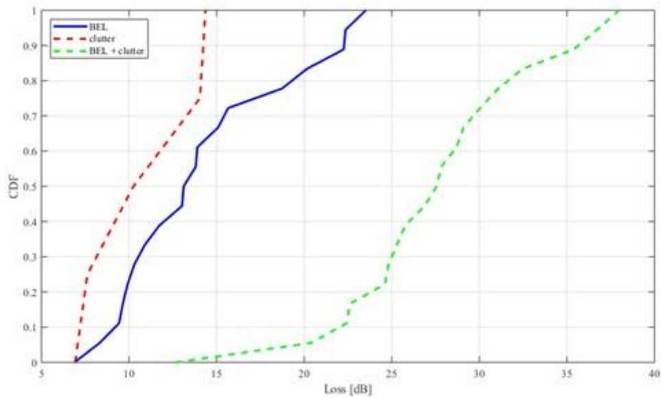
FIGURE 337 3 GHz BEL and BEL+clutter loss
