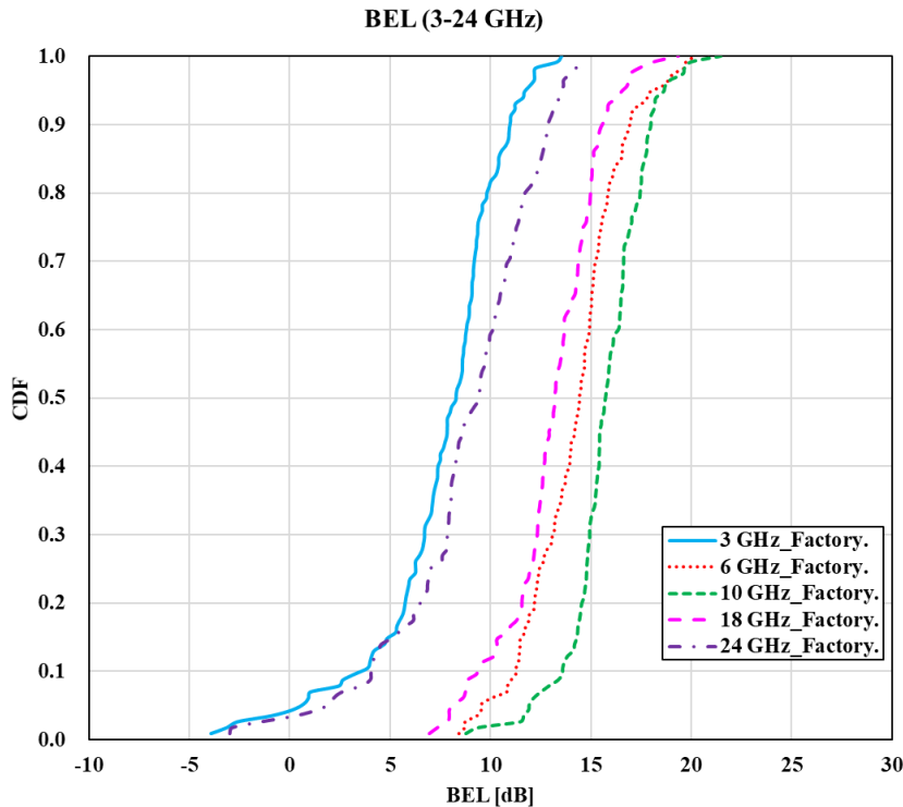
FIGURE 309 3-24 GHz CDF characteristics of the building entry loss
