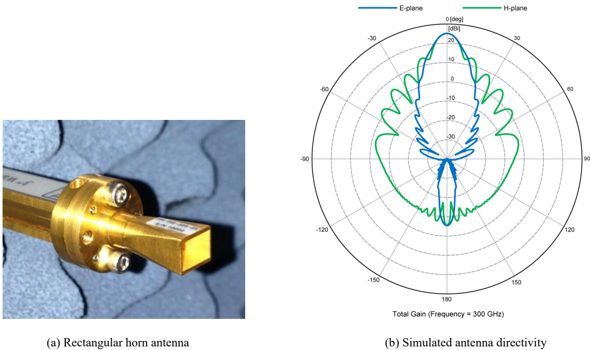
FIGURE 362 Antenna for the measurement
