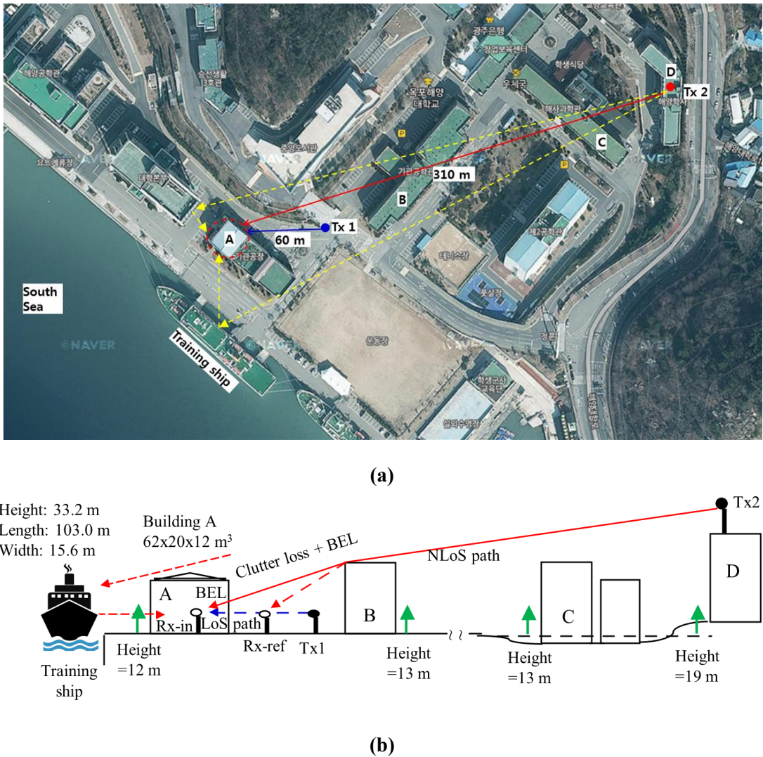
FIGURE 324 Measurement site and environments (a) in MMU' campus in Korea and (b) the height of the main buildings over the NLoS path
