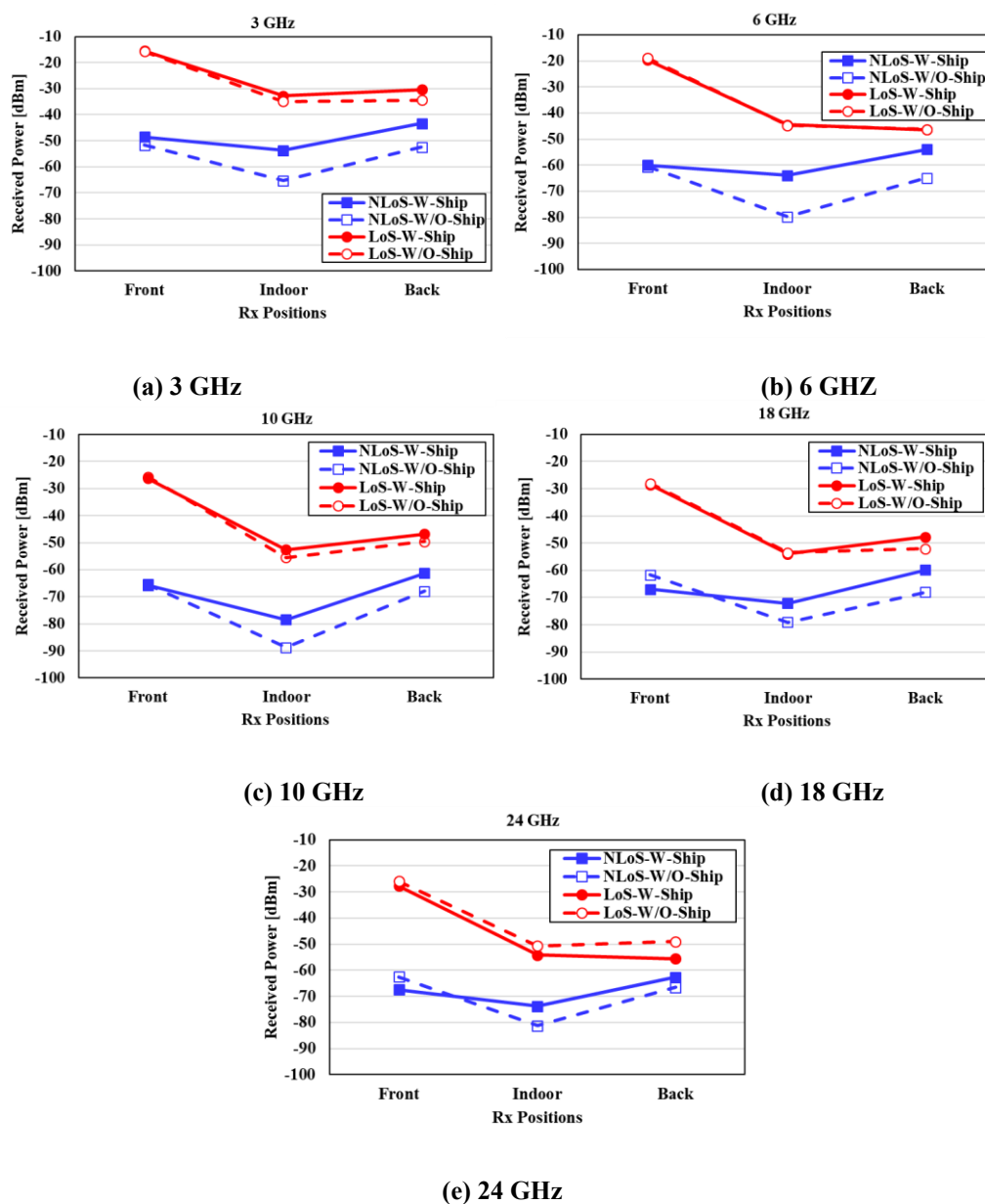
Power measured at the front, inside and back side of Building A
