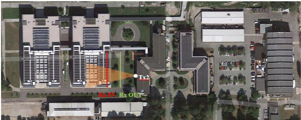
FIGURE 347 Scenario top view with 3 dB antenna beam width coverage
