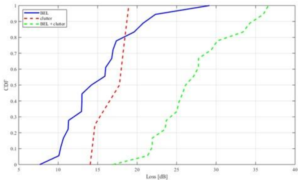
FIGURE 338 24 GHz BEL and BEL+clutter loss
