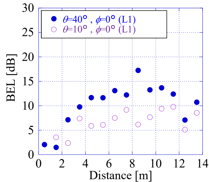
FIGURE 374 Measurement result for \theta dependency
