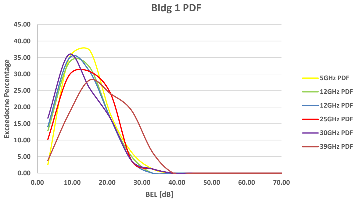
FIGURE 197 BEL PDFs for building 1
