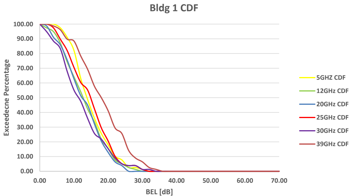
FIGURE 202 BEL CDFs for building 1
