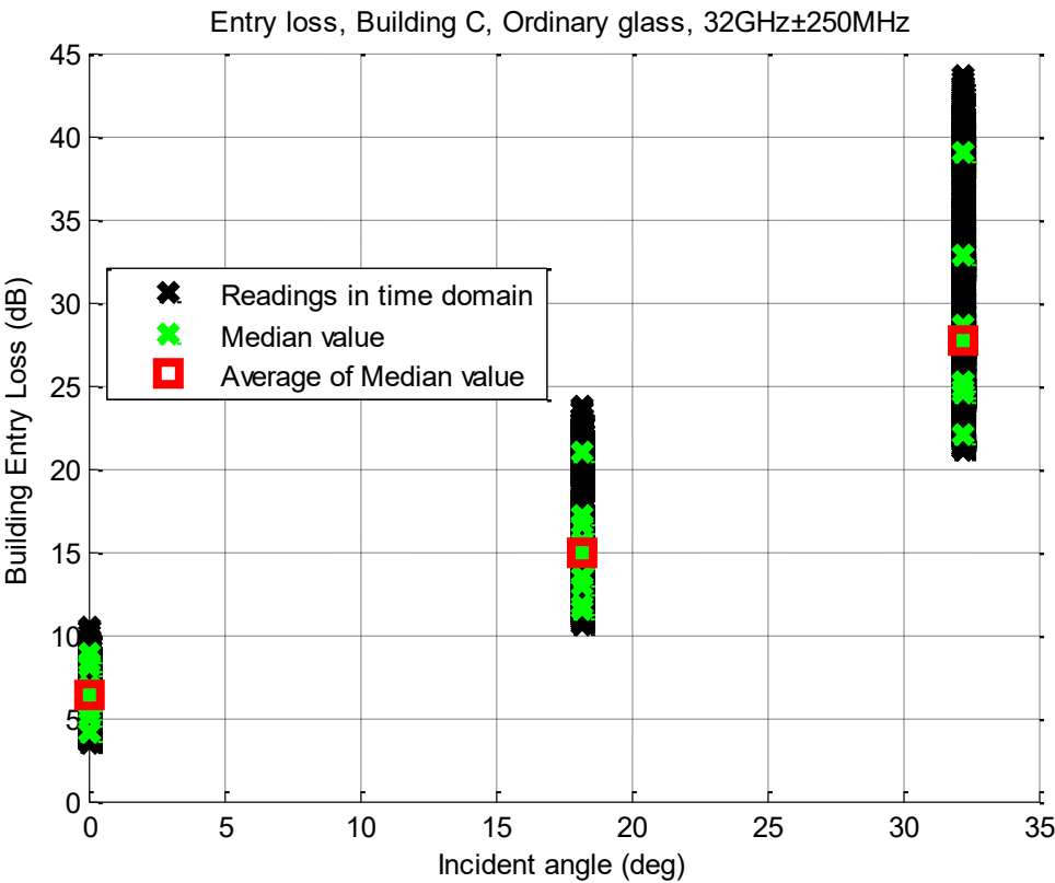
FIGURE 221 500 continuous reading->Median value of BEL at 11 frequencies->Average of Median value
