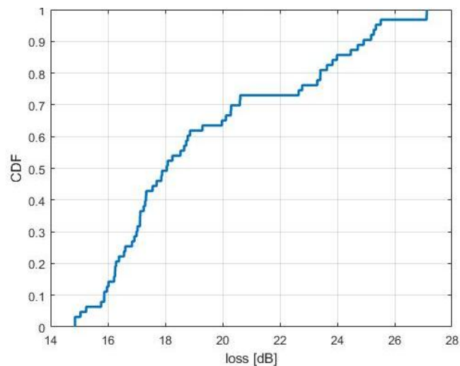
FIGURE 353 Clutter loss CDF
