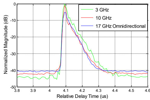
FIGURE 79 PDPs across the frequency bands for R33
