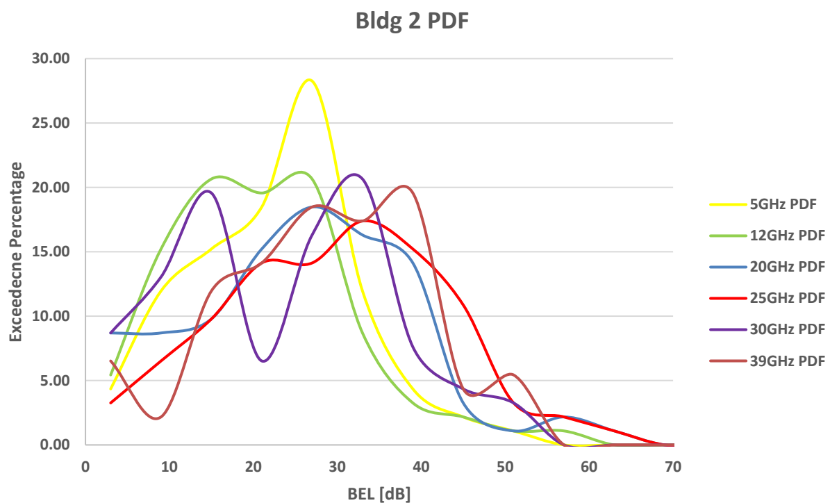
FIGURE 198 BEL PDFs for building 2
