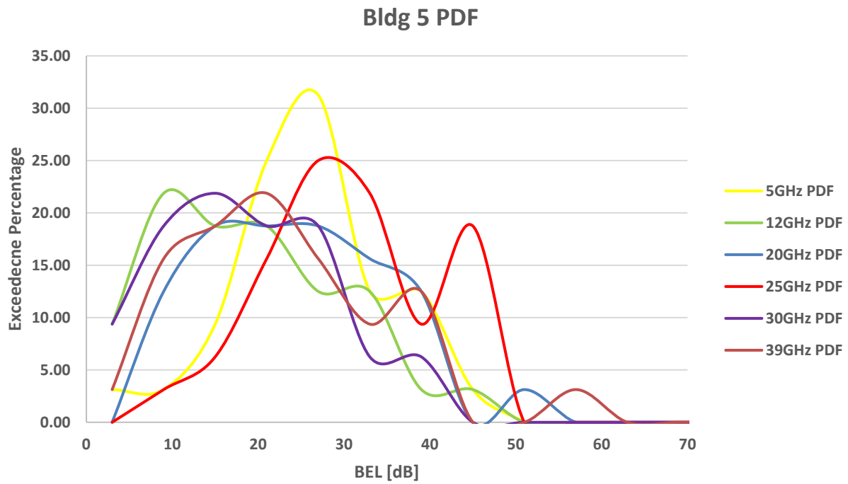
FIGURE 201 BEL PDFs for building 5
