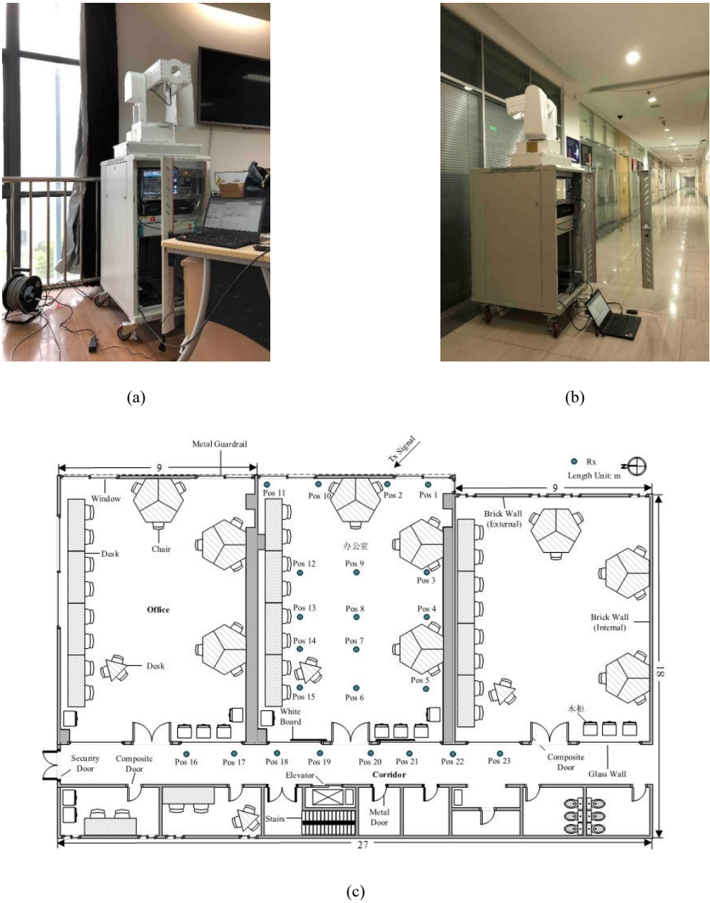
Indoor office receiver locations
