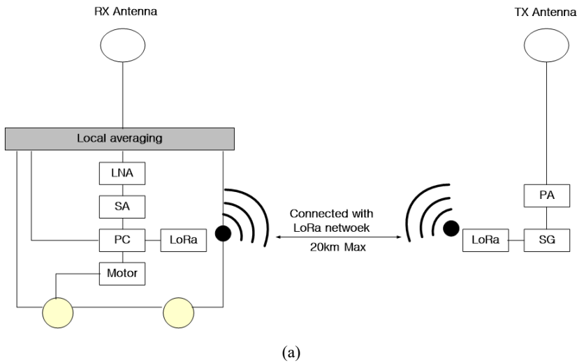
Building entry loss measurement set-up (a) and transmitter and receiver (b) for Factory B
