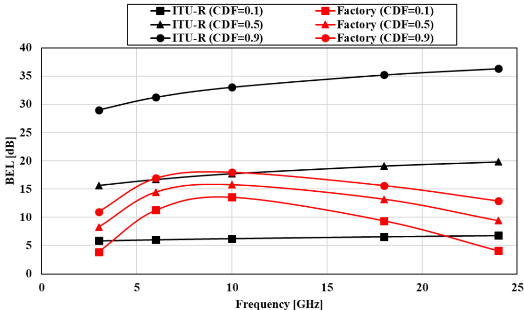
FIGURE 310 Frequency dependency of building entry loss at 10, 50 and 90 percentile levels
