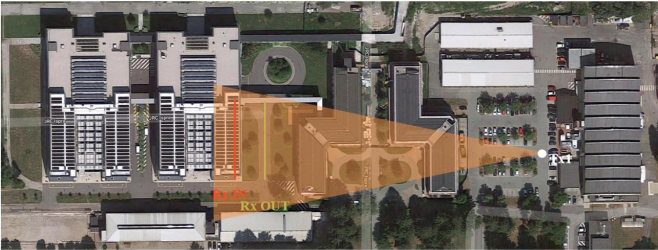
FIGURE 344 Scenario top view with 3 dB antenna beam width coverage
