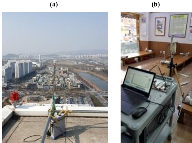
FIGURE 334 Measurement environment (a) Tx for clutter loss (b) Rx for clutter loss(inside)
