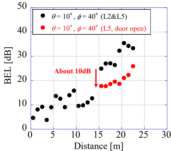
FIGURE 376 Measurement result showing the effects of the door
