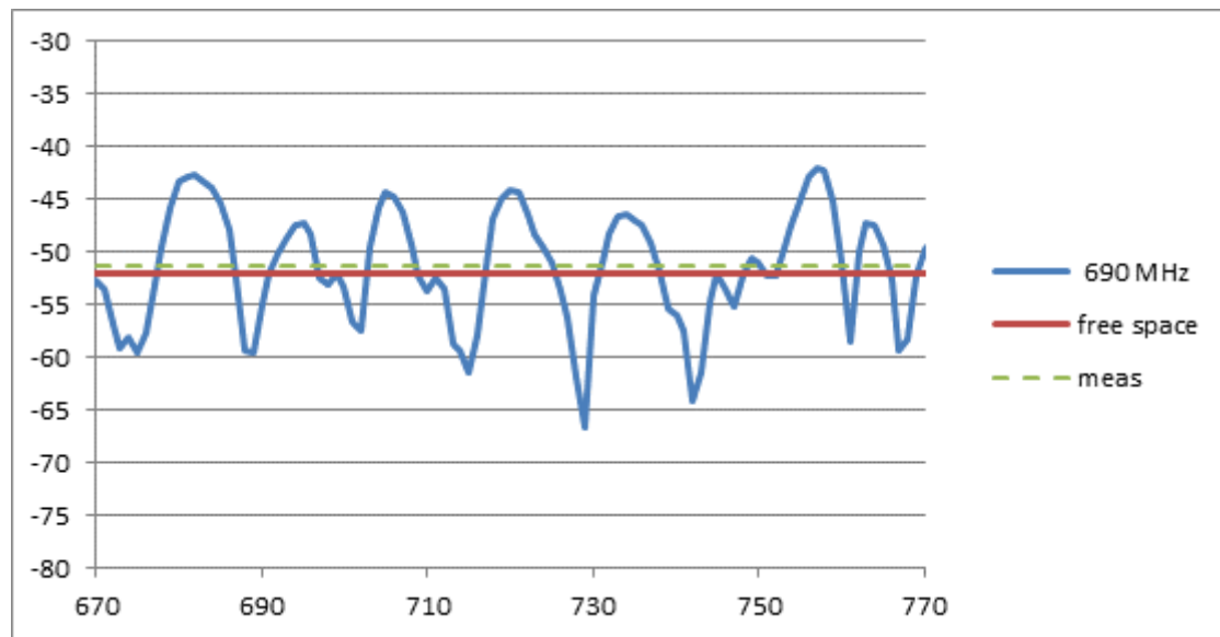
FIGURE 106 Balcony reference measurement (floor 3)
