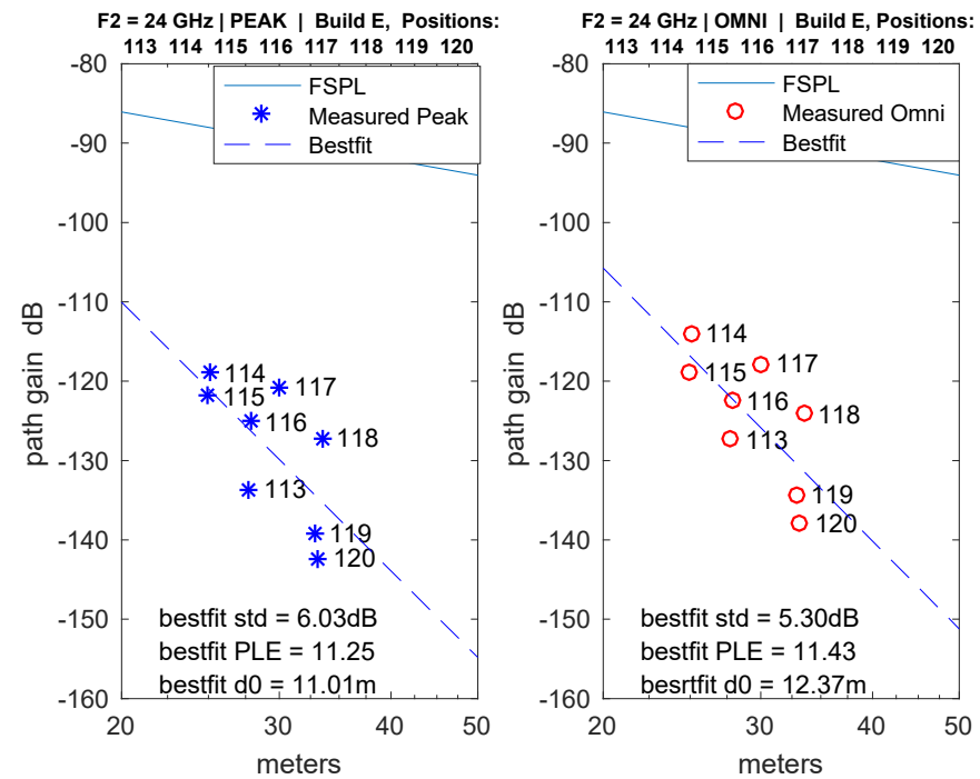
Example measurements on Tx2 signal
