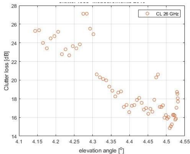
FIGURE 352 Clutter loss from 2019 measurements
