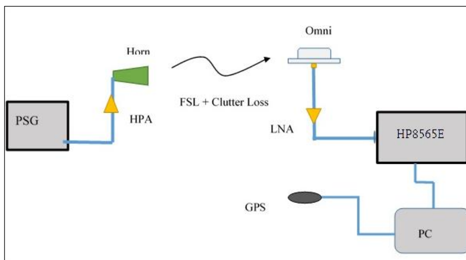
Measurement set up
