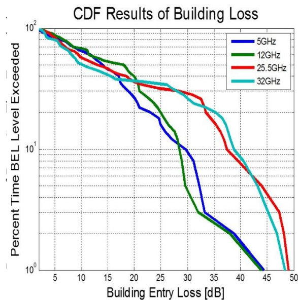
CDF of building entry loss for Building 2
