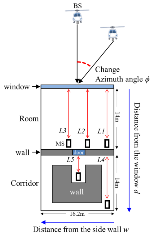
(b) Change of azimuth angle and MS position
