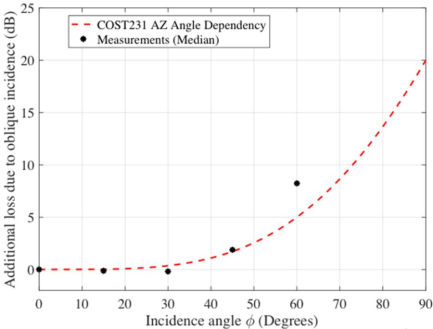
FIGURE 300 Incidence angle dependency
