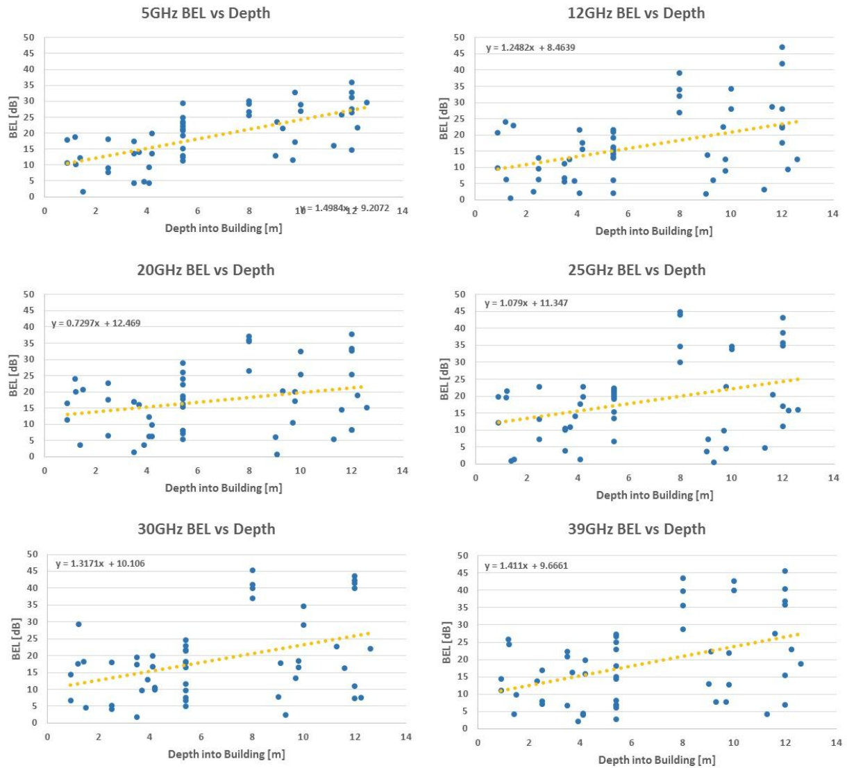
FIGURE 195 BEL vs depth for building 4
