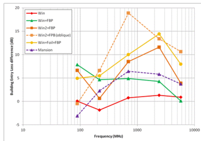
FIGURE 13 Increase in BEL compared to baseline configuration
