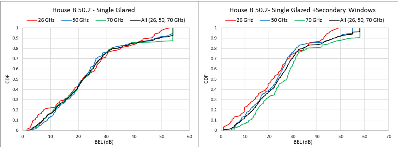
FIGURE 182 BEL CDFs for house B 50.2 with single glazed and single glazed plus secondary windows
