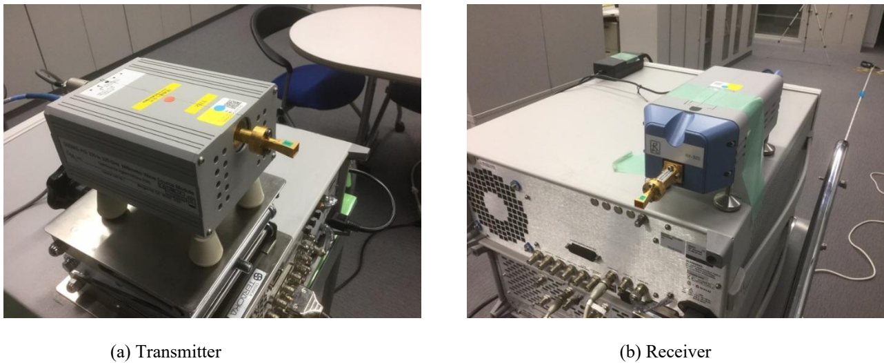
FIGURE 361 Measurement system
