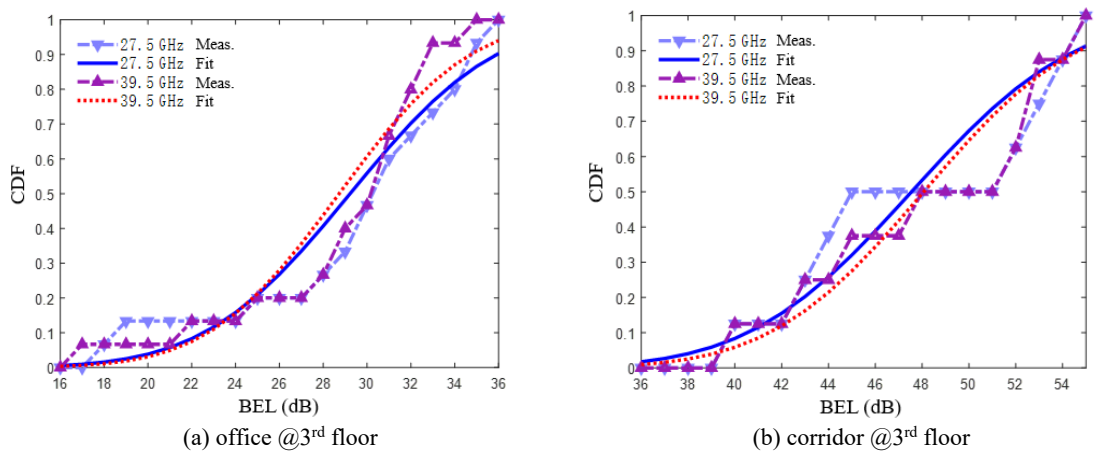
FIGURE 294 CDF distribution of measured BEL in urban environments
