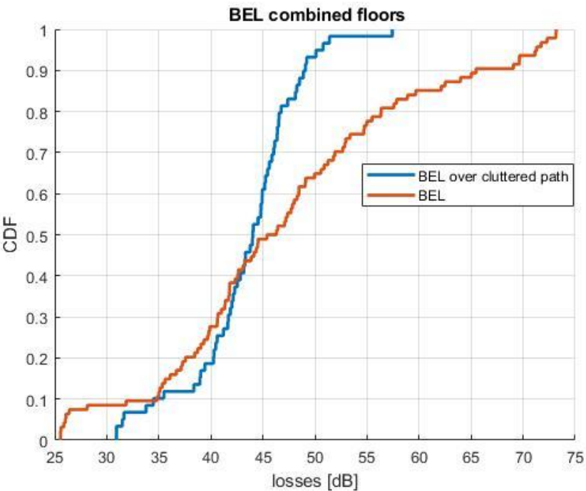
FIGURE 351 BEL estimated from Tx1(clutter) and Tx2 (BEL)
