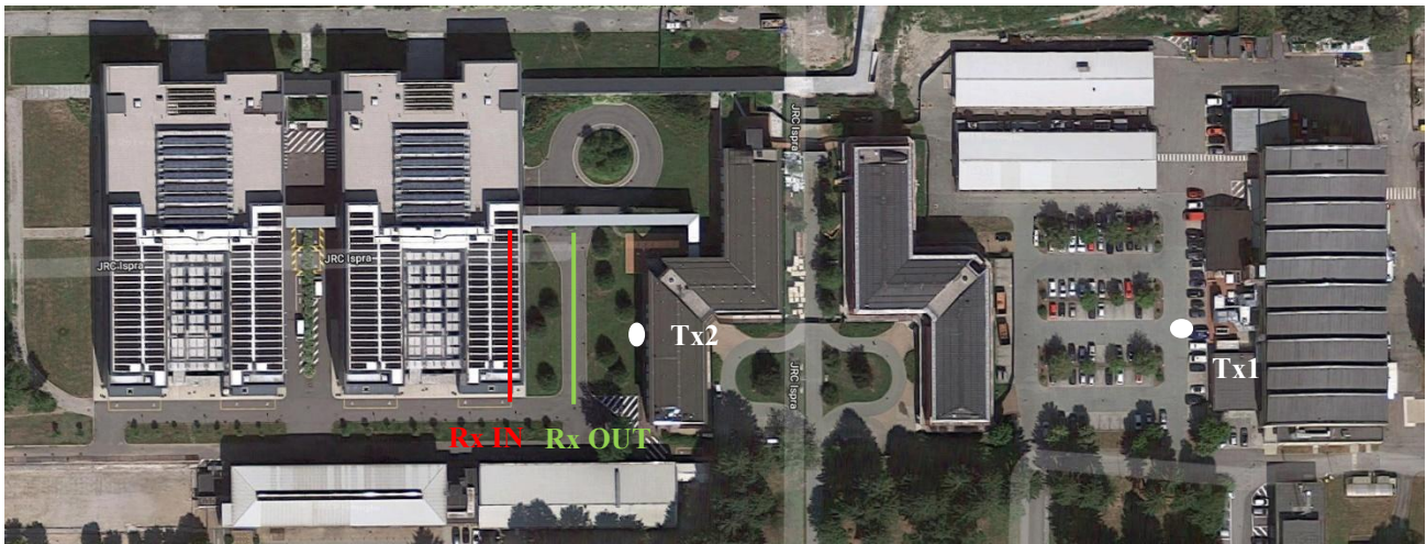
FIGURE 339 Measurement scenario
