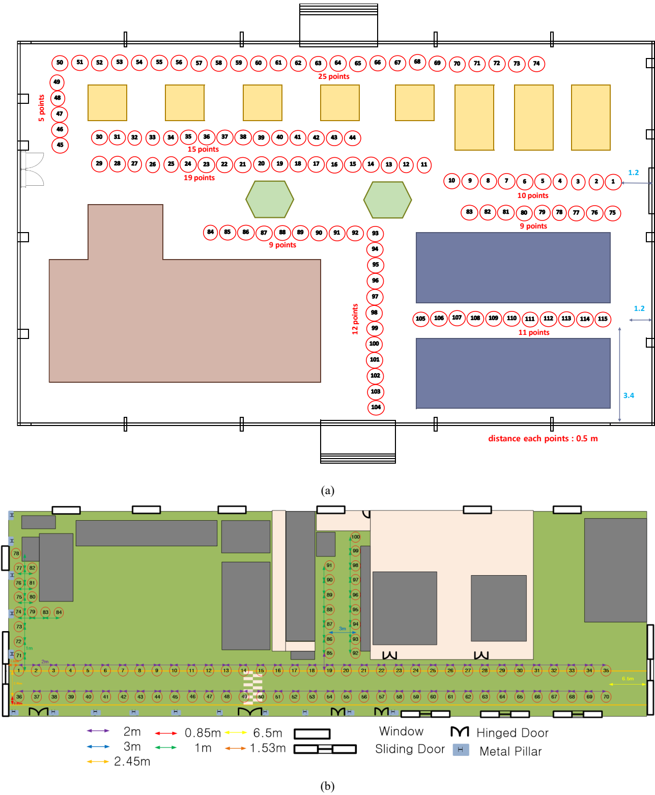
Floor plans and building entry loss measurement points for Factory A (a) and Factory B (b)
