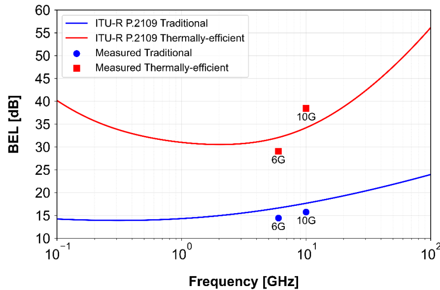
Comparison of measured median building entry loss with Recommendation ITU-R P.2109-2
