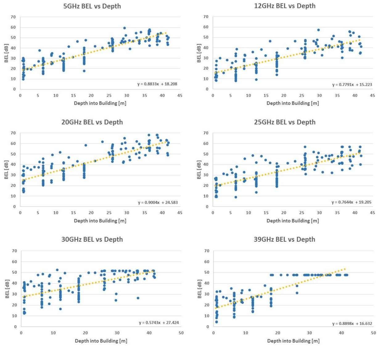
FIGURE 194 BEL vs depth for building 3
