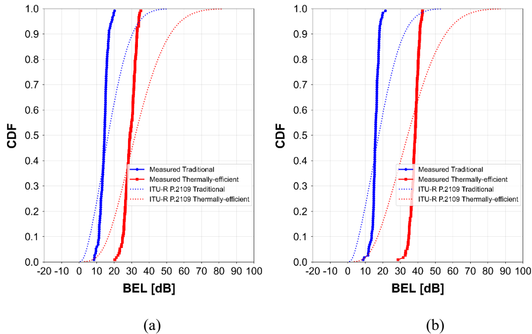
CDF characteristics of measured BEL values: (a) 6 GHz and (b) 10 GHz
