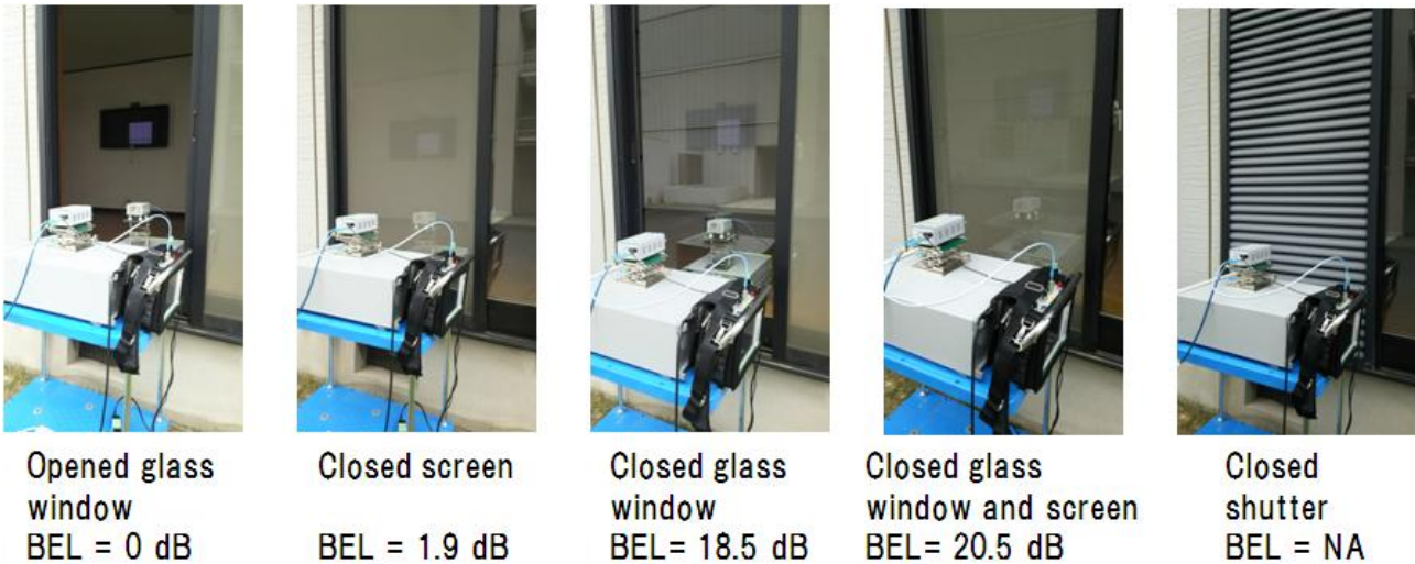
FIGURE 369 BEL measurement for a glass window (5 mm thickness), blind and shutter
