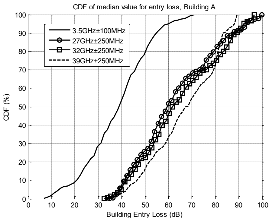
FIGURE 171 CDF of median value for entry loss, building A
