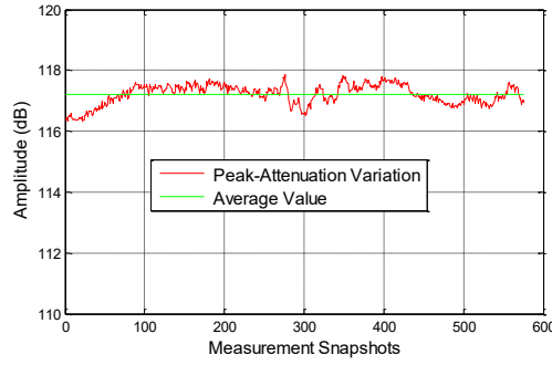
FIGURE 75 Peak-Attenuation Variation at 17 GHz (Dir.) for A5
