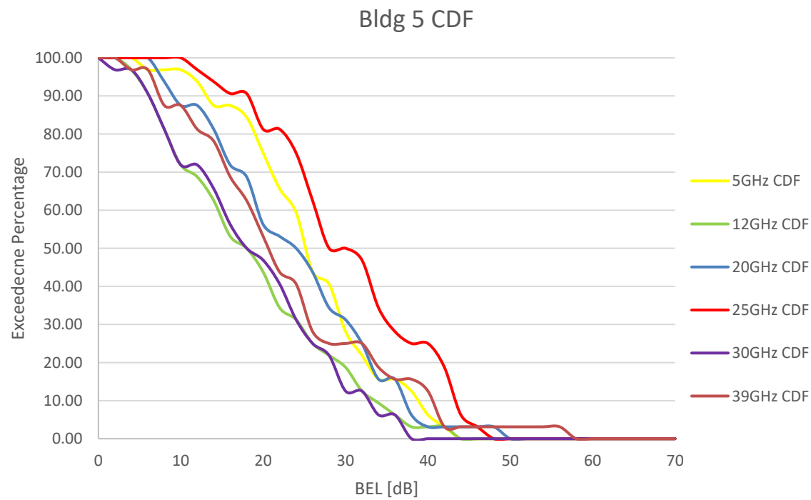
FIGURE 206 BEL CDFs for building 5
