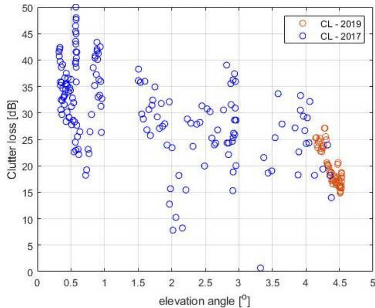
Clutter loss measurements 2019 and 2017
