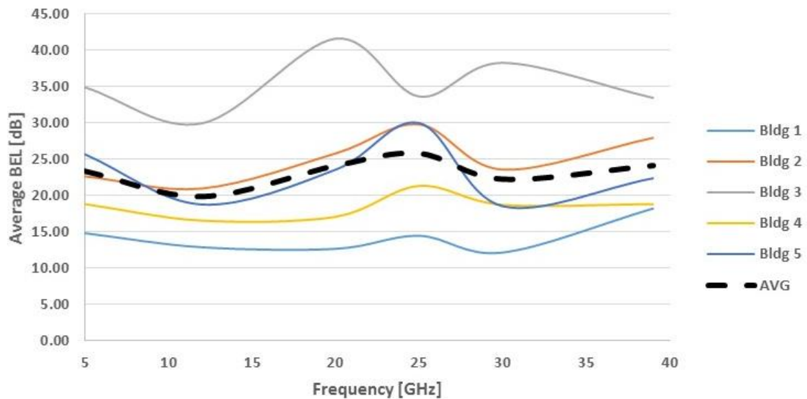
FIGURE 207 Frequency dependence of BEL
