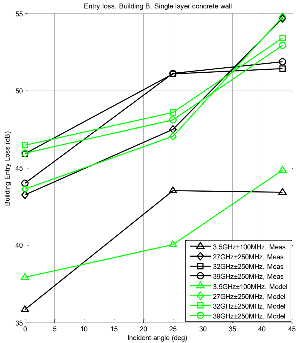
FIGURE 224 Entry loss, Building B, Single layer concrete wall
