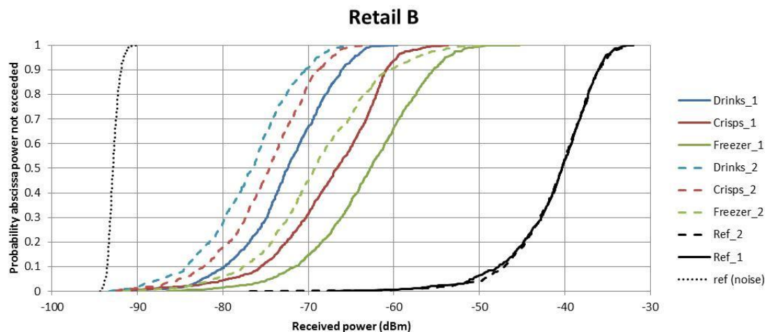
Summary results for 'Retail B' measurements
