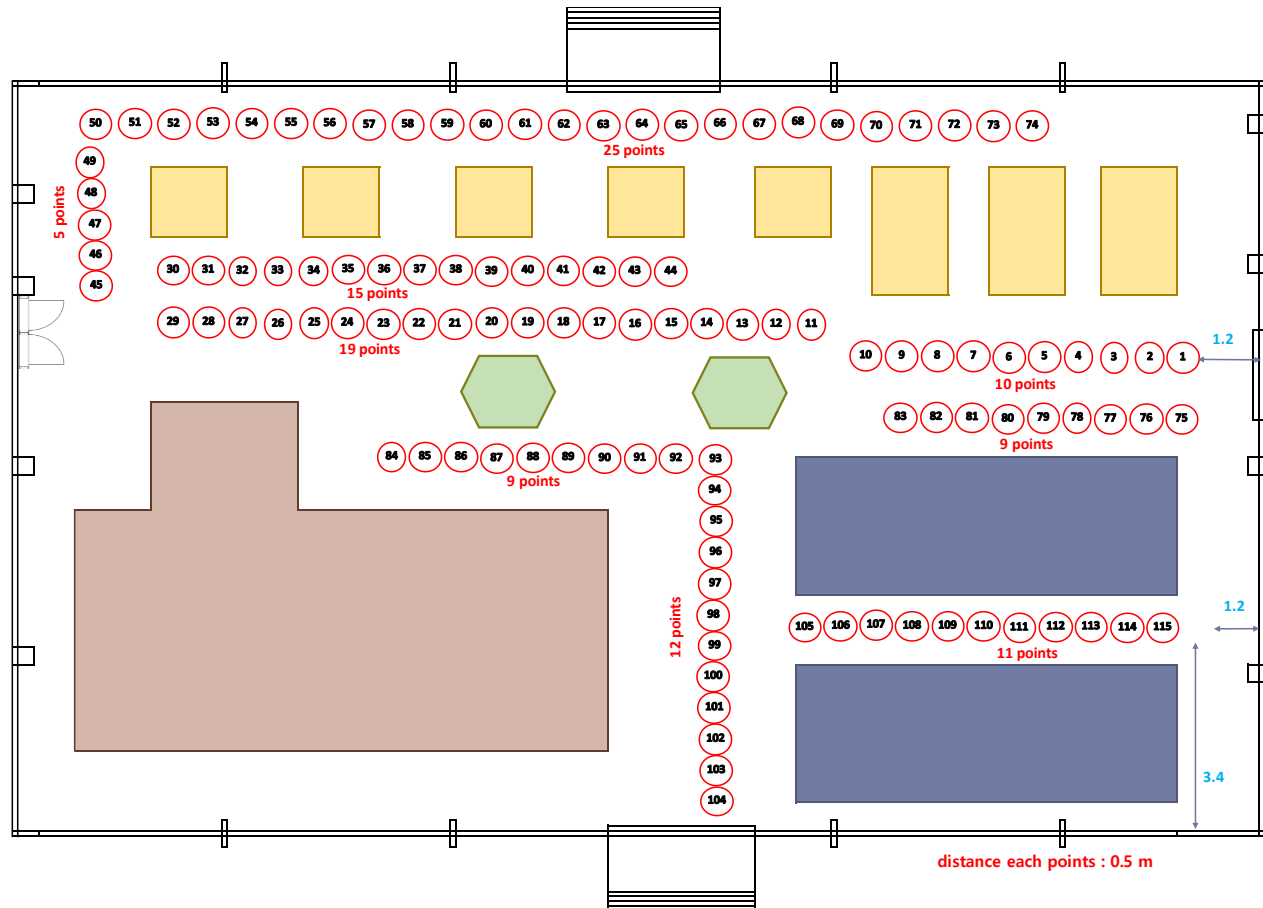
Factory floor plan and building entry loss measurement points of the receiver
