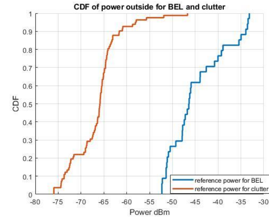
FIGURE 348 CDF of received power outside the building from Tx1 (over cluttered path) and Tx2 (BEL)
