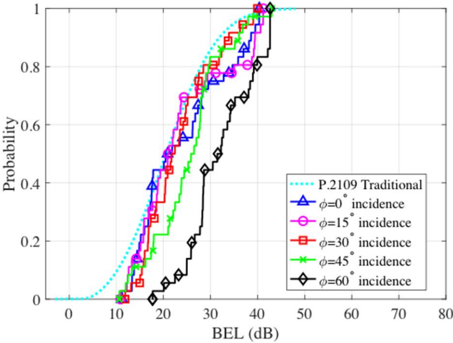
FIGURE 299 CDF of BEL measurement
