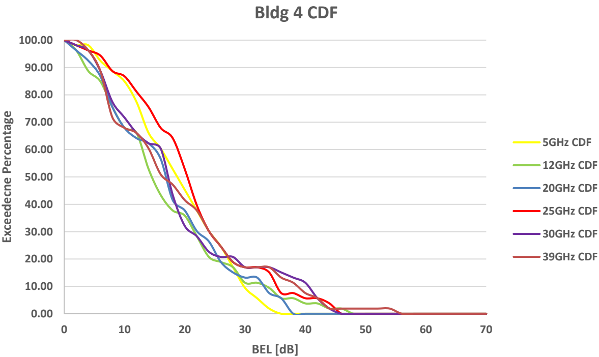
FIGURE 205 BEL CDFs for building 4
