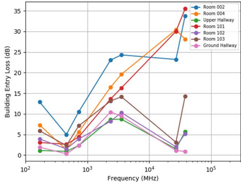
FIGURE 268 BEL for all rooms in Mansion at normal incidence
