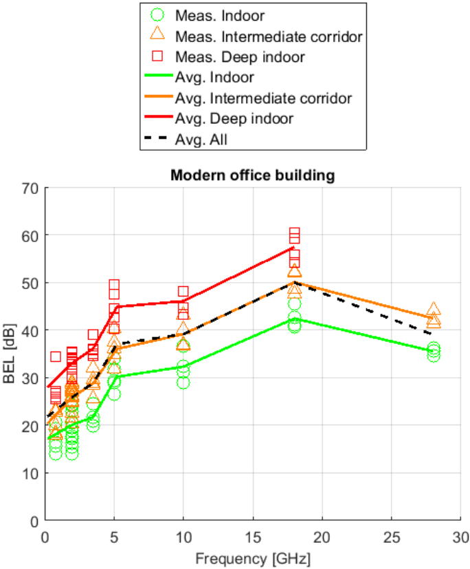
FIGURE 178 BEL measurement results for the modern office building
