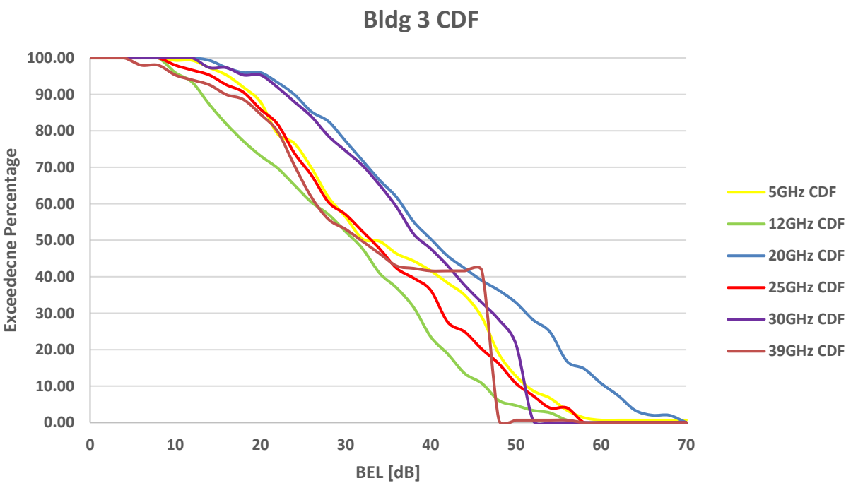
FIGURE 204 BEL CDFs for building 3
