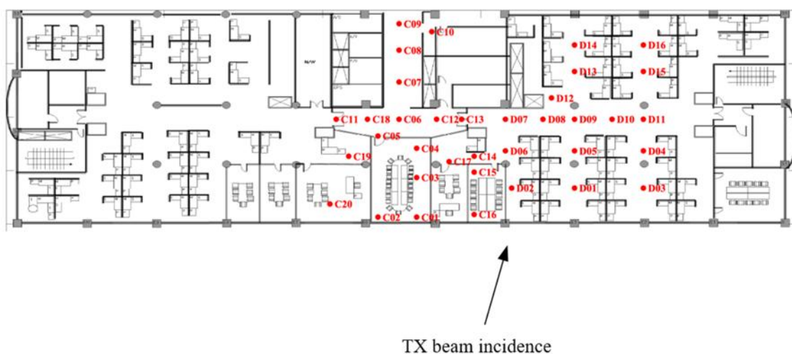
FIGURE 298 BEL measurement setup (planar view)
