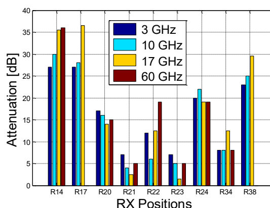
FIGURE 152 Building entry losses across the four bands
