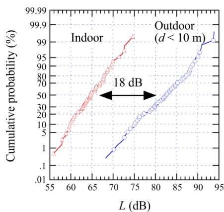
FIGURE 4 Cumulative probabilities of measured path loss data
