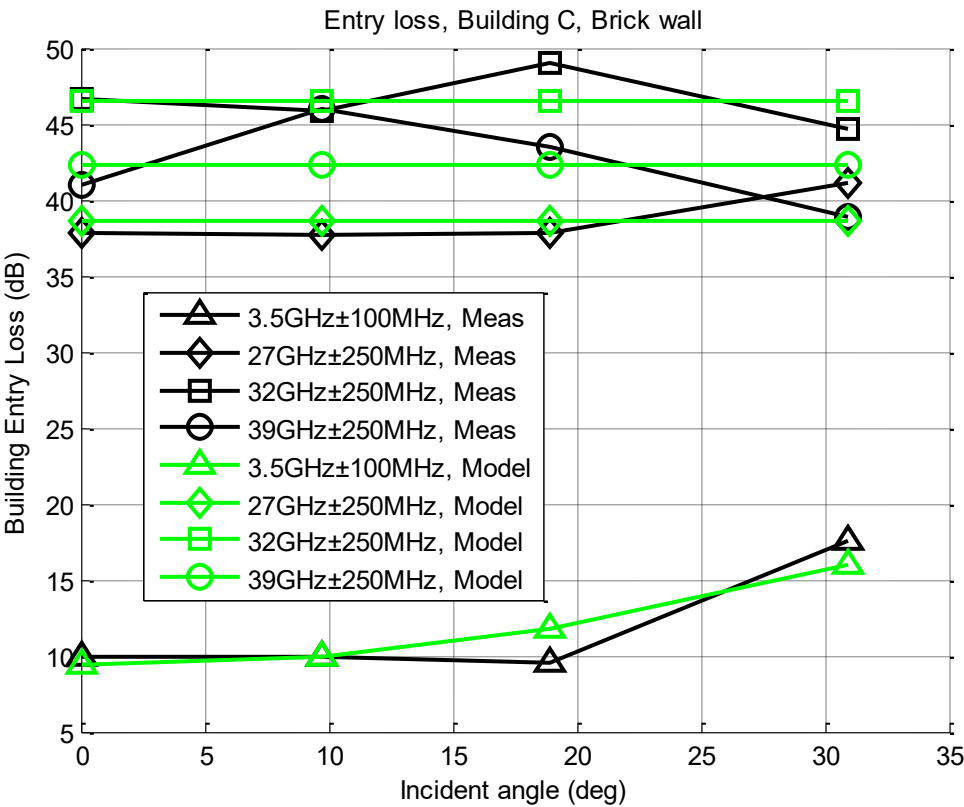
Entry loss, Building C, Brick wall
