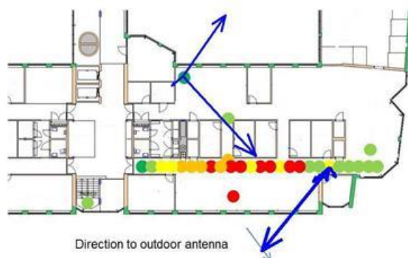
FIGURE 48 Attenuation in scenario two, with wide-beam antenna at the outdoor site (See Table 24 for colour legend)
