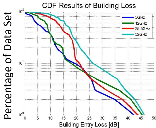
CDF of building entry loss for Building 1
