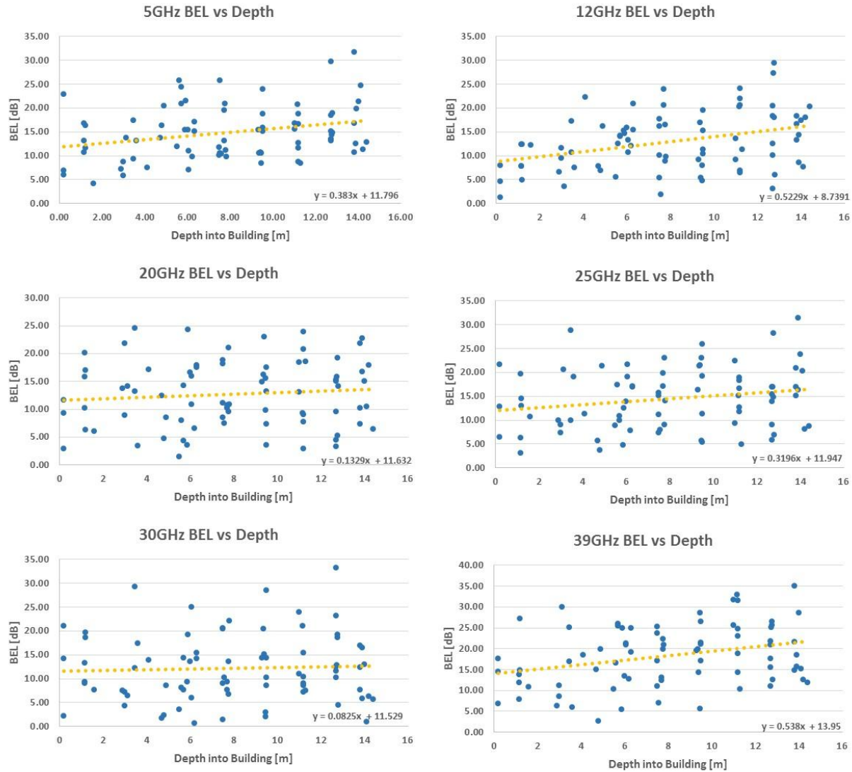
FIGURE 192 BEL vs depth for building 1
