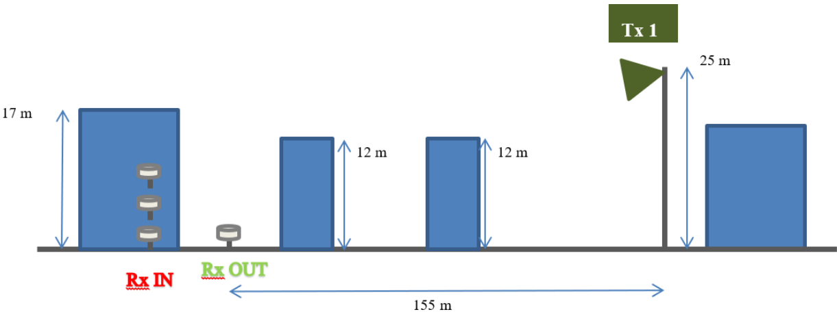
FIGURE 343 Scenario side view
