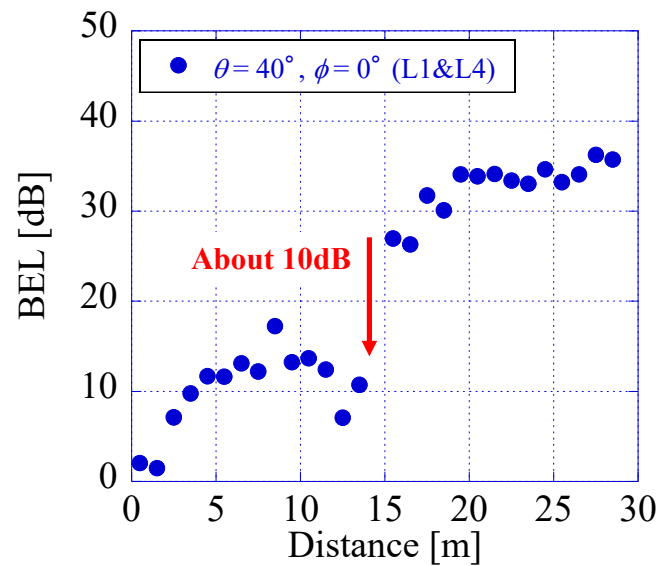
FIGURE 375 Measurement result showing the effects through the wall
