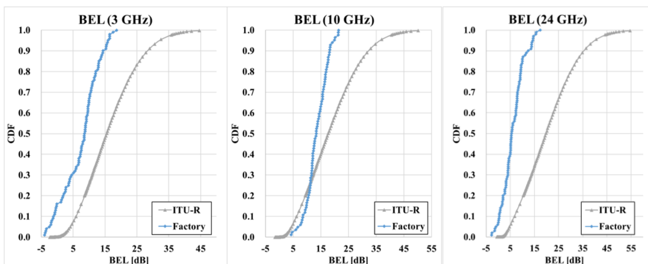
FIGURE 383 CDF characteristics of the building entry loss in terms of frequency for Factory B
