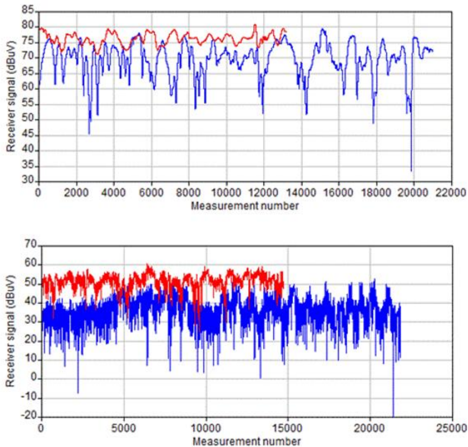
FIGURE 11 Measurements made indoors (blue) and outdoors (red) – see text
