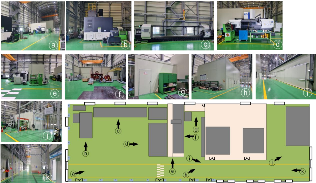
FIGURE 380 Interior images from various points for Factory B
