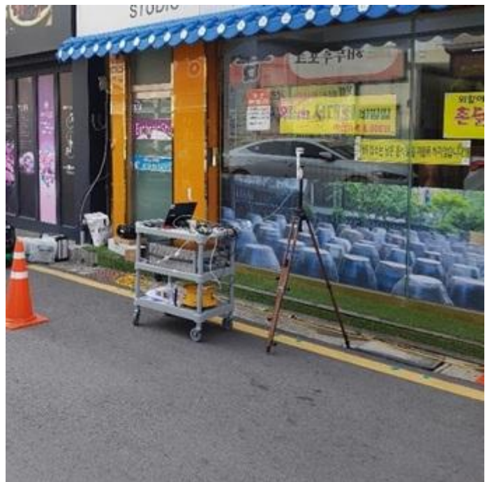
FIGURE 333 Configuration of measurement equipment (a) Transmitter (b) Receiver
