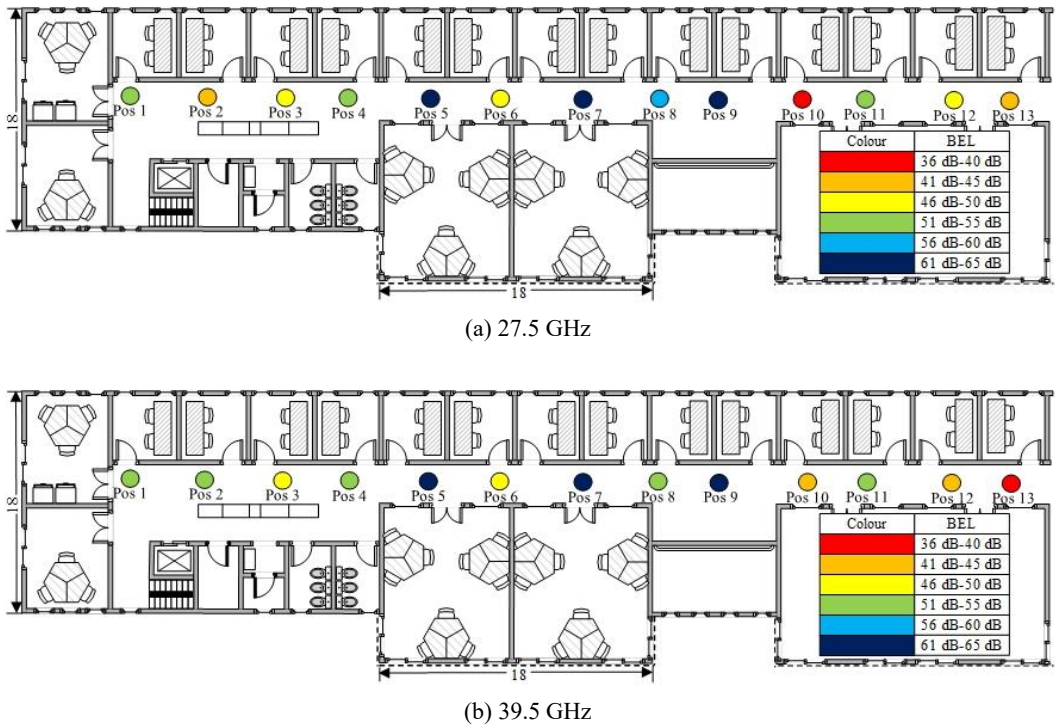
FIGURE 293 BEL for omni-directional channel in corridor environment at 4 th floor
