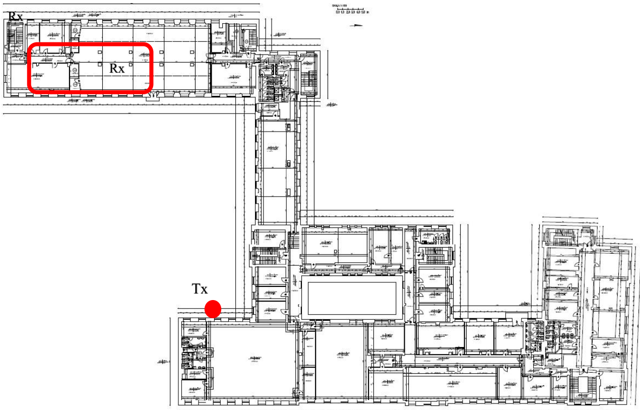
Top view of Orange facility with Tx and Rx locations
