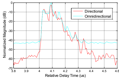
FIGURE 76 PDP (Dir. Vs Omni.) 17 GHz for R24
