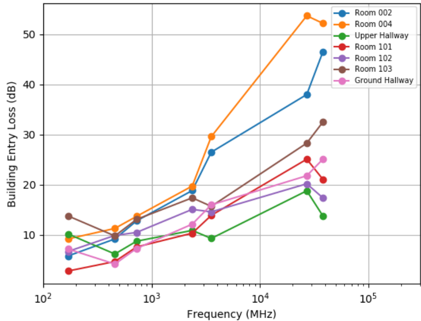
FIGURE 269 BEL for all rooms in Mansion at 45-degree incidence
