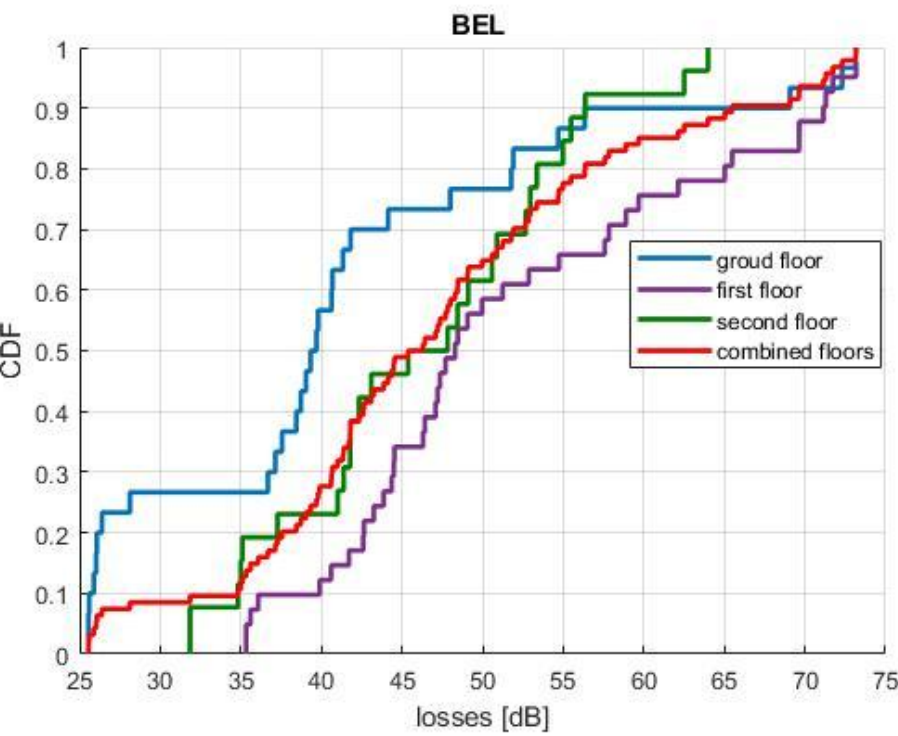
FIGURE 349 BEL estimated from Tx2
