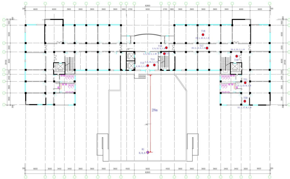
FIGURE 86 The transmitting points indoor and the receiving points outdoor on the fourth floor, the length of the platform is 28 m
