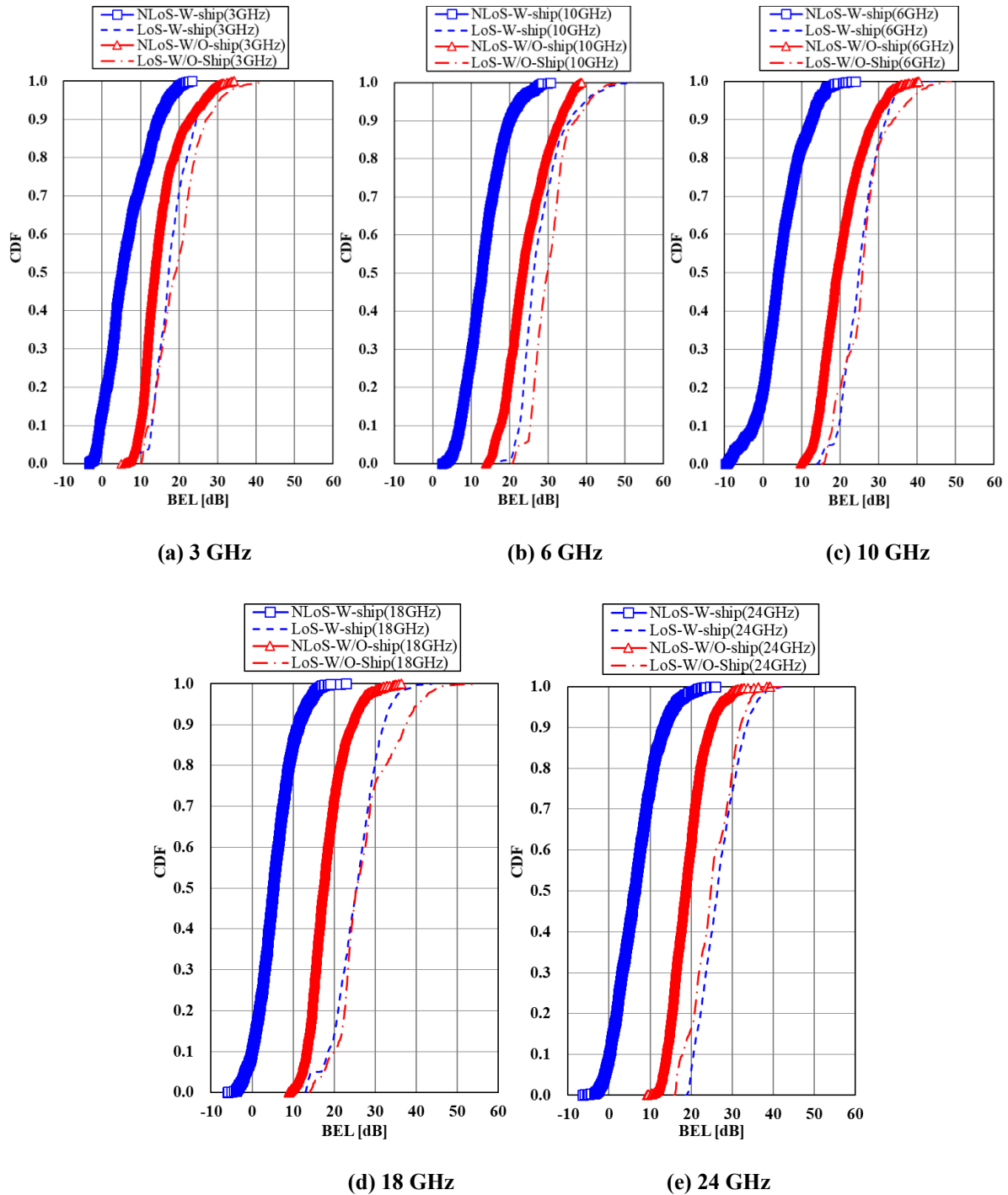
CDF characteristics of measured BEL values at 3-24 GHz
