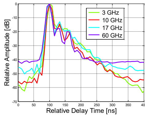
FIGURE 153 PDPs at 3, 10, 17 and 60 GHz at location 25
