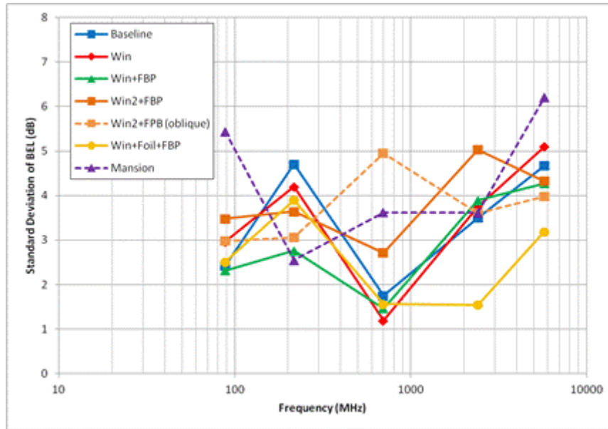
FIGURE 12 Room to room standard deviation of building entry loss
