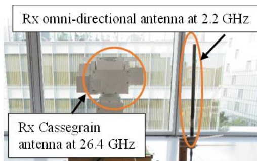
(b) Rx antenna setup at 2 and 26 GHz
