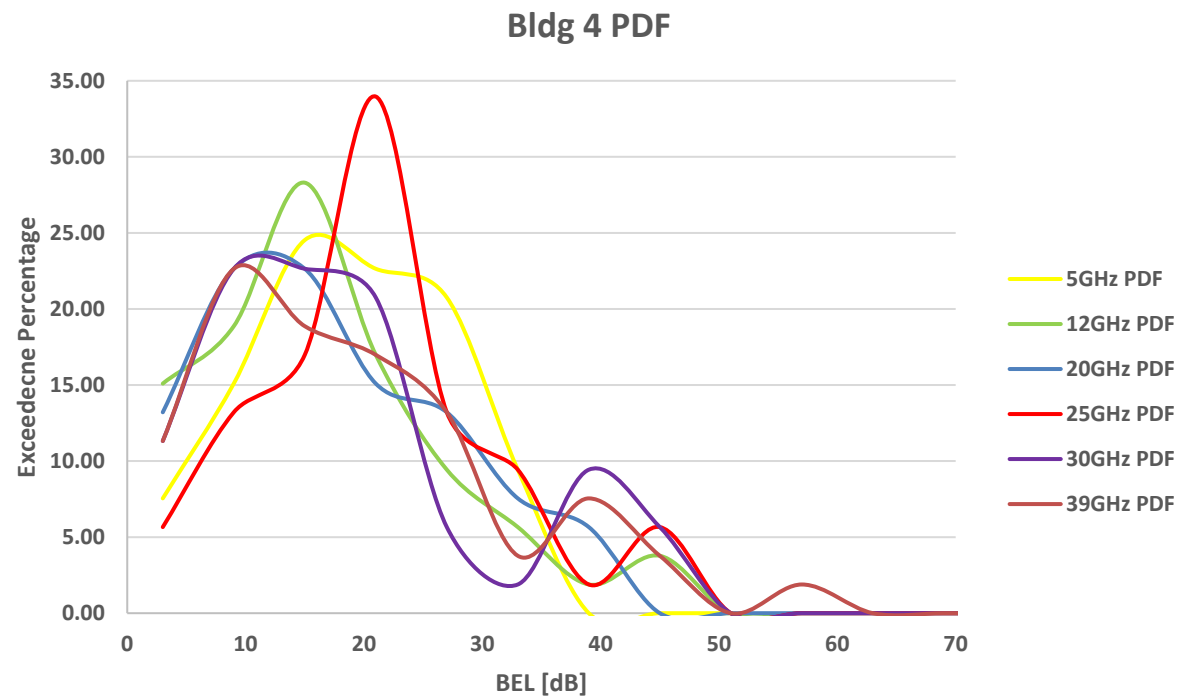
FIGURE 200 BEL PDFs for building 4
