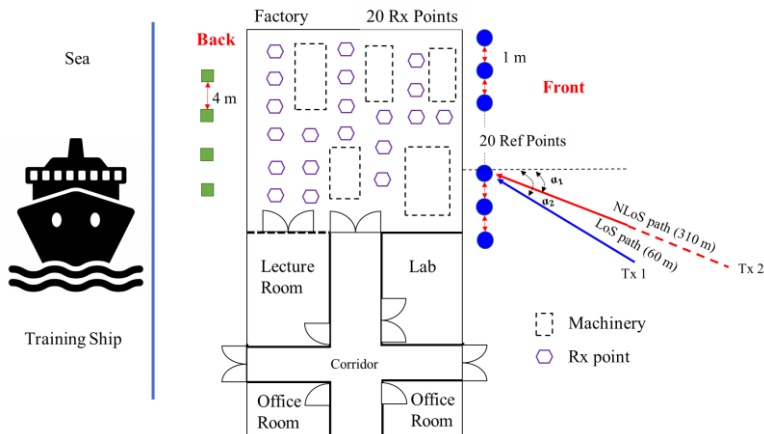
FIGURE 325 Outdoor and indoor measurement scenarios for two paths
