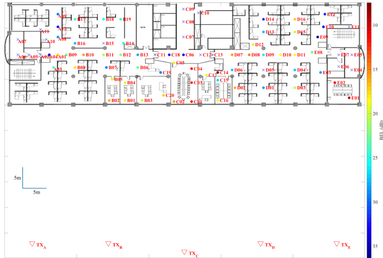
FIGURE 257 Omnidirectional BEL measurements in Building A
