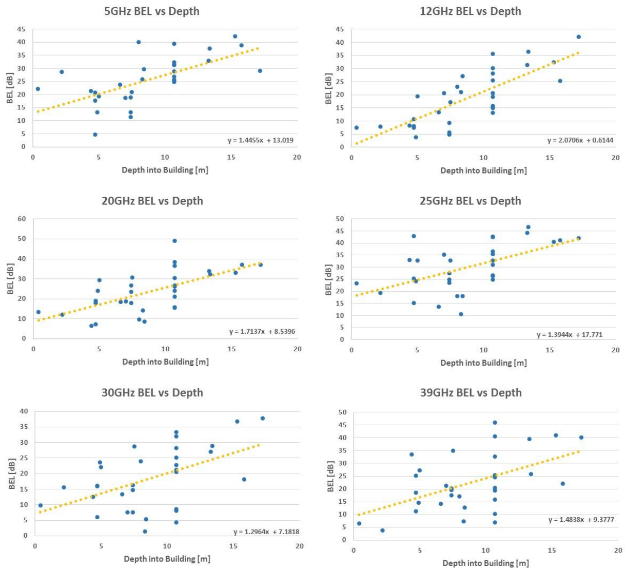
FIGURE 196 BEL vs depth for building 5
