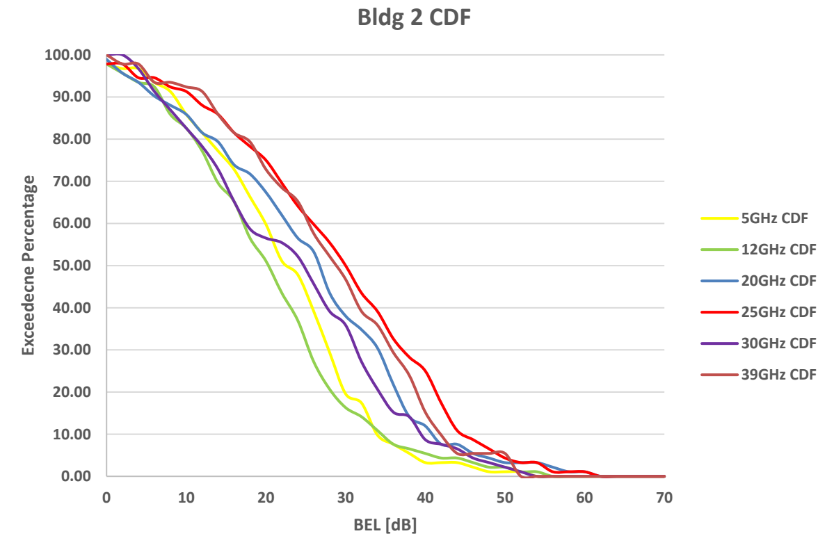
FIGURE 203 BEL CDFs for building 2
