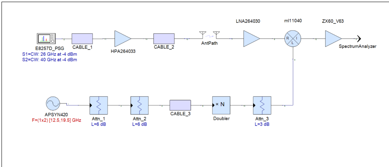
FIGURE 356 Experimental measurement setup
