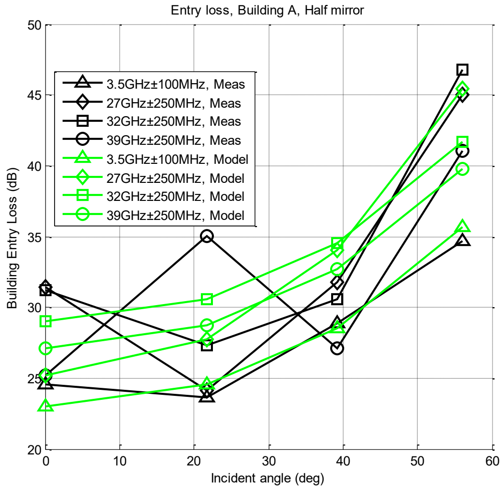
FIGURE 222 Entry loss, Building A, Half mirror
