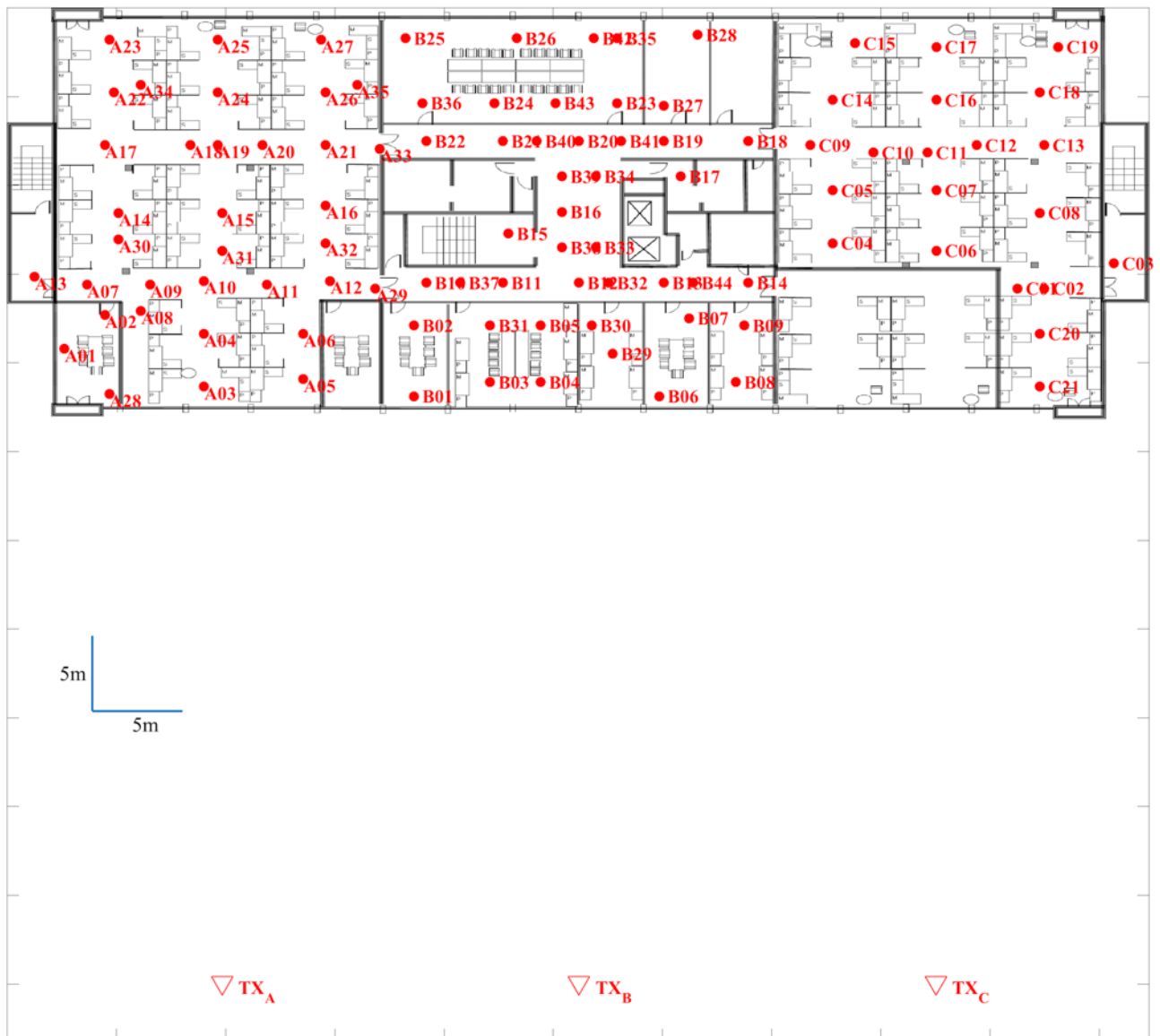
FIGURE 255 Measurement points for Building B
