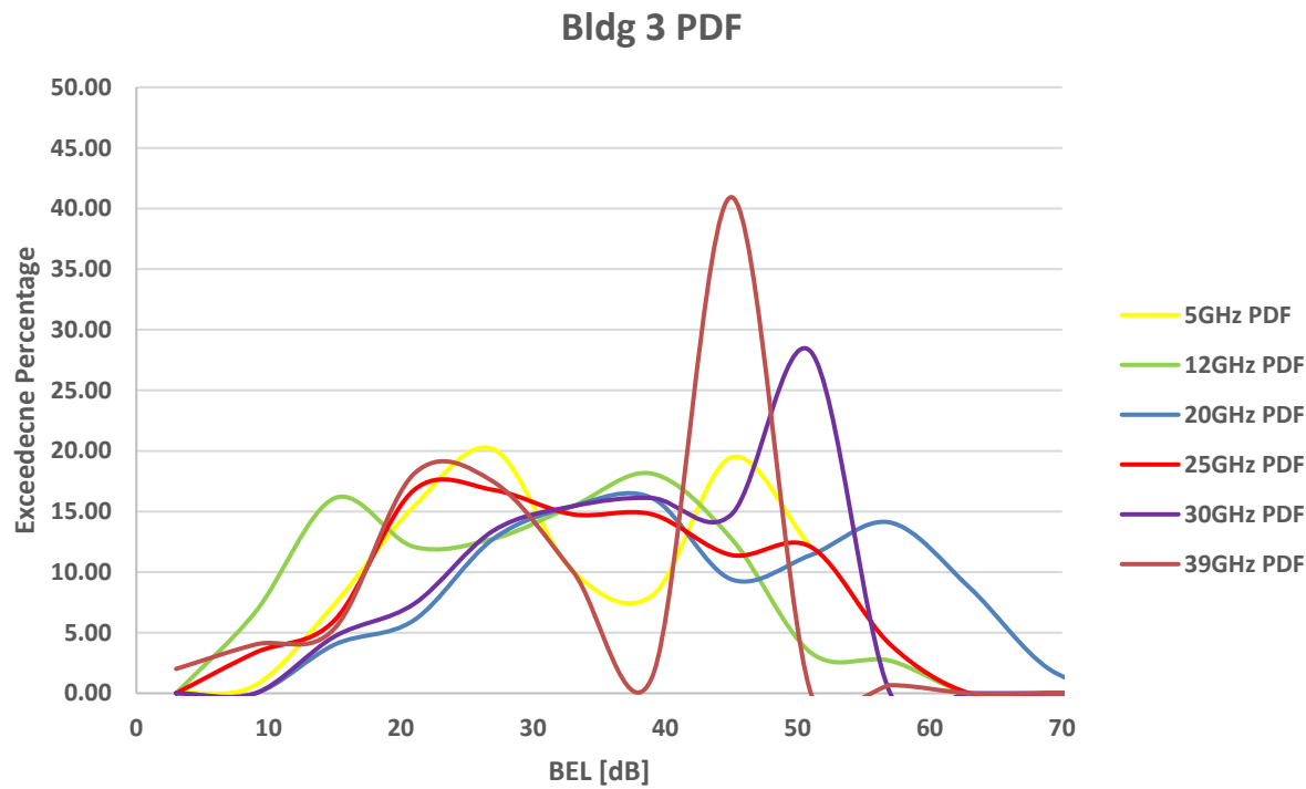
FIGURE 199 BEL PDFs for building 3
