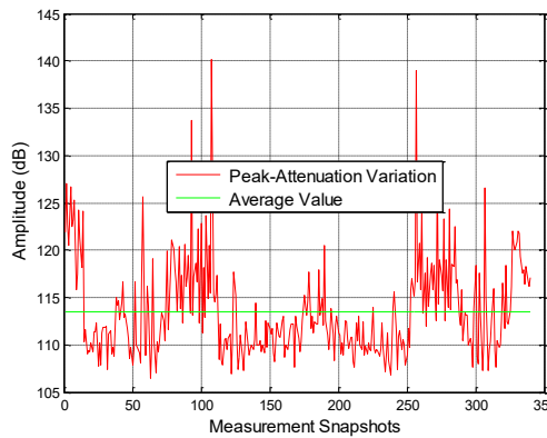
FIGURE 74 Peak-Attenuation Variation at 17 GHz (Omni.) for R32
