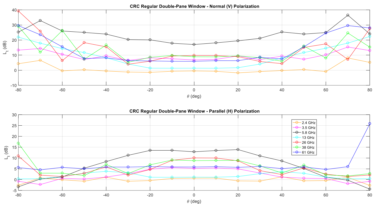
FIGURE 142 Transmission loss L_t as a function of incidence angle ( \theta ) for regular, double-pane window, similar to the ones found in CRC building 76 (Fig. 126)
