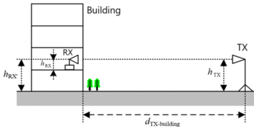
BEL measurement setup
