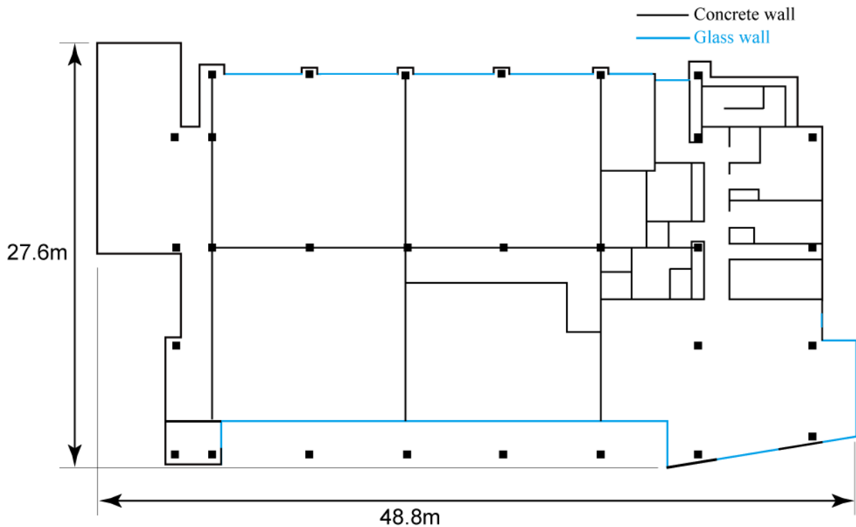
Ground floor plan of the light gauge steel building
