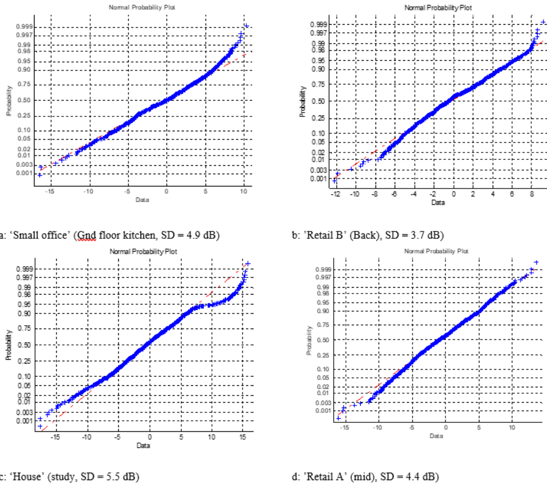
FIGURE 44 Sample loss distributions
