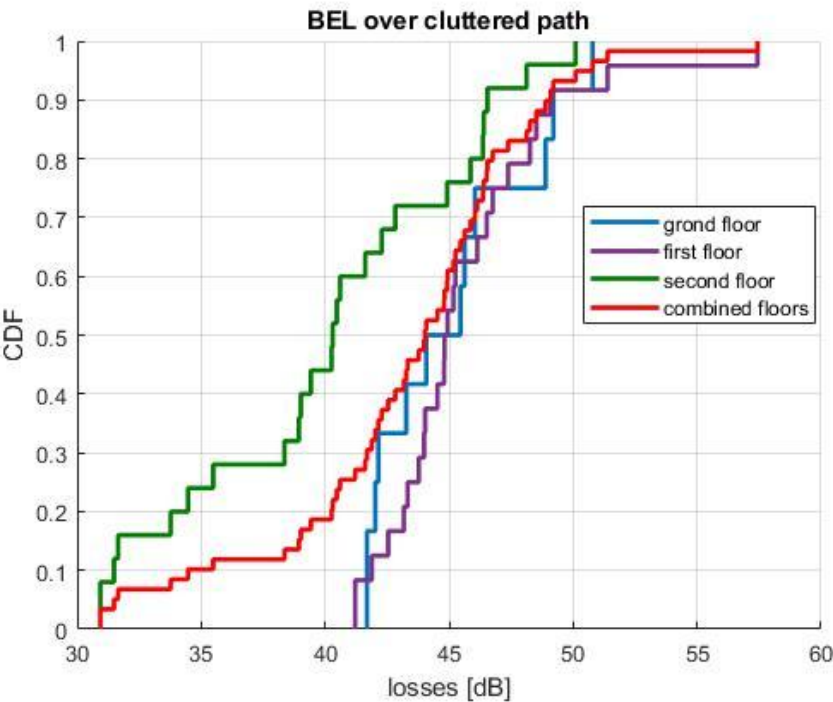
FIGURE 350 BEL estimated from Tx1 (over cluttered path)
