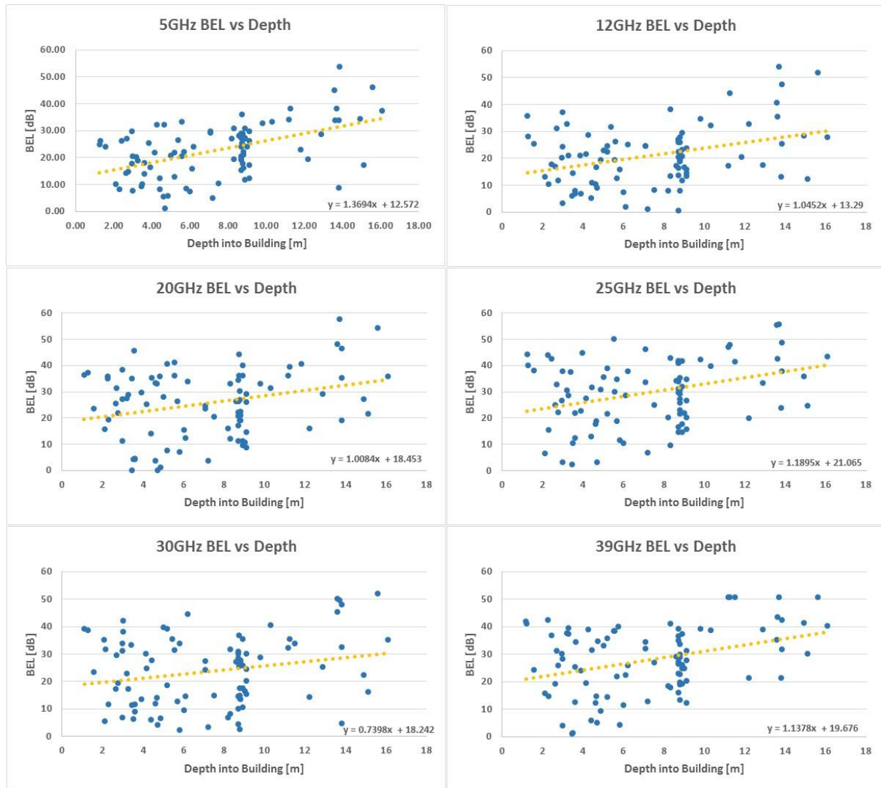
FIGURE 193 BEL vs depth for building 2
