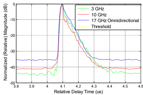
FIGURE 80 Relative PDPs across the frequency bands for R33
