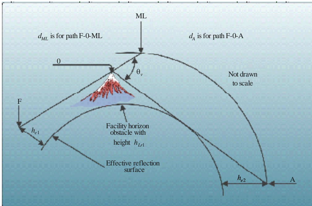
FIGURE 8 Paths used to determine diffraction attenuation
