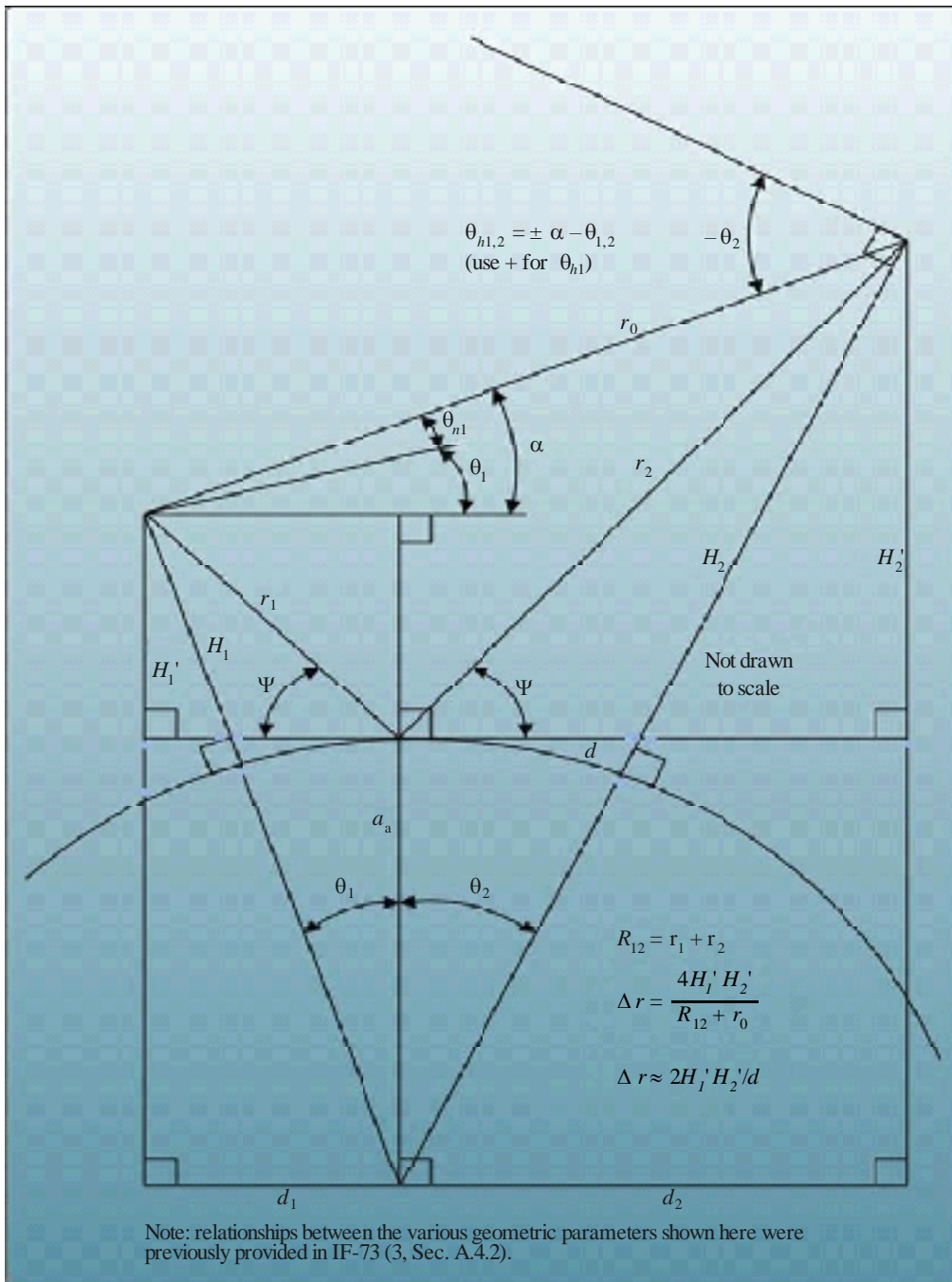
FIGURE 9 Spherical earth with two ray path geometry
