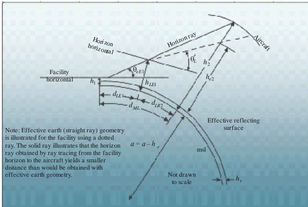
FIGURE 5 Facility radio horizon geometry
