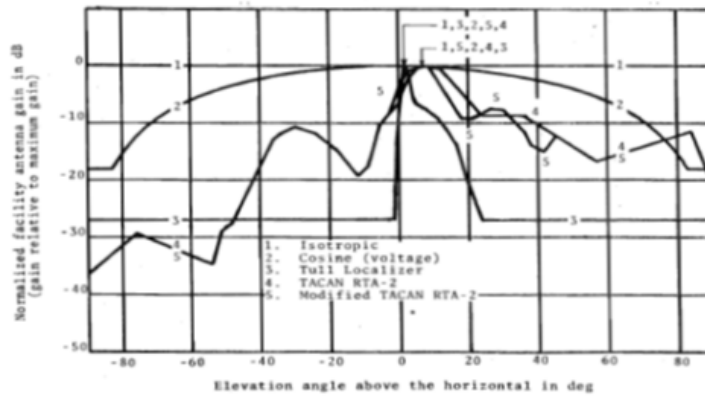
FIGURE 11 Normalized antenna gain vs. elevation angle [2]
