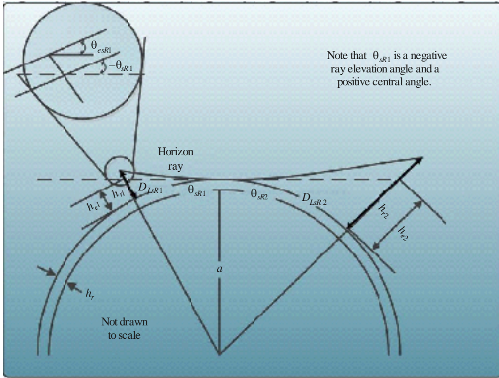
FIGURE 4 Effective height geometry
