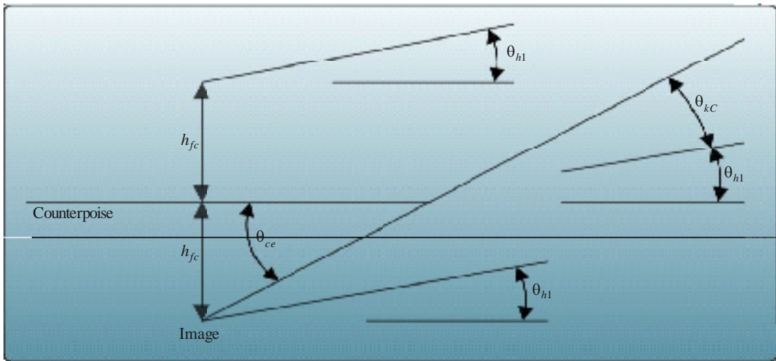
Geometry for earth reflection diffraction parameter, v_b , with limited surface of counterpoise
