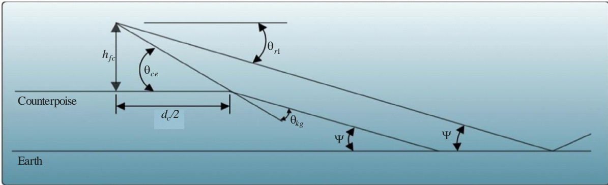
Geometry for earth reflection diffraction parameter, v_g , with counterpoise shadowing
