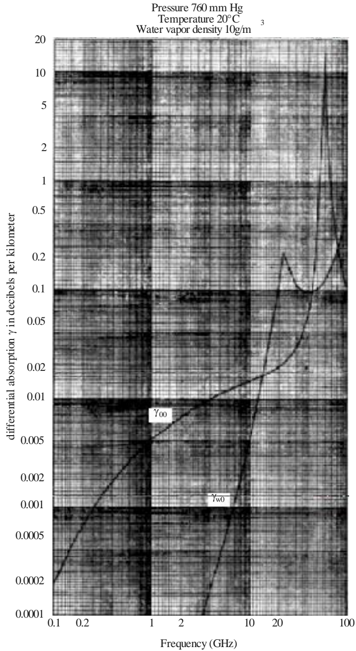
FIGURE 13 Surface values of atmospheric absorption by oxygen and water vapour [5]
