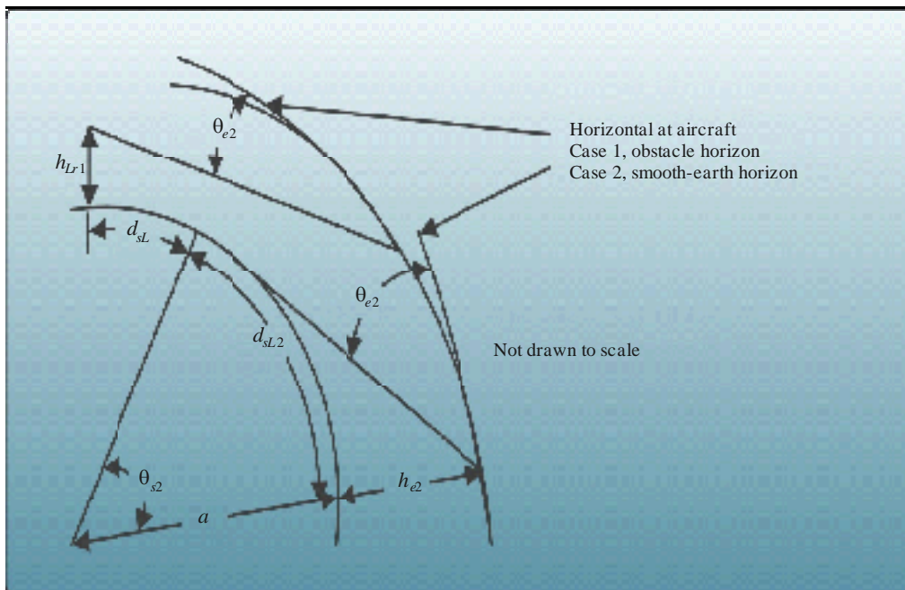
FIGURE 7 Geometry for the higher antenna radio horizon
