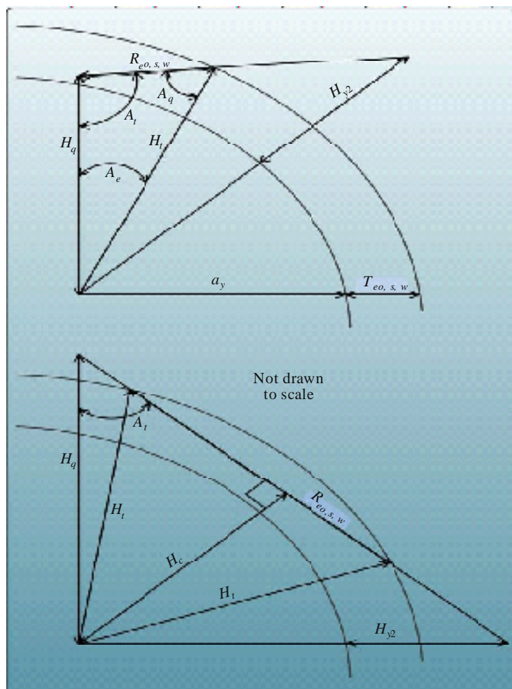
FIGURE 12 Geometry associated with atmospheric absorption
