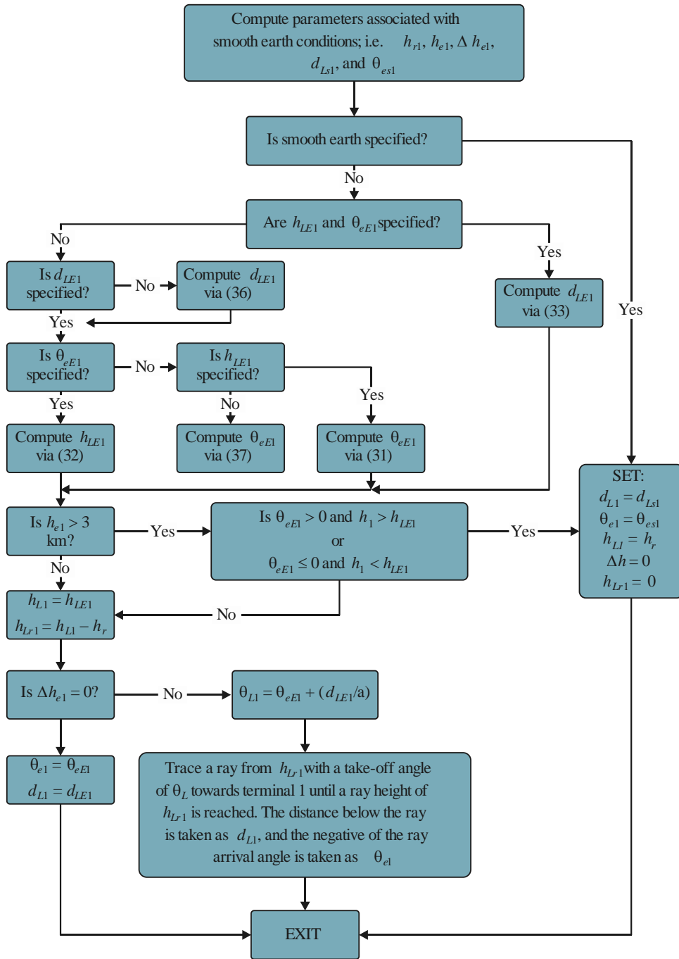
FIGURE 6 Logic flow to calculate facility horizon parameters
