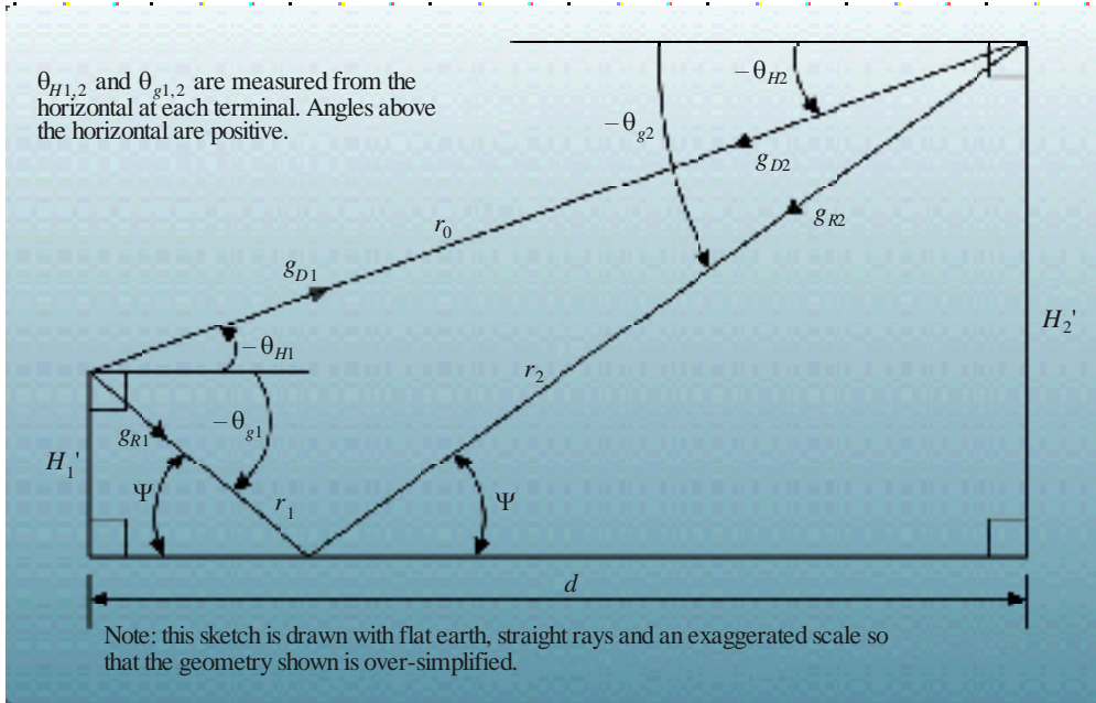
Antenna gain notation and correspondence between ray take-off angles and gains
