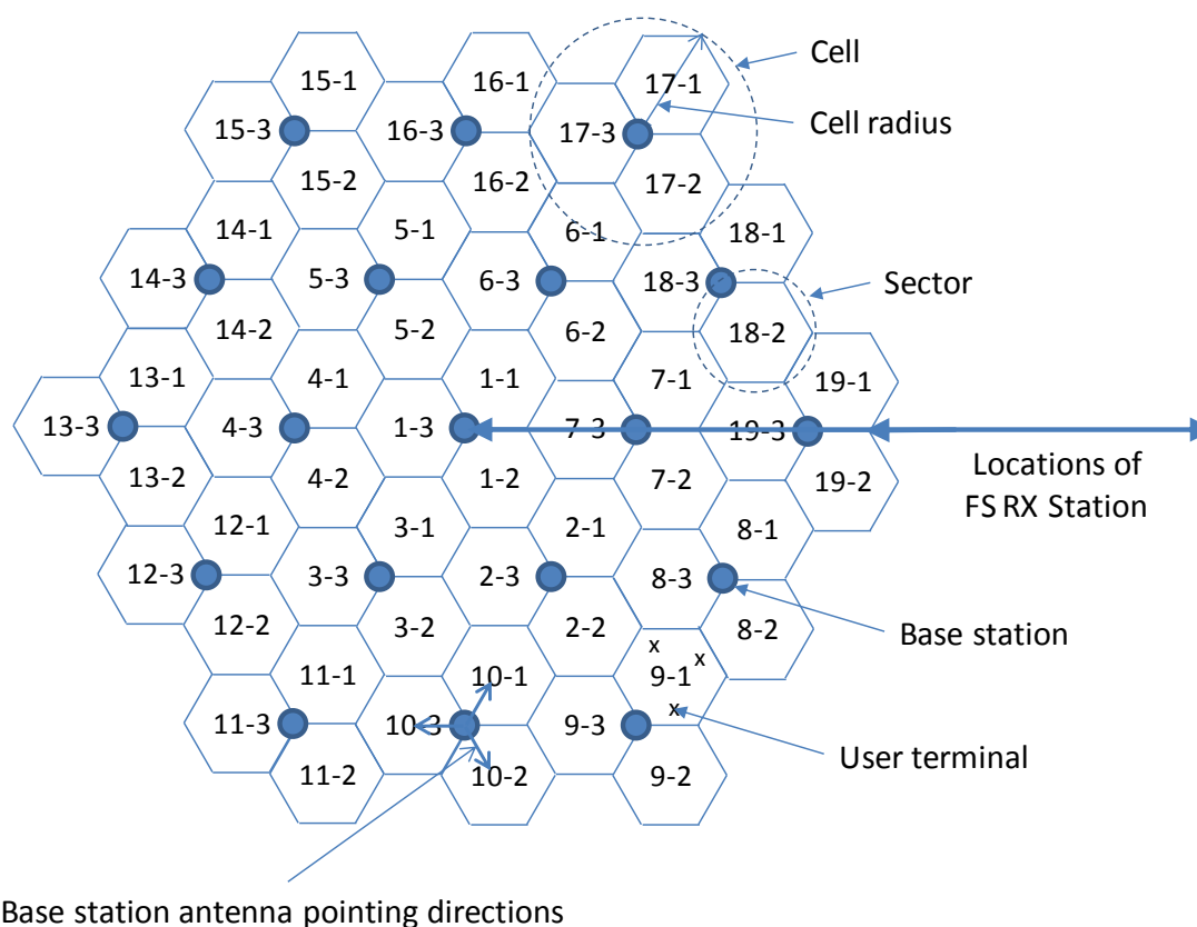
FIGURE 1 IMT Network Layout
