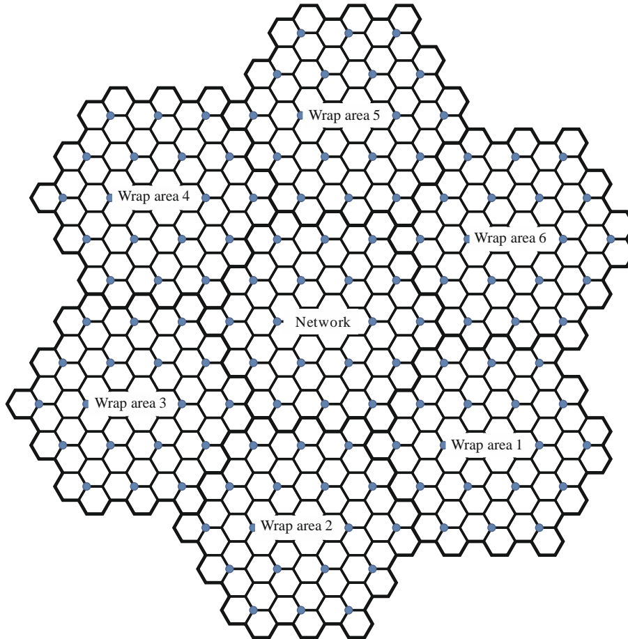
FIGURE 2 IMT network layout with “wrap-around” clusters
