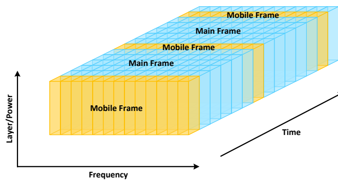
Frame structure of Time Division Multiplexing (TDM)
