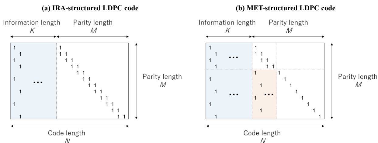
Parity-check matrix structure
