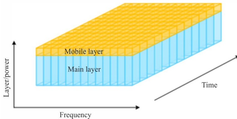
FIGURE 7 Frame structure of Layer Division Multiplexing (LDM)
