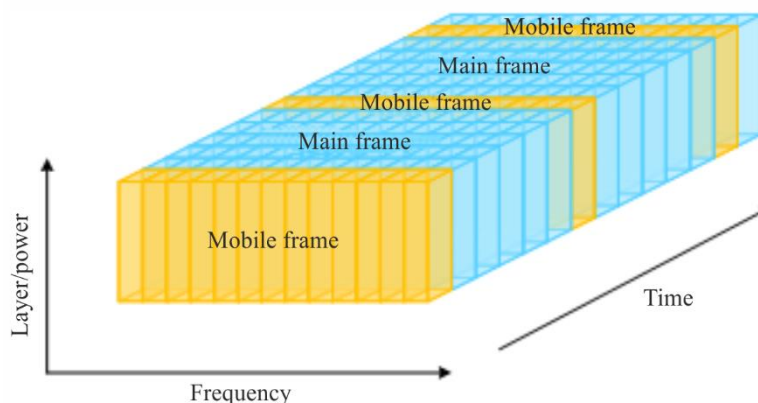
FIGURE 6 Frame structure of Time Division Multiplexing (TDM)
