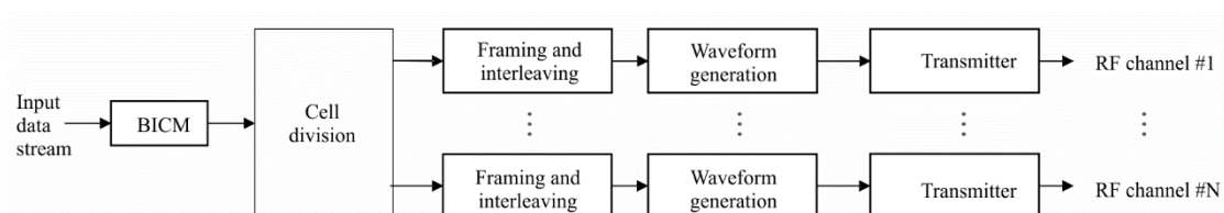
Block diagram of channel bonding without stream division
