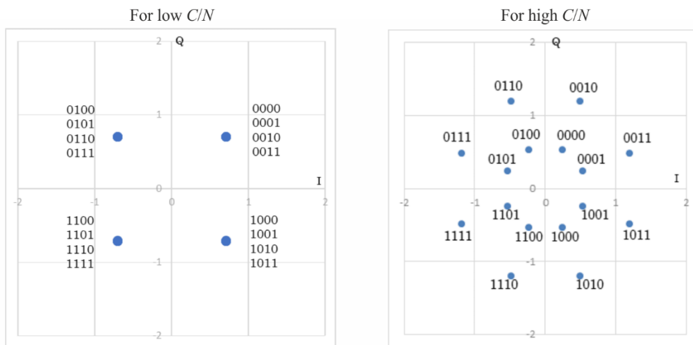
FIGURE 3 Non-Uniform Constellations (16 signal points) for different C/N
