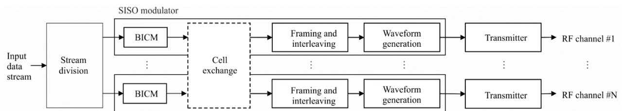
Block diagram of channel bonding with stream division
