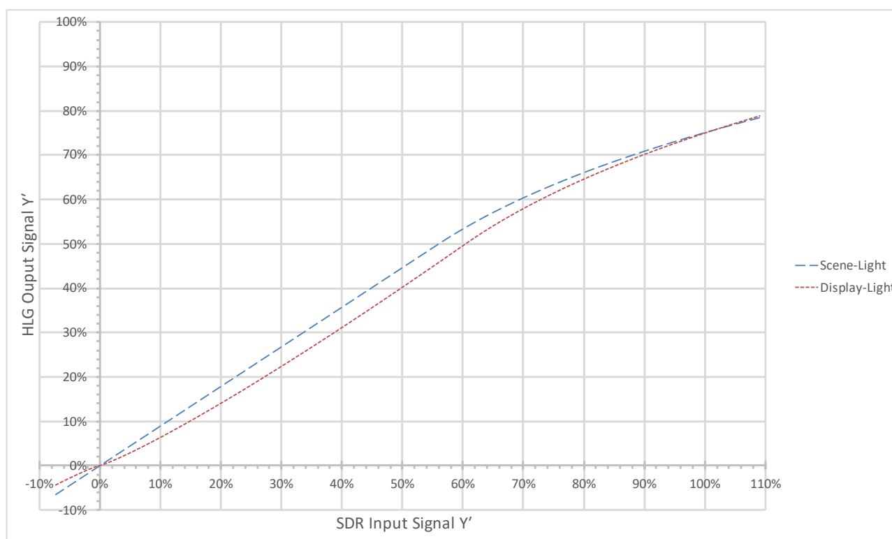
FIGURE 12 Comparison of scene-light and display-light direct-mapping
