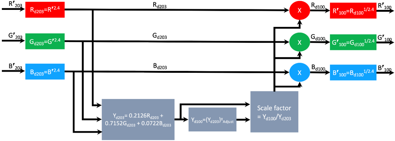
FIGURE A11-1 Conversion of 203 cd/m 2 SDR signals to 100 cd/m 2 SDR signals
