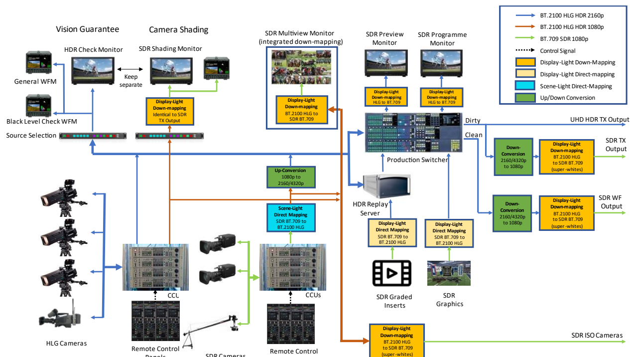
FIGURE 20 HDR production with camera shading in SDR
