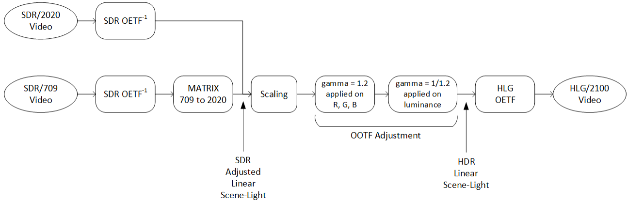
FIGURE 11 SDR to HLG mapping with gamma adjustment (scene-referred)
