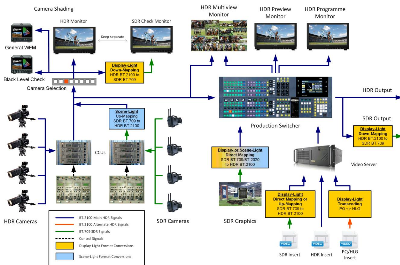
FIGURE 19 HDR production with SDR derived by down-mapping
