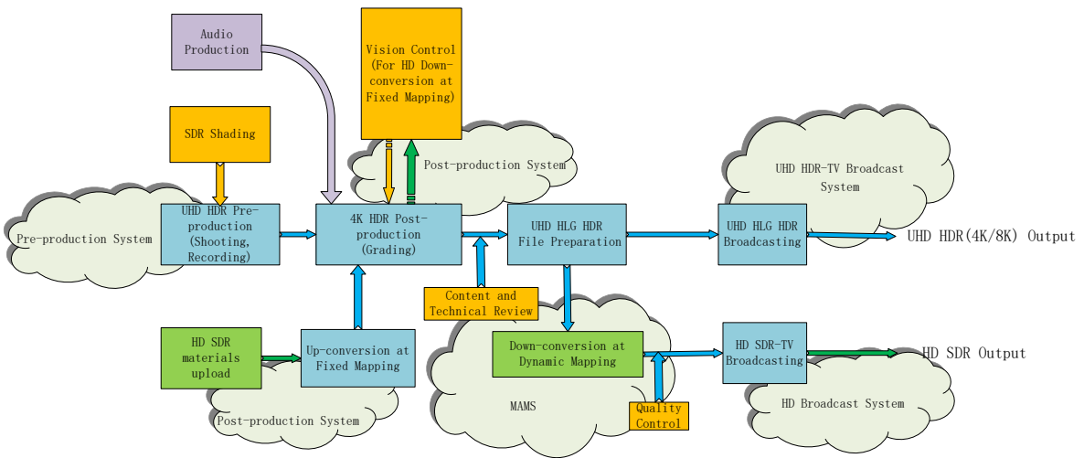
FIGURE A8-2 CMG workflow of recorded programmes (2)
