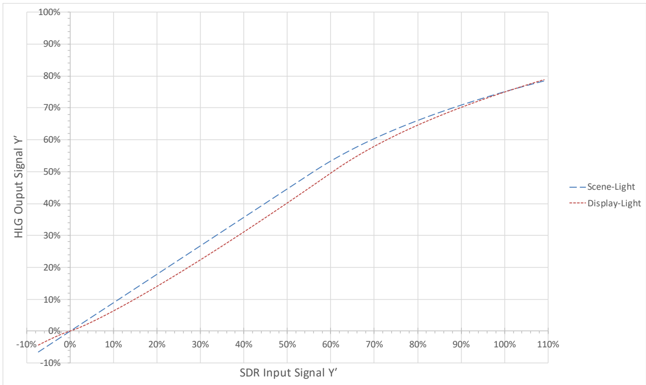
FIGURE 12 Comparison of scene-light and display-light direct-mapping
