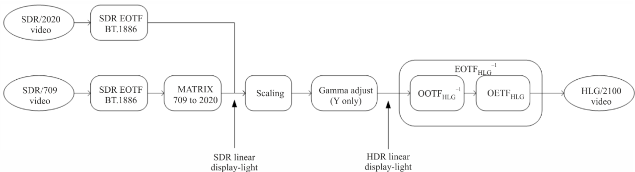
FIGURE 8 Model for “display-referred” mapping with OOTF “gamma” adjustment of SDR into HLG
