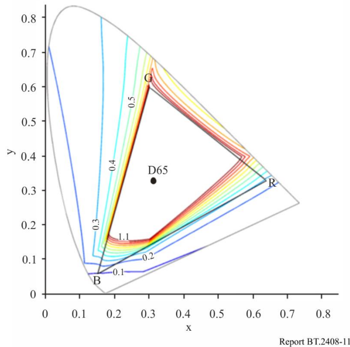
FIGURE 11 Extending the BT.709 camera colour gamut
