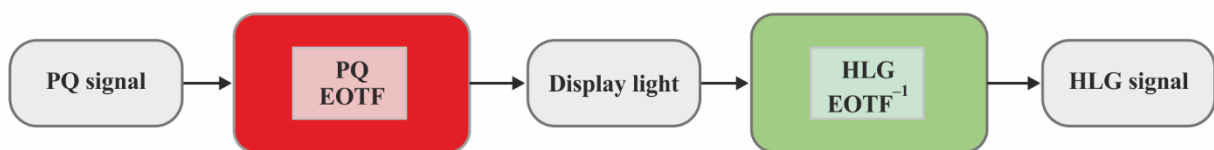
Concept of transcoding from PQ to HLG
