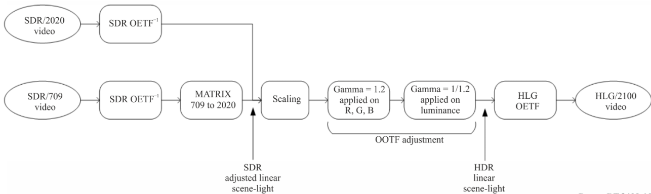
FIGURE 10 SDR to HLG mapping with gamma adjustment (scene-referred)
