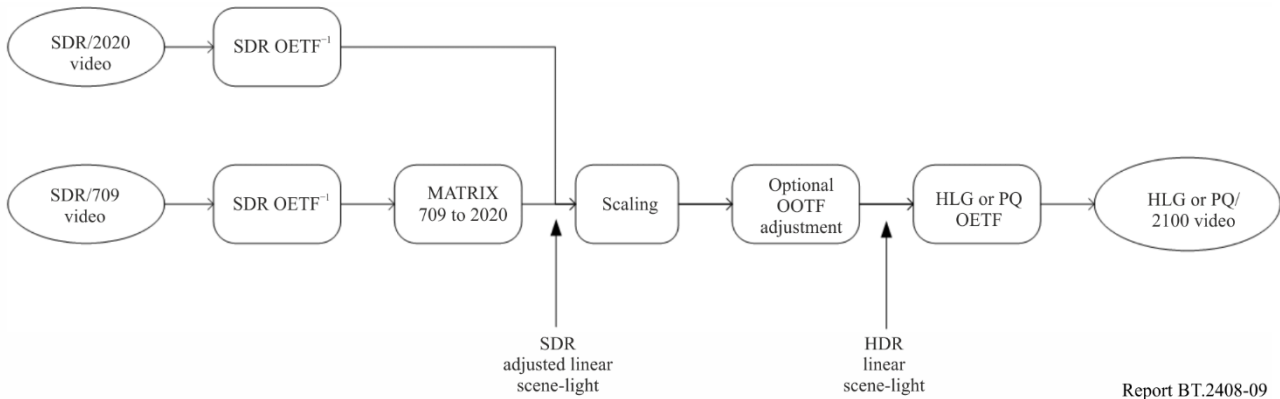
FIGURE 9 SDR to HDR mapping (scene-referred)
