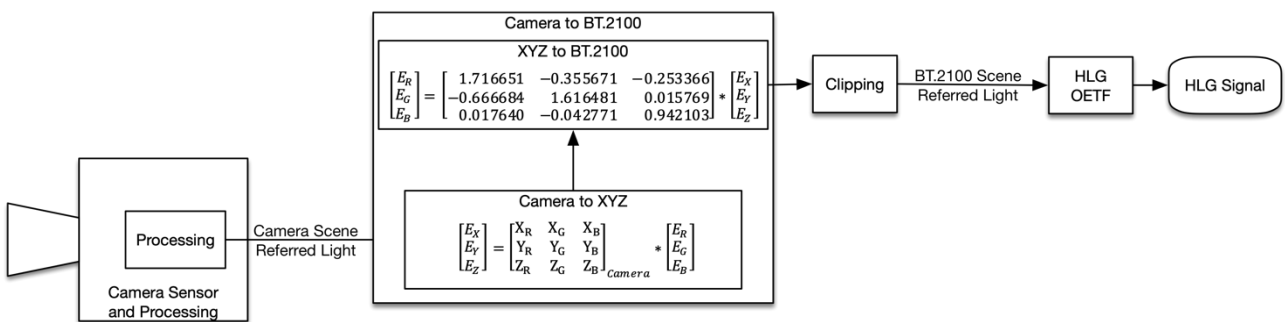
FIGURE 46 Conversion of arbitrary scene referred light signals to a BT.2100 HLG signal using a scene referred workflow
