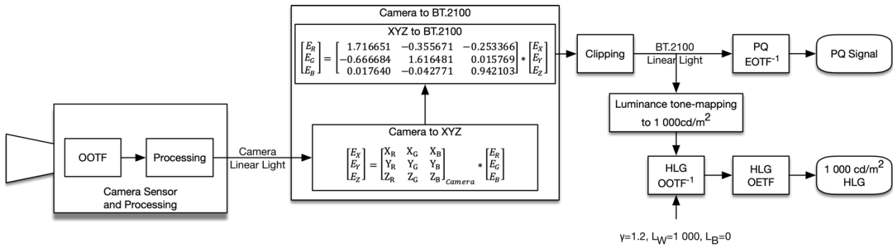
FIGURE 45 Conversion of arbitrary display referred linear light signals to BT.2100 signals using a display referred workflow
