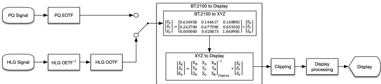
FIGURE 48 Conversion of Recommendation ITU-R BT.2100 signals to an arbitrary display using a display referred workflow
