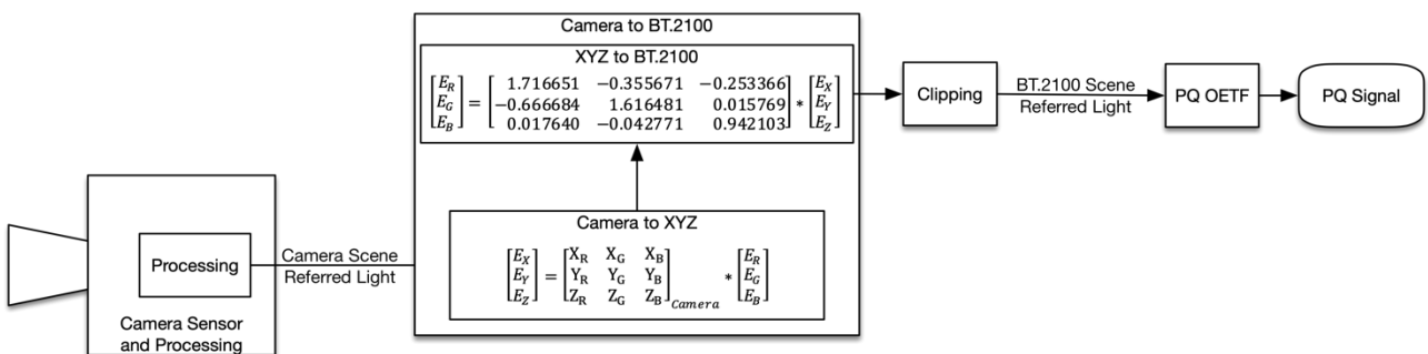
FIGURE 47 Conversion of arbitrary scene referred light signals to a BT.2100 PQ signal using a scene referred workflow
