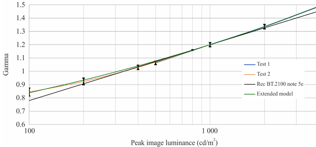
Gamma value to match images for different screen peak brightness
