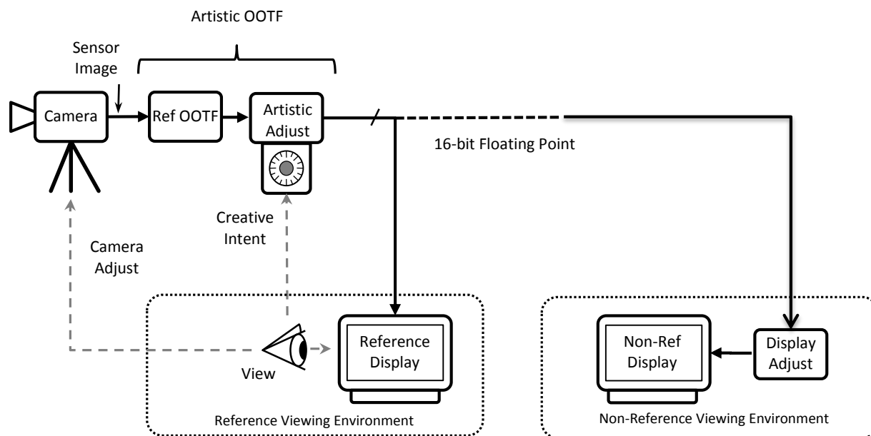
FIGURE 11 HDR floating point system
