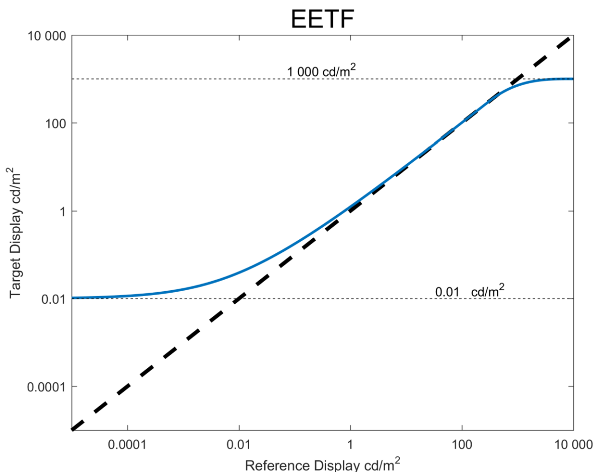
FIGURE 18 Example EETF From 0 - 10 000 \text{cd/m}^2 to 0.01 - 1 000 \text{cd/m}^2
