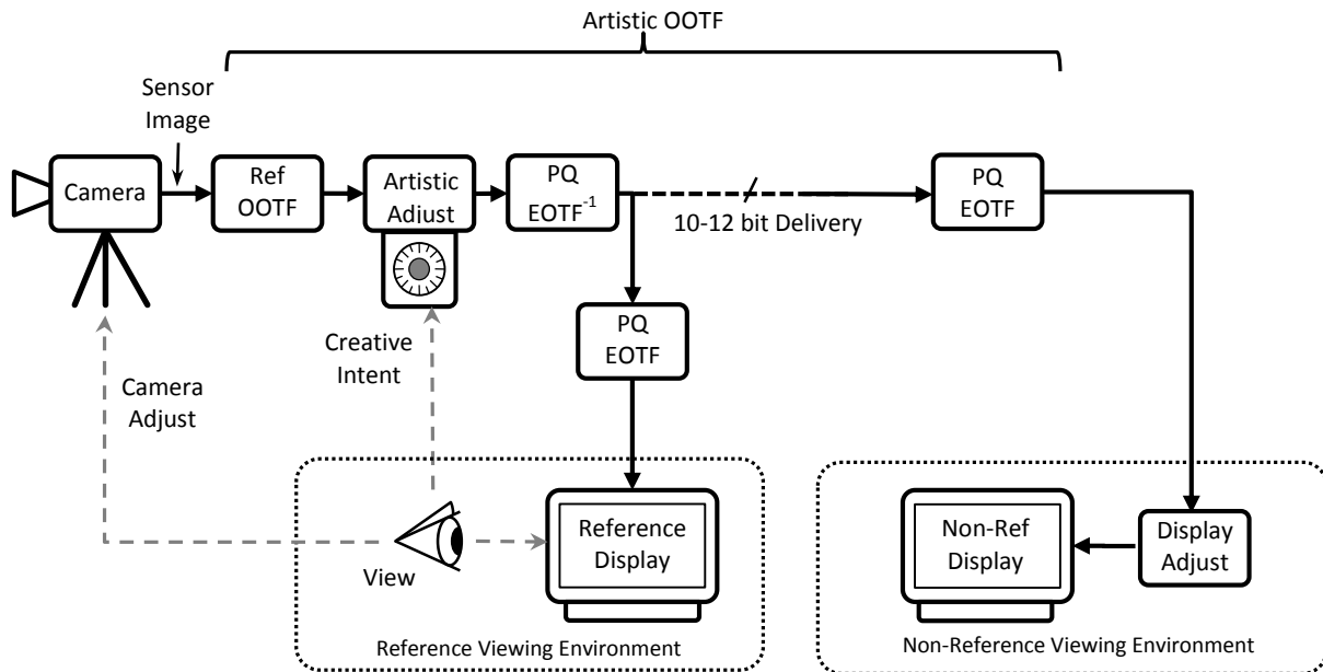
FIGURE 12 PQ HDR-TV system with 10 or 12 bit integer values
