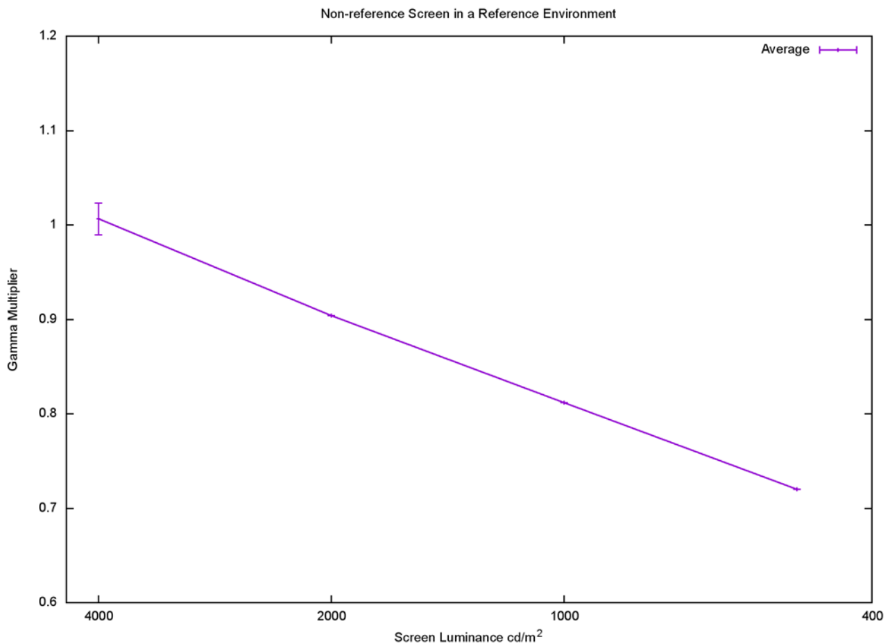
FIGURE 22 Average gamma multiplier for different screen peak brightness
