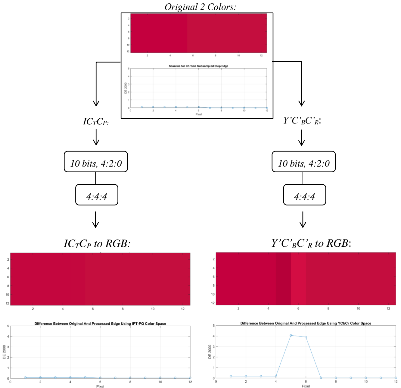
FIGURE 29 Colour sub-sampling distortions based on correlation with luminance
