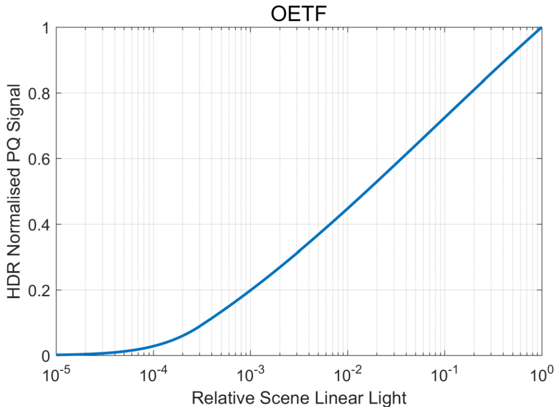
FIGURE 17 HDR OETF
