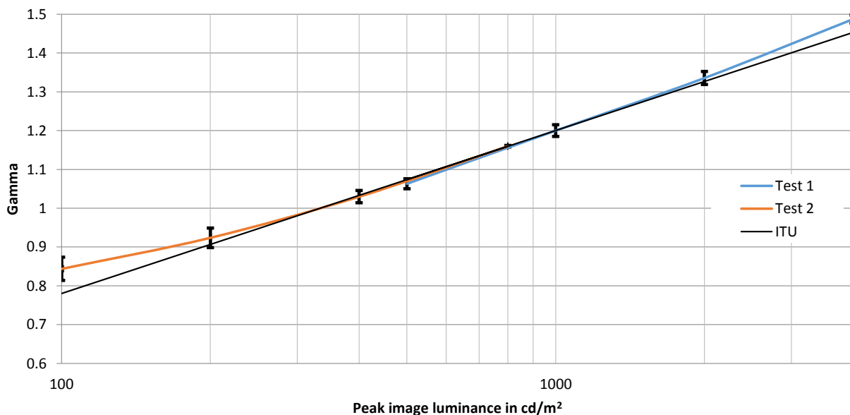
FIGURE 22 Gamma value to match images for different screen peak brightness
