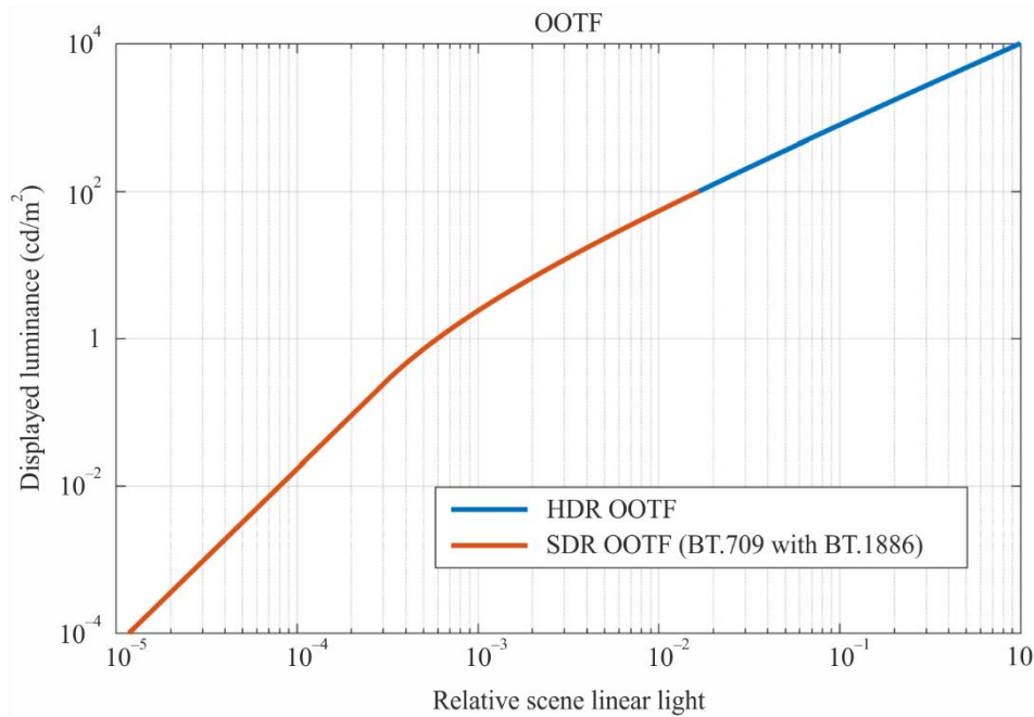
FIGURE 15 PQ and SDR OOTF
