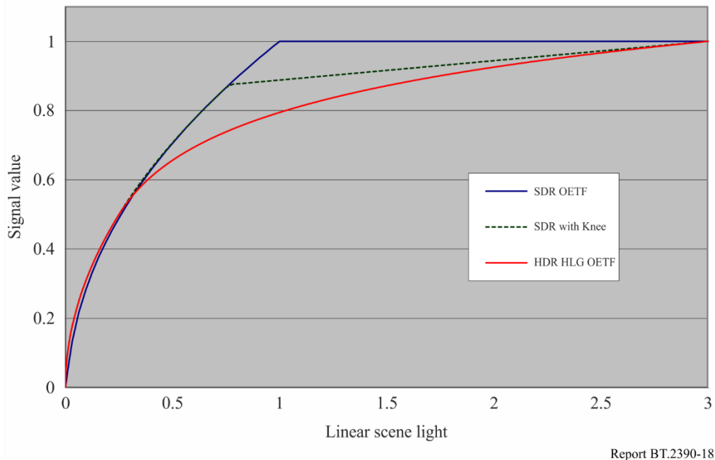
FIGURE 18 Comparison of SDR and HLG HDR OETFs
