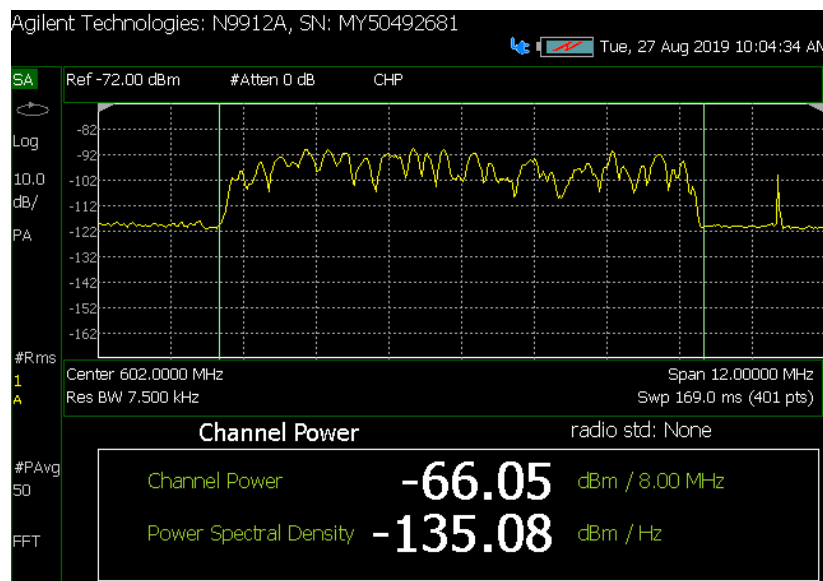
FIGURE P5-4 Typical spectrum of the received signal
