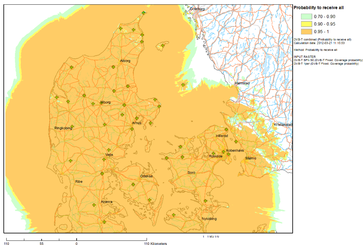
FIGURE P2-67 T2 National SFN 64-QAM R = 3/5 TG 19/128 (532 \mu s)
