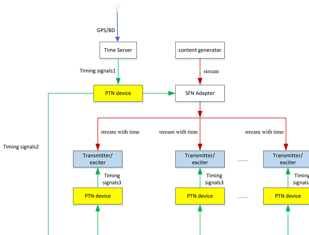
FIGURE P4-20 Proposed SFN system structure
