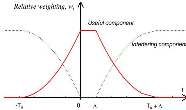
FIGURE P2-7 T-DAB model - Splitting of the signal power into useful and interfering components
