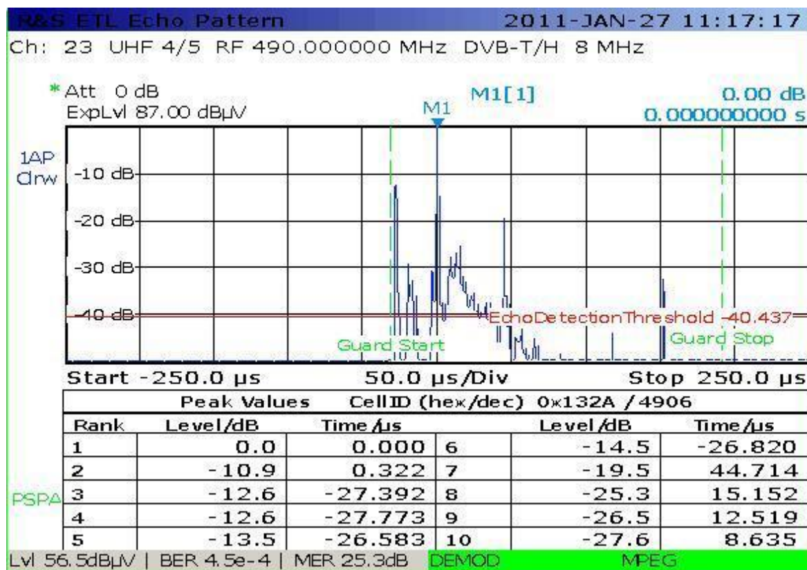
FIGURE P2-34 Stazzona Channel analysis
