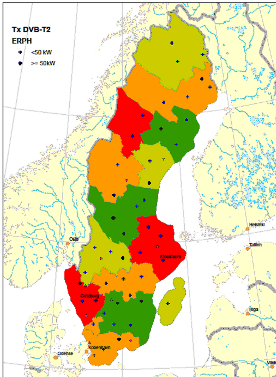
FIGURE P2-69 Frequency Network in Sweden
