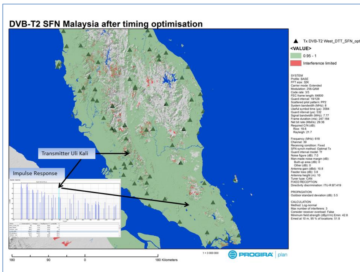
FIGURE P2-82 Resulting DVB-T2 coverage after optimization of SFN self-interference
