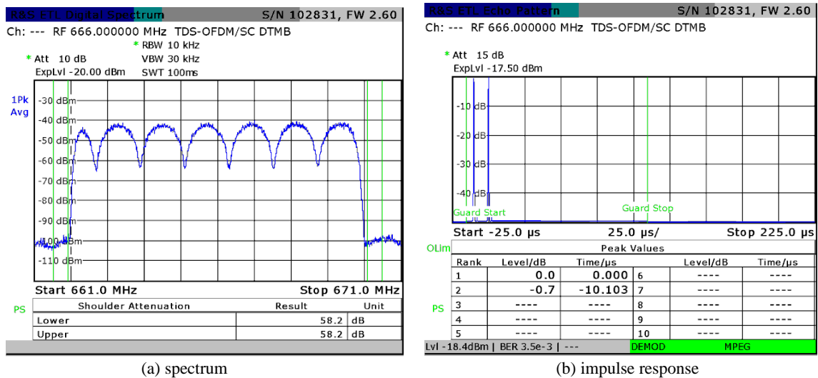
FIGURE P4-16 Signal characteristics of the combined signal
