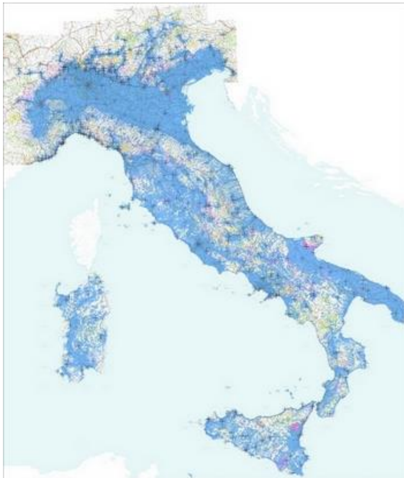
FIGURE P2-35 DFREE at the end of the Analogue Switch Off (1-SFN) – More than 400 sites – Useful coverage > 90% population
