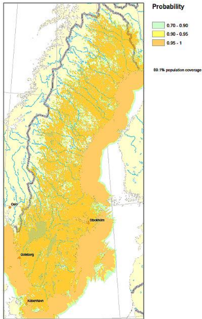
FIGURE P2-70 National SFN frequency plan, 256-QAM R=3/4 TG=19/128 (532 \mu s)
