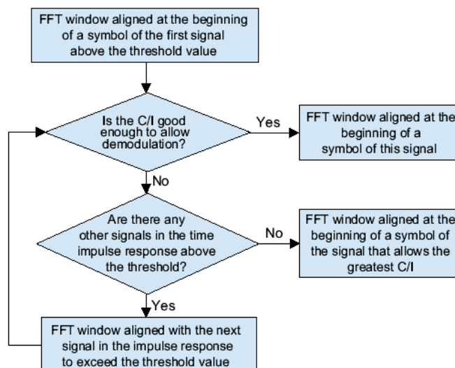
Flowchart describing the Quasi-Optimal Strategy
