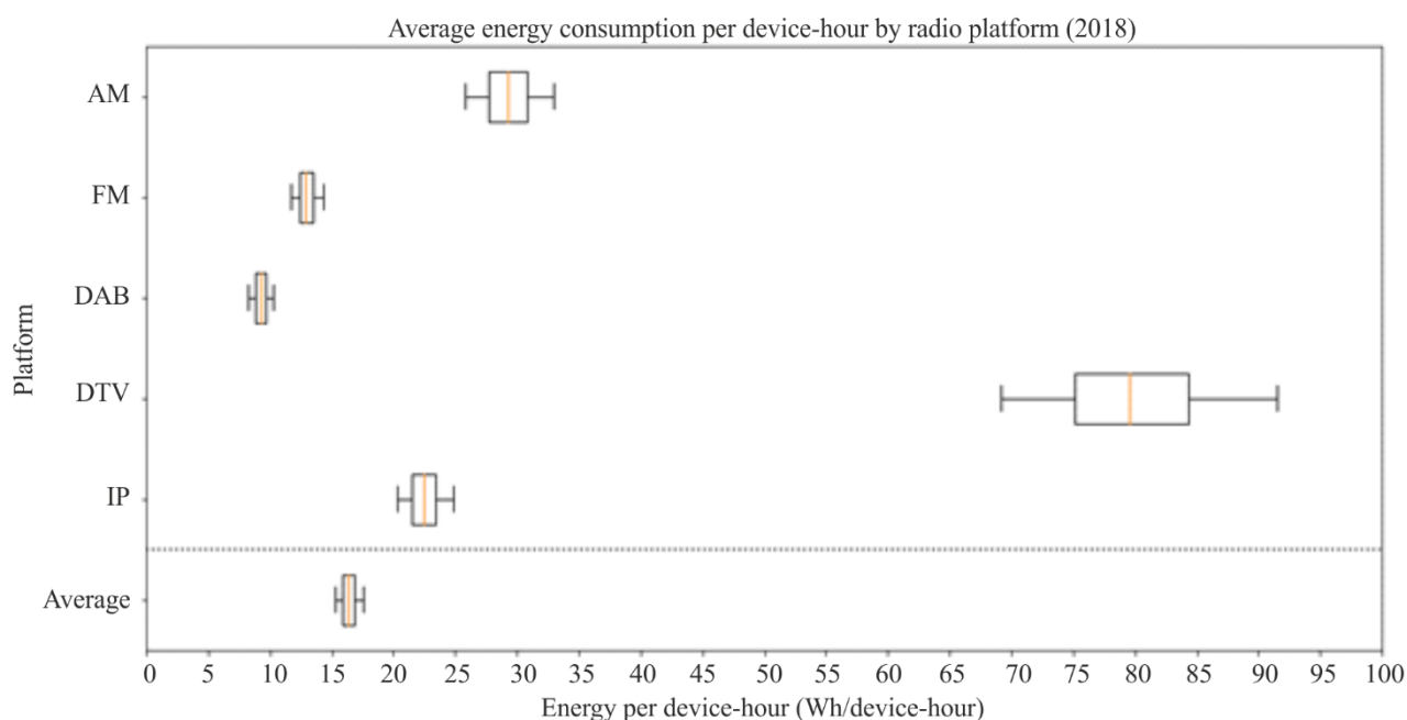
FIGURE 35 Estimated energy per device-hour to prepare, distribute and consume BBC radio in 2018 per platform
