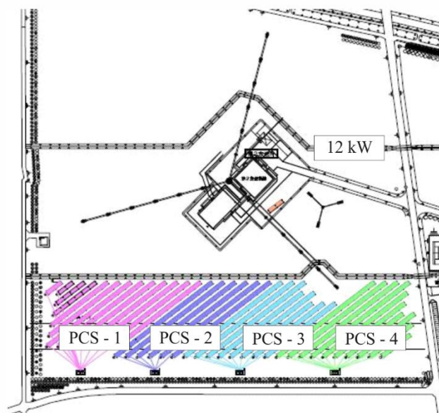
FIGURE 6 Positioning of solar panels
