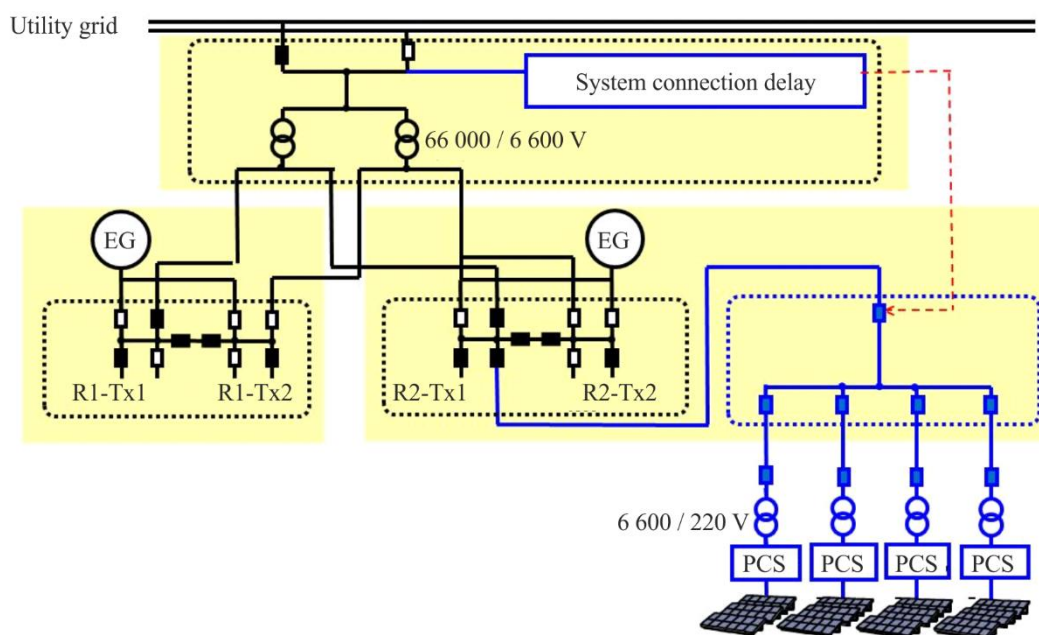
FIGURE 10 Connecting to the grid
