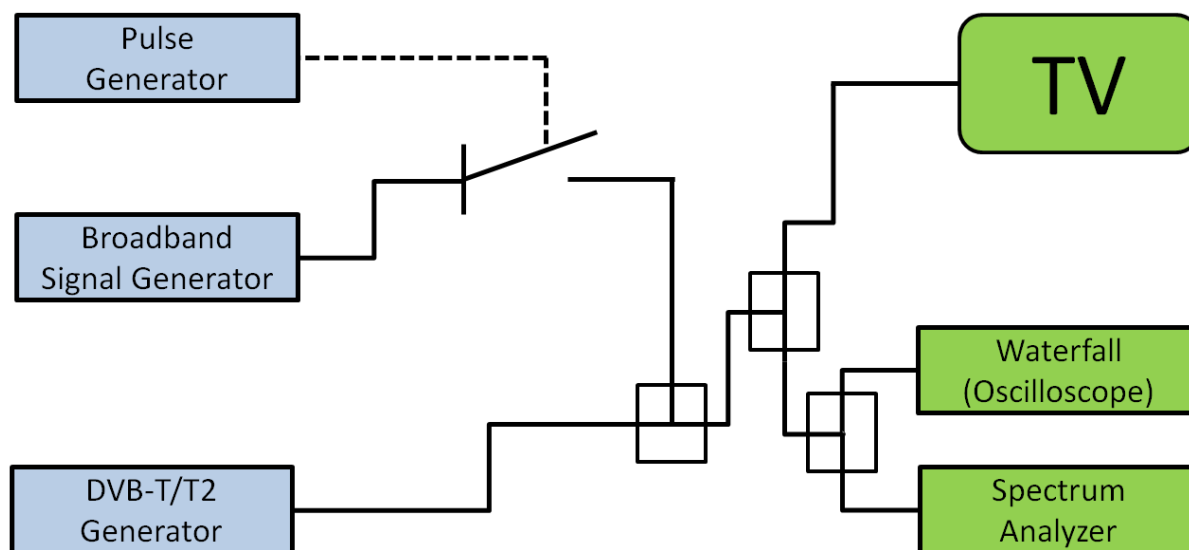
FIGURE A1-1 Test setup
