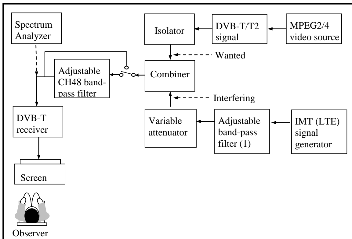
FIGURE A2-1 Measurements set-up
