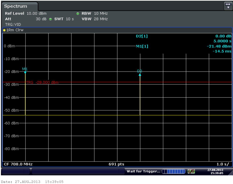
FIGURE A1-9 Spectrum analyser trace showing 5 second pulse repetition
