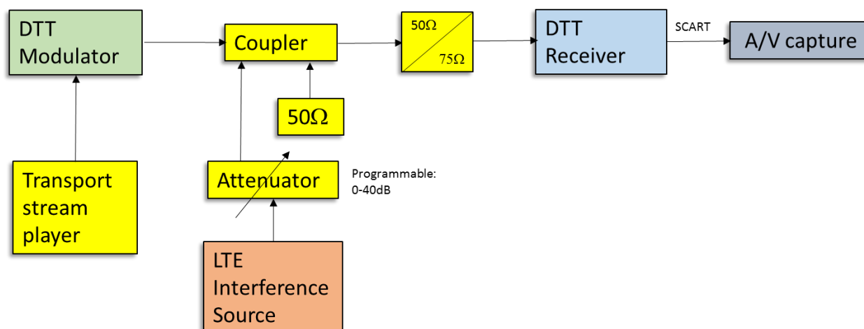
Laboratory test configuration
