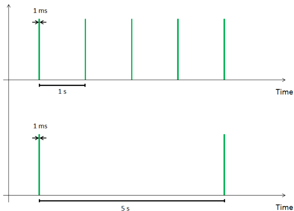
Pulse pattern for Cases #1 and #2
