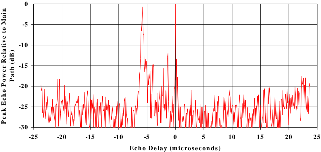
FIGURE A3-27 Peak echo power observed in the RF capture at Site 8 using a single bowtie-type antenna in a fourth-floor urban apartment
