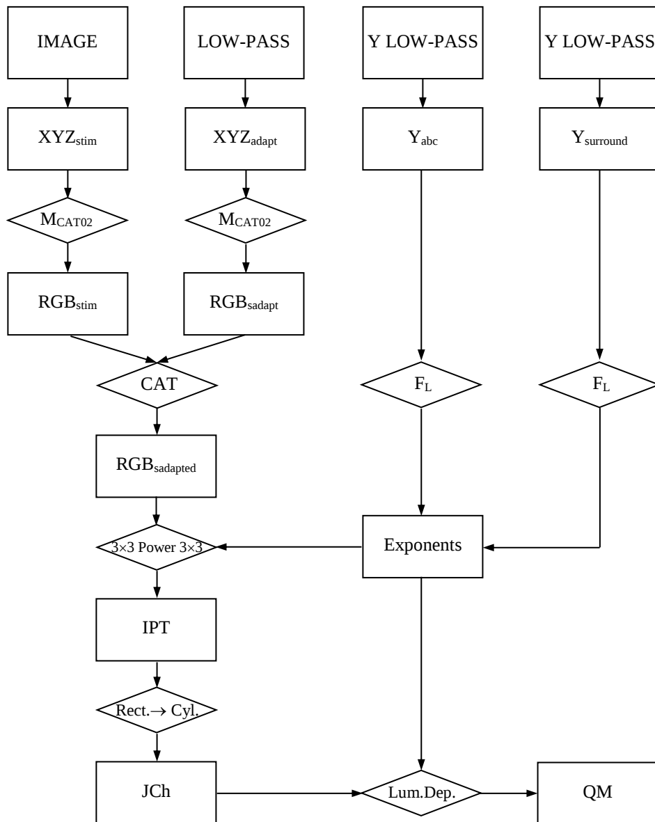
Flowchart of iCAM image appearance model
