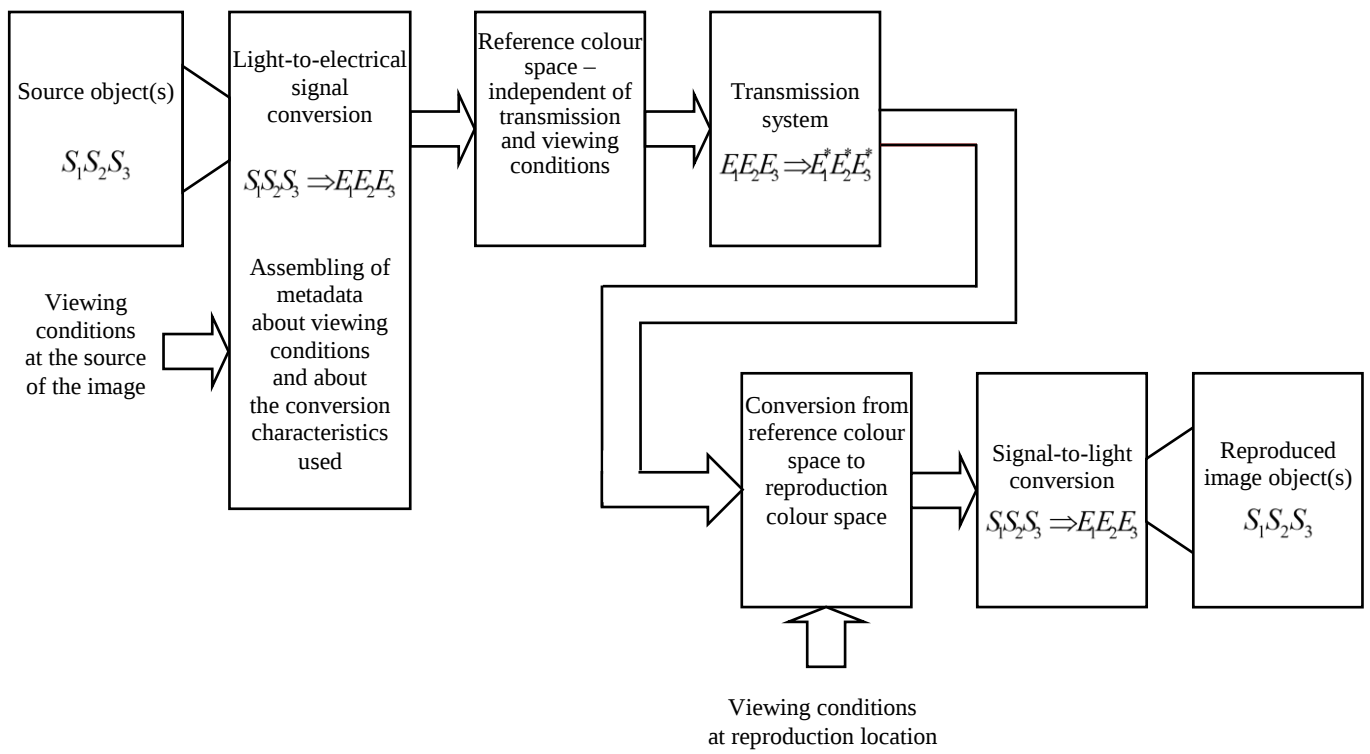
Block diagram of a potential adaptive system
