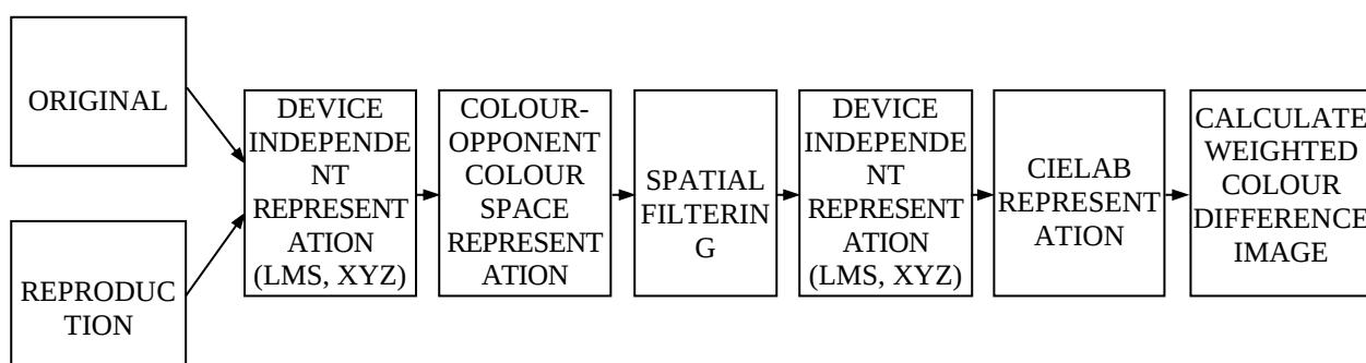
FIGURE 5.1 Flowchart of S-CIELAB
