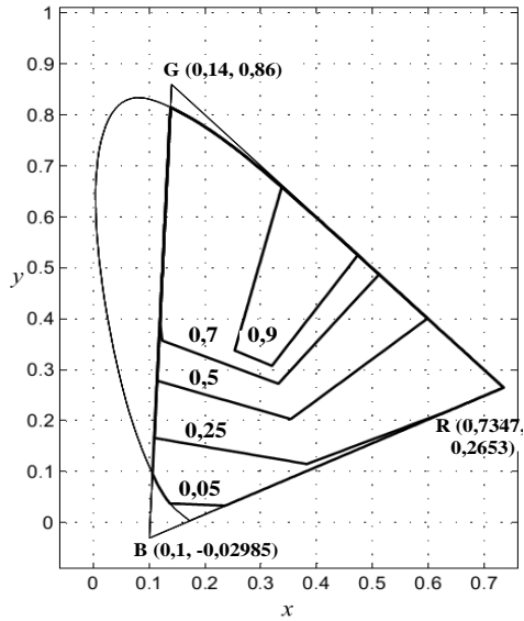
Colour gamut boundaries of DC system on the CIE-31 chromaticity diagram plane
