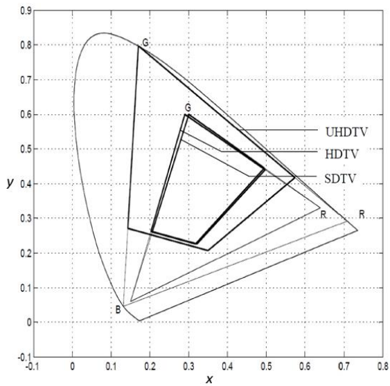
Colour gamuts of SDTV, HDTV and UHDTV systems for in XYZ space
