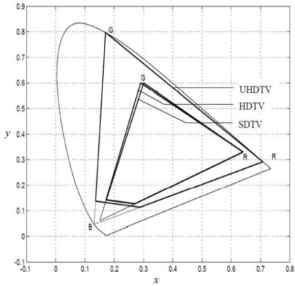
Colour gamuts of SDTV, HDTV and UHDTV systems for in XYZ space
