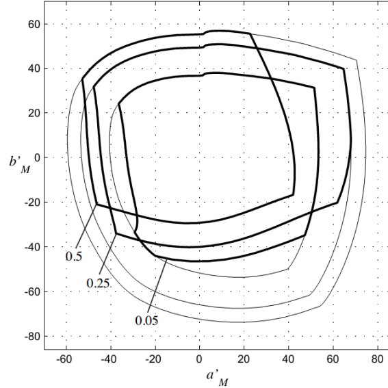
Colour gamut boundaries of DC system for L_A = 50 \text{ cd/m}^2 on the plane of a'_M, b'_M
