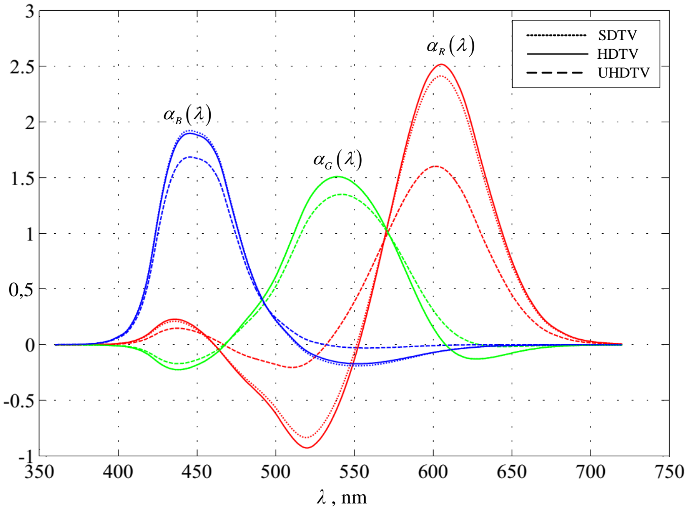
FIGURE 2.1 Comparison of the spectral sensitivity characteristics of primary signal channels of SDTV, HDTV, UHDTV in terms of CIE 1931 colorimetry
