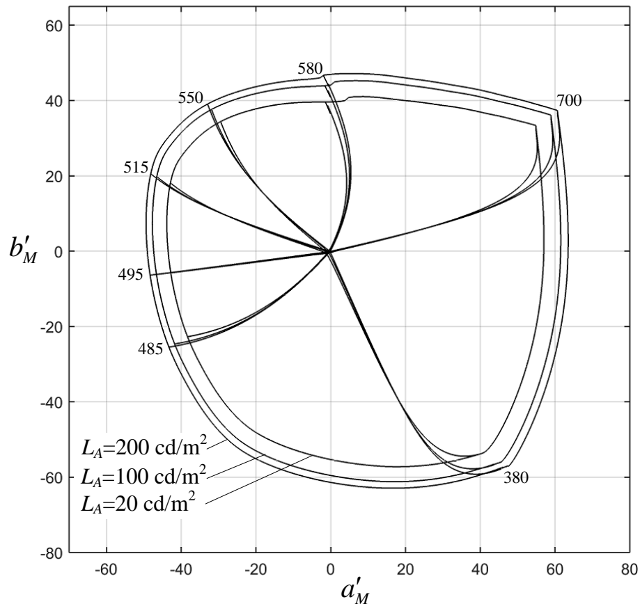
FIGURE A.1 Chromaticity diagram CAM02-UCS ( a'_M, b'_M ), Y_w=100, Y=10
