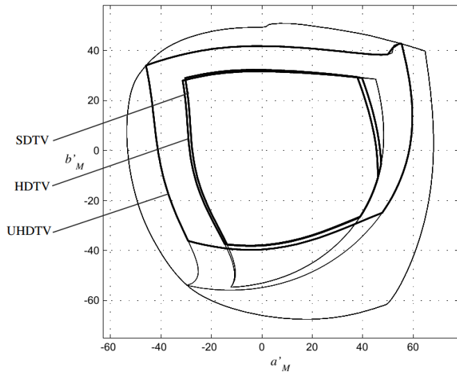
Colour gamuts of SDTV, HDTV and UHDTV systems for L_A = 50 \text{ cd/m}^2 in CAM02-UCS space
