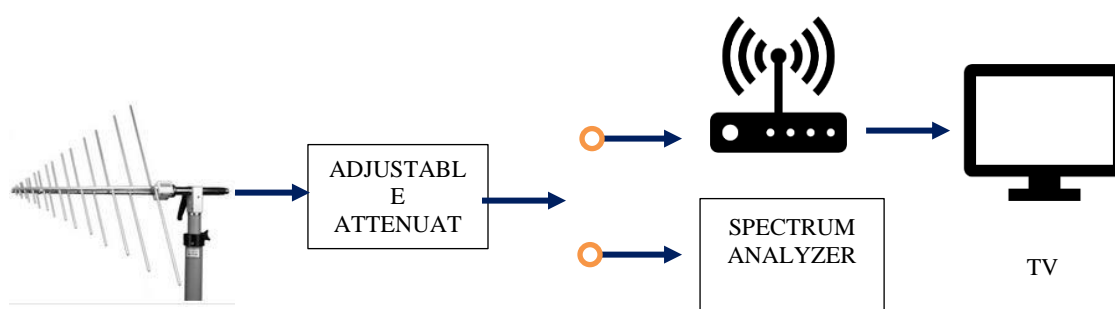
FIGURE 51 Test setup
