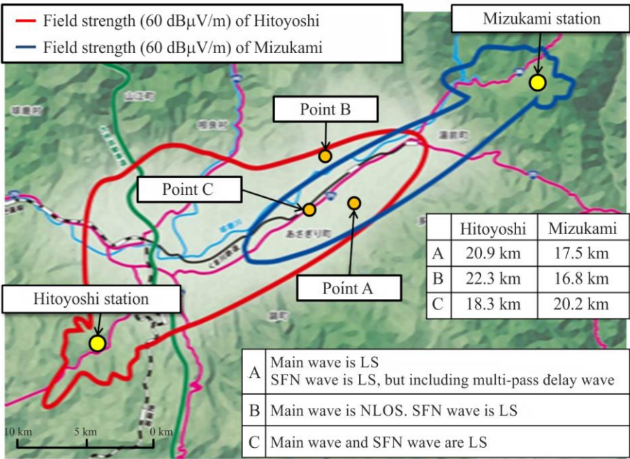
FIGURE 16 Measuring points
