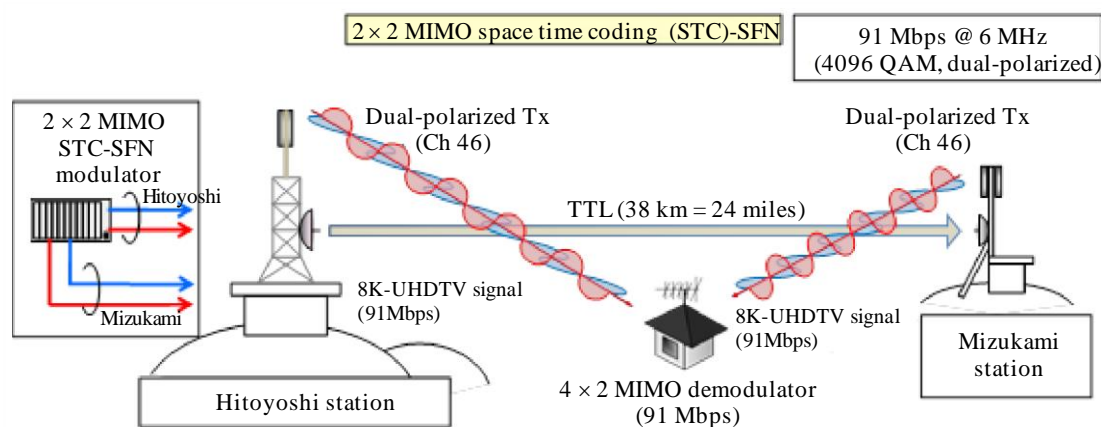
Outline of 2x2 MIMO STC-SFN transmission system
