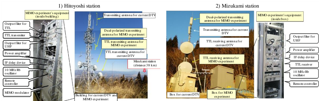
FIGURE A1.12 Equipment of MIMO experimental stations
