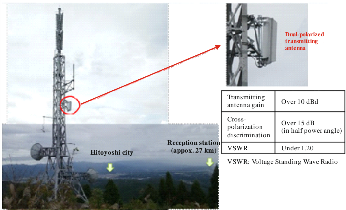
FIGURE A1.2 Transmitting station and equipment
