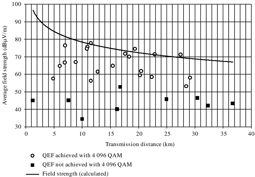
FIGURE A1.8 Average field strength vs. transmission distance
