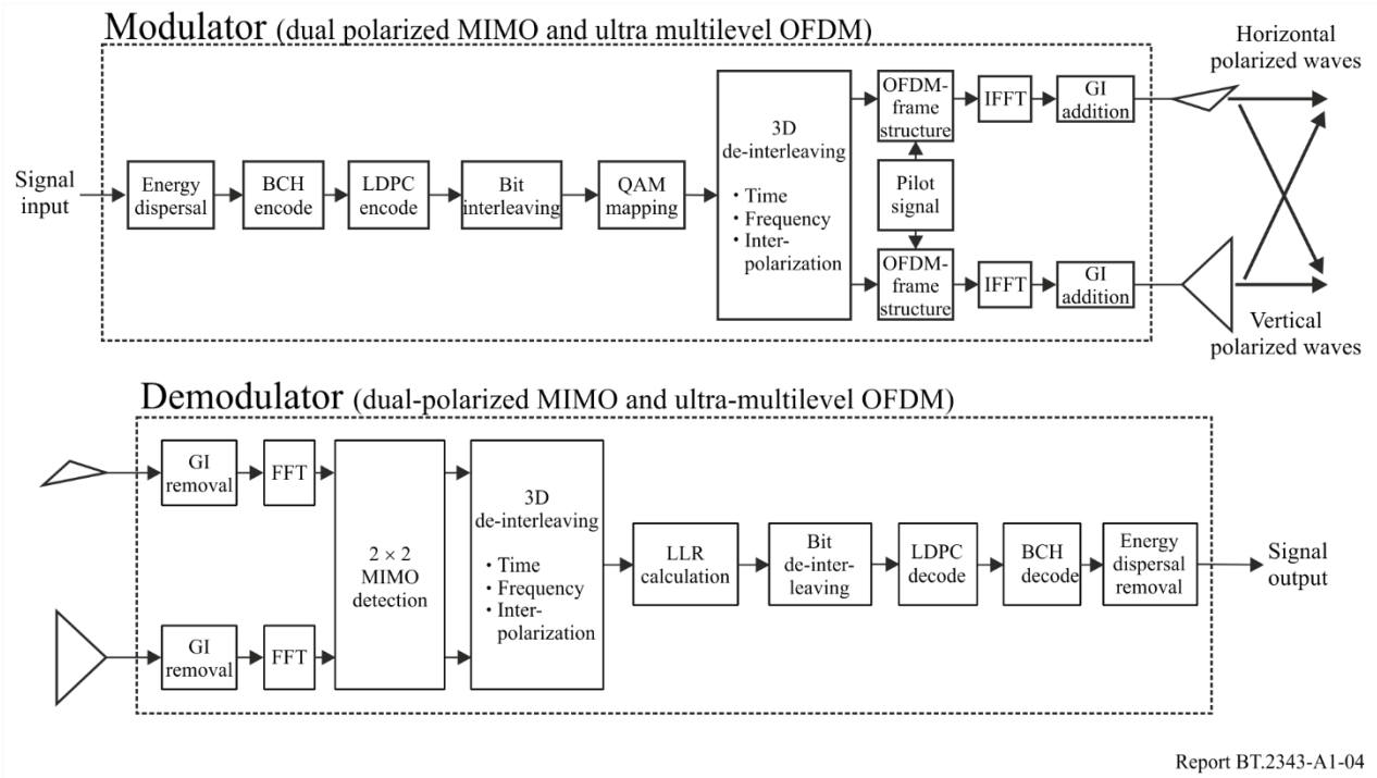
FIGURE A1.4 Block diagram of 8K experiments
