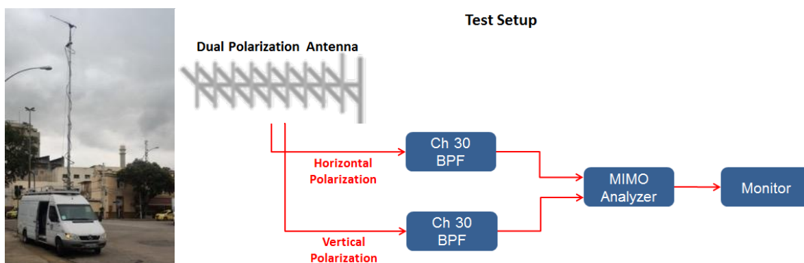
Test setup
