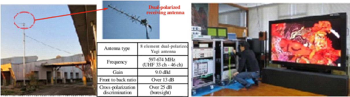
FIGURE A1.3 Receiving station and equipment
