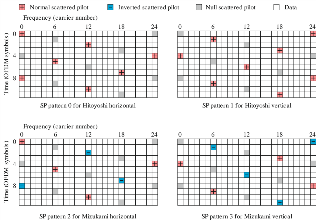
Scattered pilot patterns
