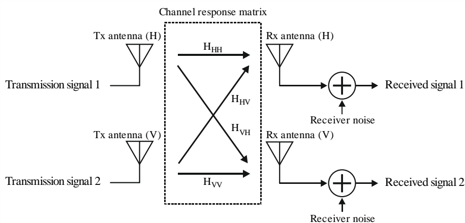
FIGURE A1.6 MIMO transmission model
