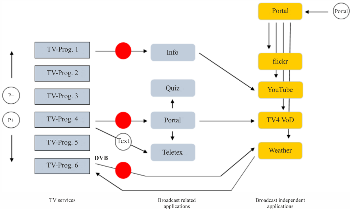
FIGURE 1.5 HbbTV applications can be tied to broadcasting services or can be independent of broadcasting services
