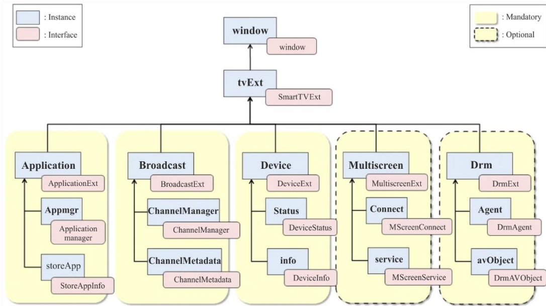
FIGURE 1.49 Smart TV Extended API structure
