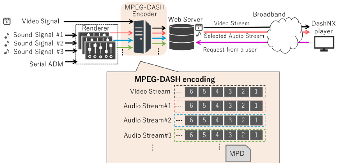
System example for distributing object-based sound services on Hybridcast
