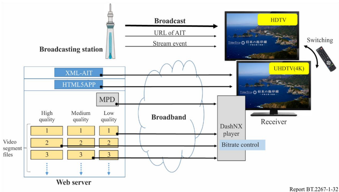
FIGURE 1.35 System configuration of multi-resolution video service using Hybridcast
