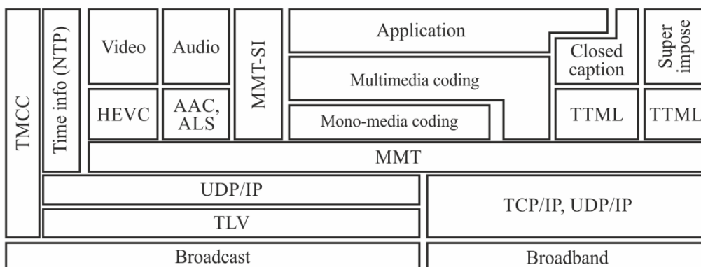
FIGURE 1.13 Protocol stack defined in ARIB STD-B62 for MMT
