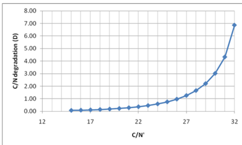
FIGURE 2 Factor D, C/N degradation (dB) for a back-stop noise level of -33 dBc
