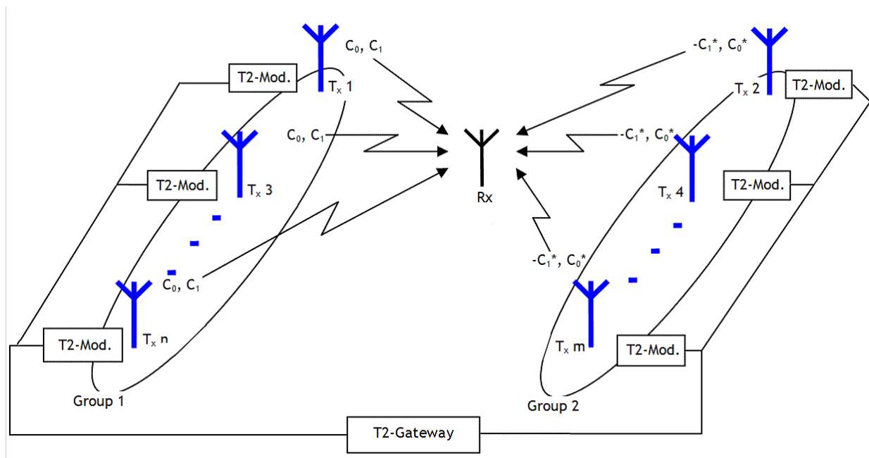
FIGURE 25 A general DVB-T2 MISO network
