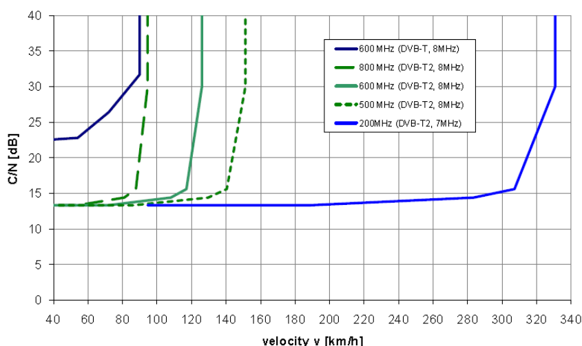
FIGURE 10 Required C/N for DVB-T and DVB-T2 as a function of the velocity of the mobile receiver, 8k FFT (from [AFM2010])
