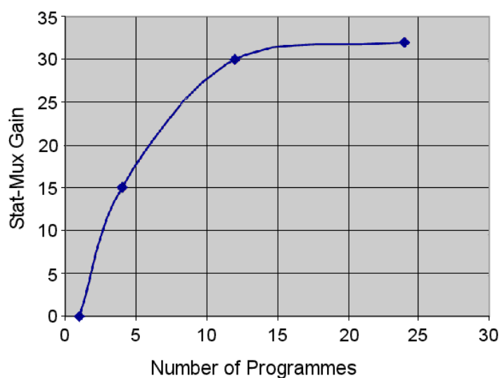
FIGURE 31 Statistical multiplex gain with MPEG-4 AVC
