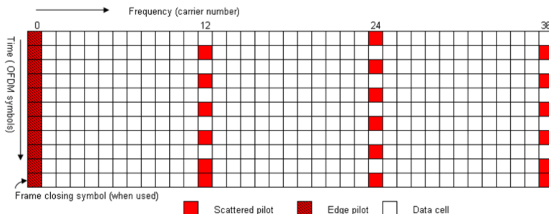
FIGURE A6.3 Scattered pilot pattern PP4 (SISO)
