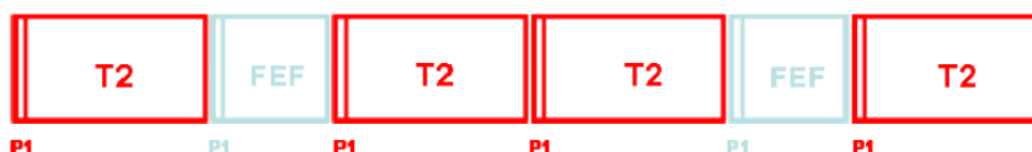
FIGURE 36 Co-existence of T2 frames and FEFs (from [TR 102 831])
