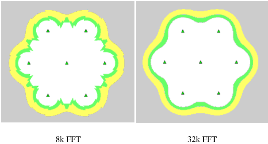
FIGURE 23 Comparison of the coverage areas for the 8k and the 32k FFT mode
