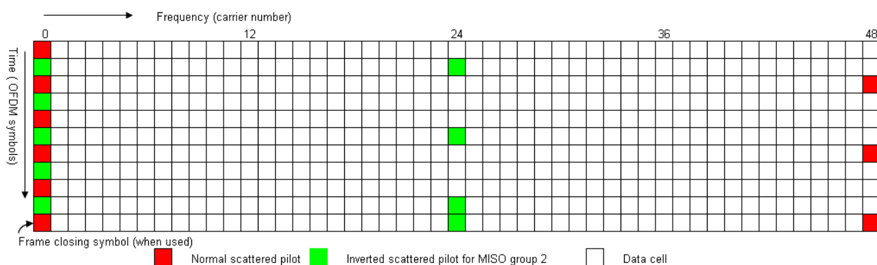
FIGURE 9 Pilot pattern 7 – MISO (from [EN 302 755 V1.3.1])
