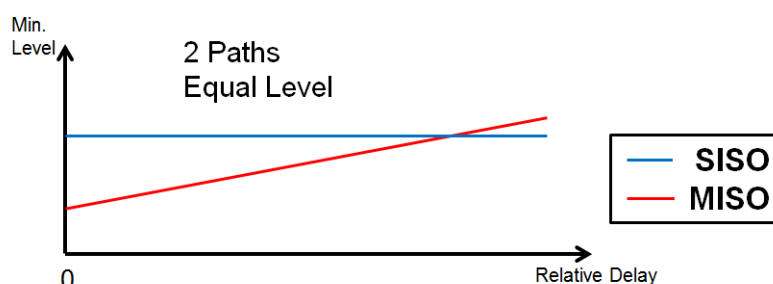
FIGURE 27 MISO gain as a function of relative delay (MISO gain = difference of min. required levels)
