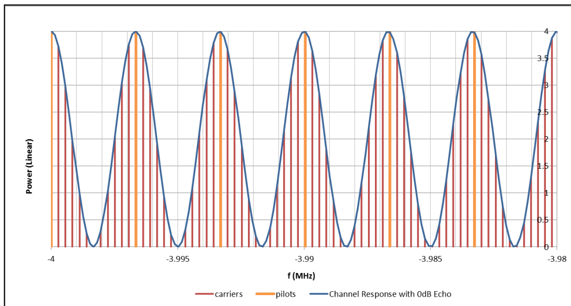
FIGURE A6.5 DTT passband in a perfect channel with 0 dB echo at 300 \mu s delay – linear amplitude
