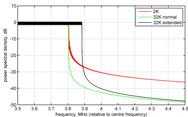
FIGURE 12 Detail of theoretical DVB-T2 spectrum for guard-interval fraction 1/8 (for 8 MHz channels) (from [EN 302 755])
