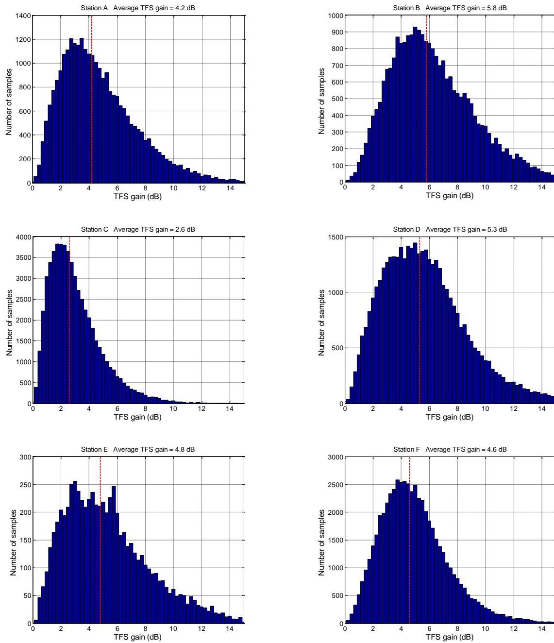
FIGURE 32 Measured distribution of TFS gain
