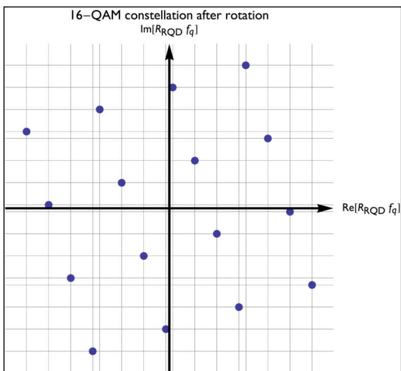
FIGURE 4 Rotated constellation diagram for 16-QAM modulation (from [TS 102 831])
