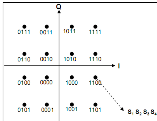
FIGURE 3 Constellation diagram for 16-QAM modulation (Figure taken from [ND2008])
