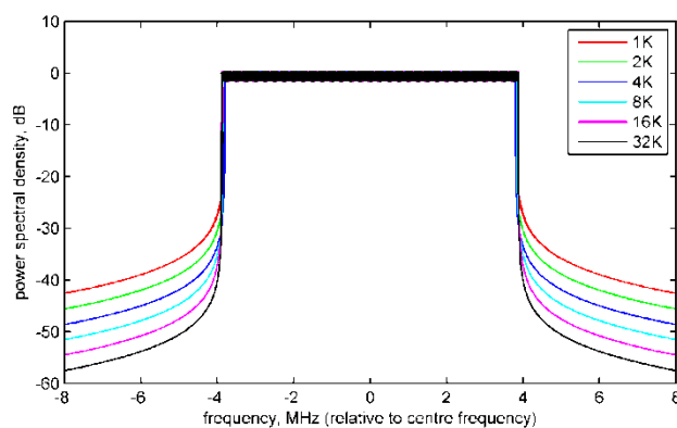
FIGURE 11 Theoretical DVB-T2 signal spectrum for guard interval fraction 1/8 (for 8 MHz channels and with extended carrier mode for 8k, 16k and 32k) (from [EN 302 755])
