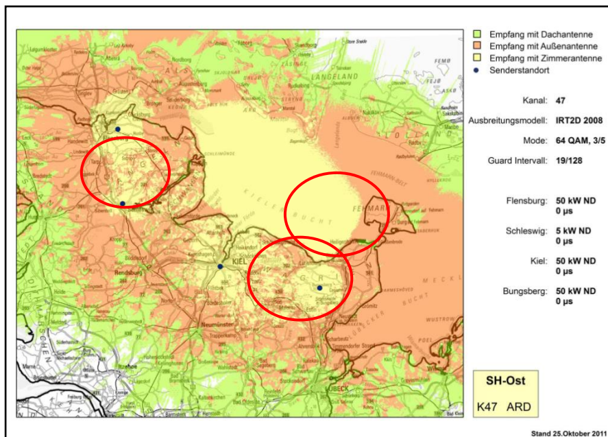
FIGURE 4.6 Portable reception, SFN, medium area, UHF, DVB-T2 in the northern part of Germany
